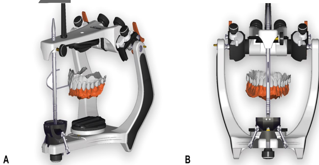
Figure 4 Mounted virtual articulator. A, Side view. B, Front view.
