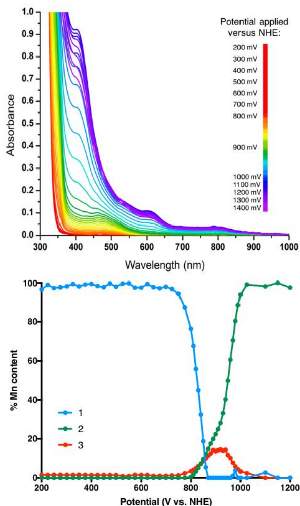
Figure 6. a) Series of final UV-Vis spectra obtained at each potential indicated after 15 min of electrolysis to a 2.5 mM solution of 1 in pH 4.47 0.1 M acetate buffer. Conditions: Pt working electrode, Pt wire counter electrode, Ag/AgCl reference electrode. b) Deconvolution of spectra shown in a), modeled as a linear combination of basis UV-vis spectra obtained from 1 , 2 , and 3 recorded at 2.5 mM, 1.25 mM, and 2.5 mM, respectively.
