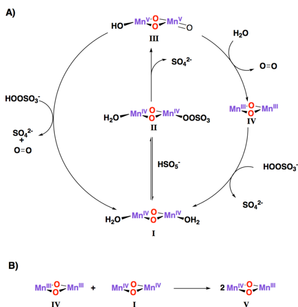
Figure 4. A) Proposed catalytic mechanism based on kinetic and EPR experiments. The left side of the figure represents the proposed mechanism if evolved oxygen arises fully from \text{HSO}_5^- incorporation, whereas the right side shows implicated states if water is incorporated. B) Comproportionation reaction scheme proposed to give rise to V.
