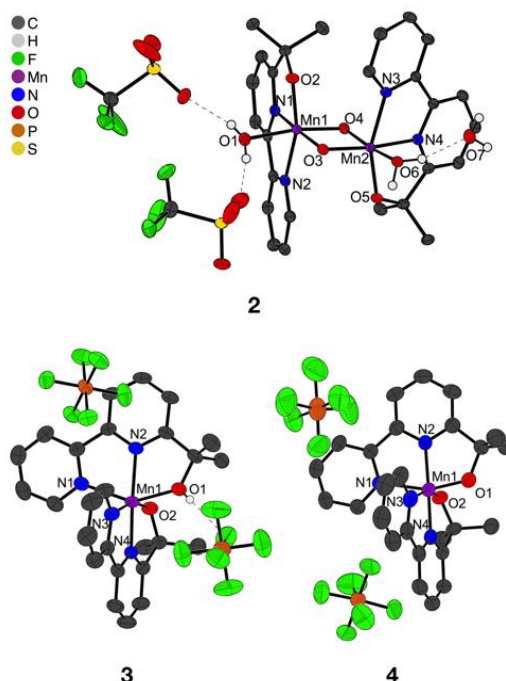
Figure 2. X-ray crystal structures of 2 , 3 , and 4 . For all three structures, thermal ellipsoids are displayed at the 50% probability level and hydrogens except for those bound to heteroatoms are omitted for clarity. For 2 , two triflate counterions and one DCM solvent molecule are omitted for clarity. See Figures S18-S20 for complete scheme and omitted moieties.
