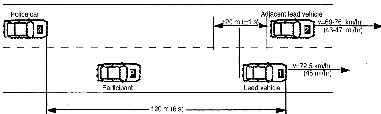
Figure 3. Typical traffic layout.
