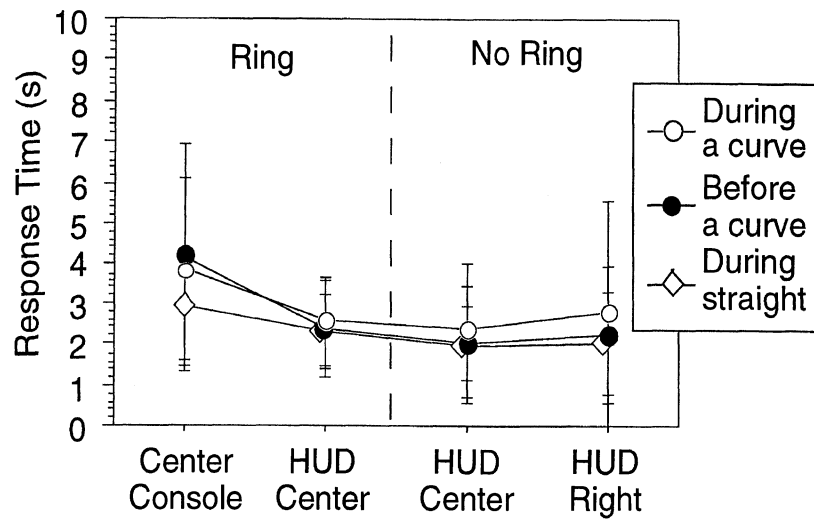
Figure 16. The effect of call timing on response time.
