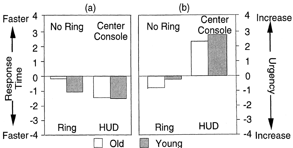
Figure 18. Perceived response time and urgency ratings.
