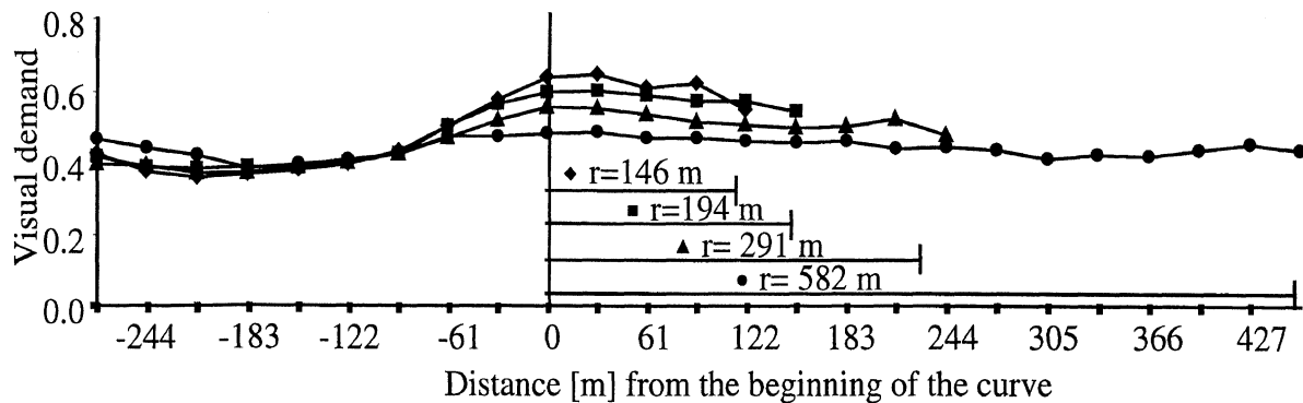
Figure 2. Visual demand as a function of curve radius and position.
