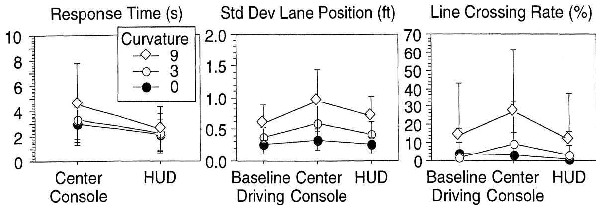
Figure 15. The effects of road curvature on task and driving performance.
