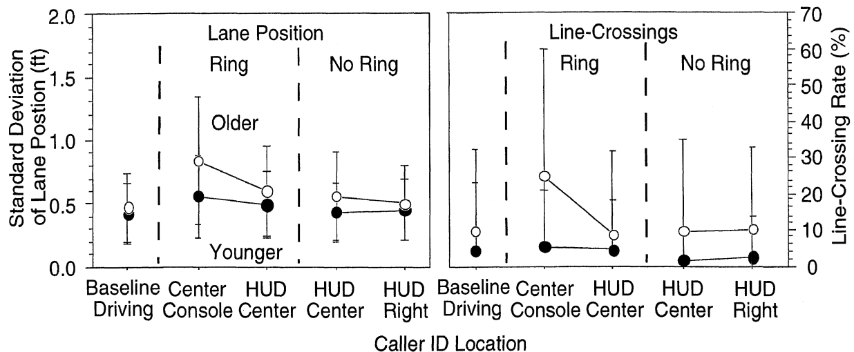
Figure 11. Lane keeping while answering the phone.
