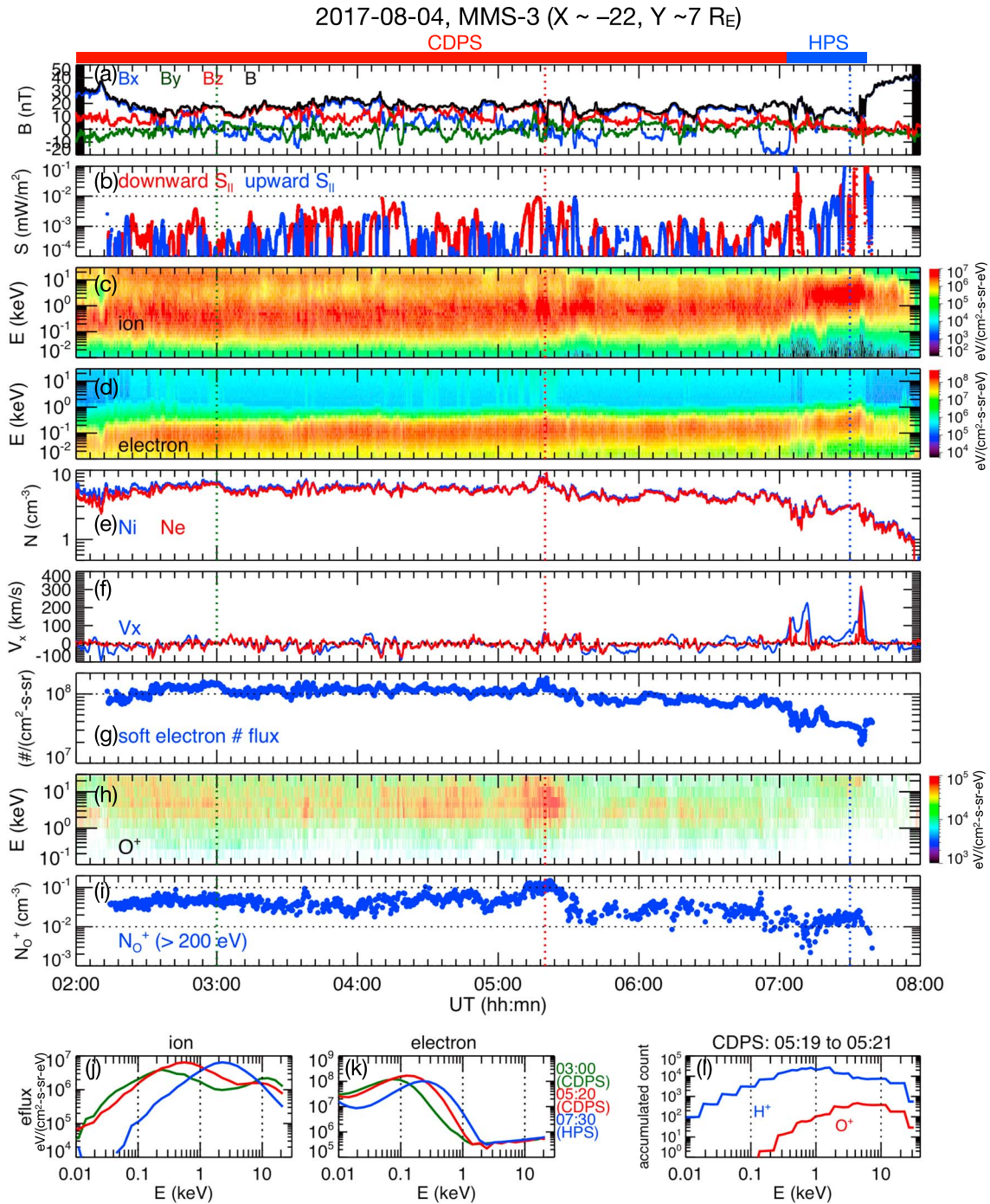
Figure 9. Event 3 on 4 August 2017. The MMS-3 observations of (a) magnetic fields, (b) the downward (red) and upward (blue) Poynting flux within the CDPS, (c) ion and (d) electron energy fluxes, (e) ion and electron number densities, (f) ion bulk flows in the X_{GSM} direction, (g) electron number fluxes integrated from 30 to 100 eV, (h) O^+ energy fluxes, and (i) the O^+ densities integrated over energies above 1 keV. Energy spectrum of (j) ion and (k) electron energy fluxes at three different times indicated by the vertical dotted lines in Figures 10a to 10i. (l) The accumulated H^+ (blue curves) and O^+ (red curves) counts within the 2-min interval indicated on the top of the plot. CDPS = cold-dense plasma sheet; HPS = hot plasma sheet; MMS = Magnetospheric Multiscale.
