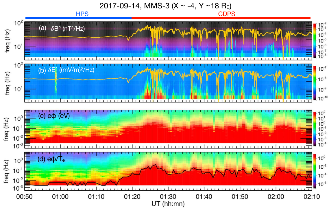
Figure 5. Event 1 on 14 September 2017. The MMS-3 observations of power spectrum of (a) \delta B and (b) \delta E . The yellow curves indicate the electron gyro frequencies. Computed power spectrum of (c) e\Phi and (d) e\Phi/T_e . The black line in (d) indicates e\Phi/T_e = 1 . CDPS = cold-dense plasma sheet; HPS = hot plasma sheet; MMS = Magnetospheric Multiscale.
