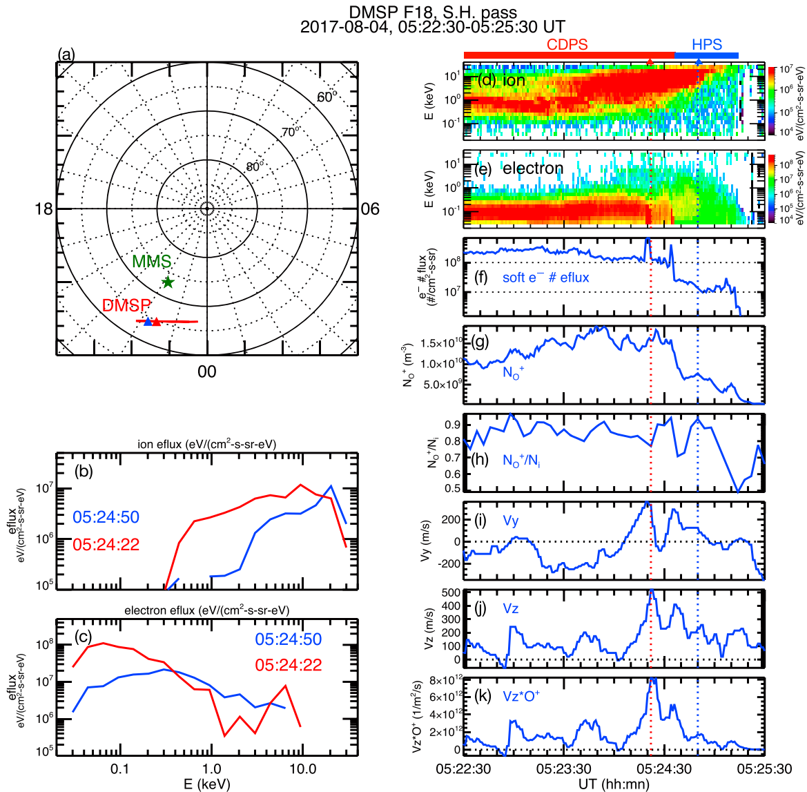
Figure 10. DMSP F-18 observations from 05:22:30 to 05:25:30 UT on 4 August 2017 for event 3. (a) The red line indicates the DMSP trajectory (the red and blue triangles indicate the location corresponding to the two different times indicated by the vertical dotted lines in Figures 10d–10k.). The green star indicates the footprint of the MMS spacecraft. Energy spectrum of (b) ion and (c) electron energy fluxes at the two different times. Temporal profiles of (d) ion and (e) electron energy fluxes, (f) electron number fluxes integrated over 30 to 100 eV, (g) the O^+ densities, (h) O^+ /ion density ratios, (i) sunward flows, (j) upward flows, and (k) the O^+ upward fluxes. CDPS = cold-dense plasma sheet; DMSP = Defense Meteorological Satellite Program; HPS = hot plasma sheet; MMS = Magnetospheric Multiscale.
