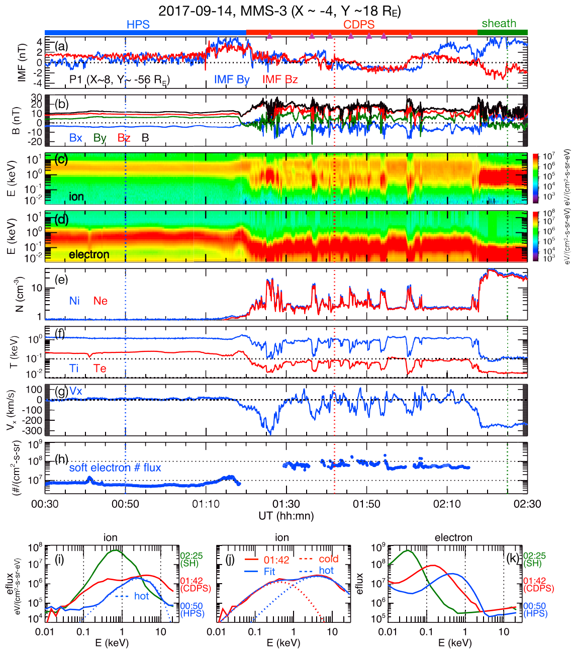
Figure 1. Event 1 on 14 September 2017. (a) IMF from ARTEMIS. The MMS-3 observations of (b) magnetic fields, (c) ion energy fluxes, (d) electron energy fluxes, (e) ion and electron number densities, (f) ion and electron temperatures, (g) ion bulk flow in the X_{GSM} direction, and (h) electron number fluxes integrated from 30 to 100 eV. Energy spectrum of (i) ion and (k) electron energy fluxes at three different times indicated by the vertical dotted lines in Figures 1a to 1h. The blue dotted line in (i) is the fit to the HPS. (j) Observed and fit ion energy fluxes at 01:42 UT. CDPS = cold-dense plasma sheet; HPS = hot plasma sheet.
