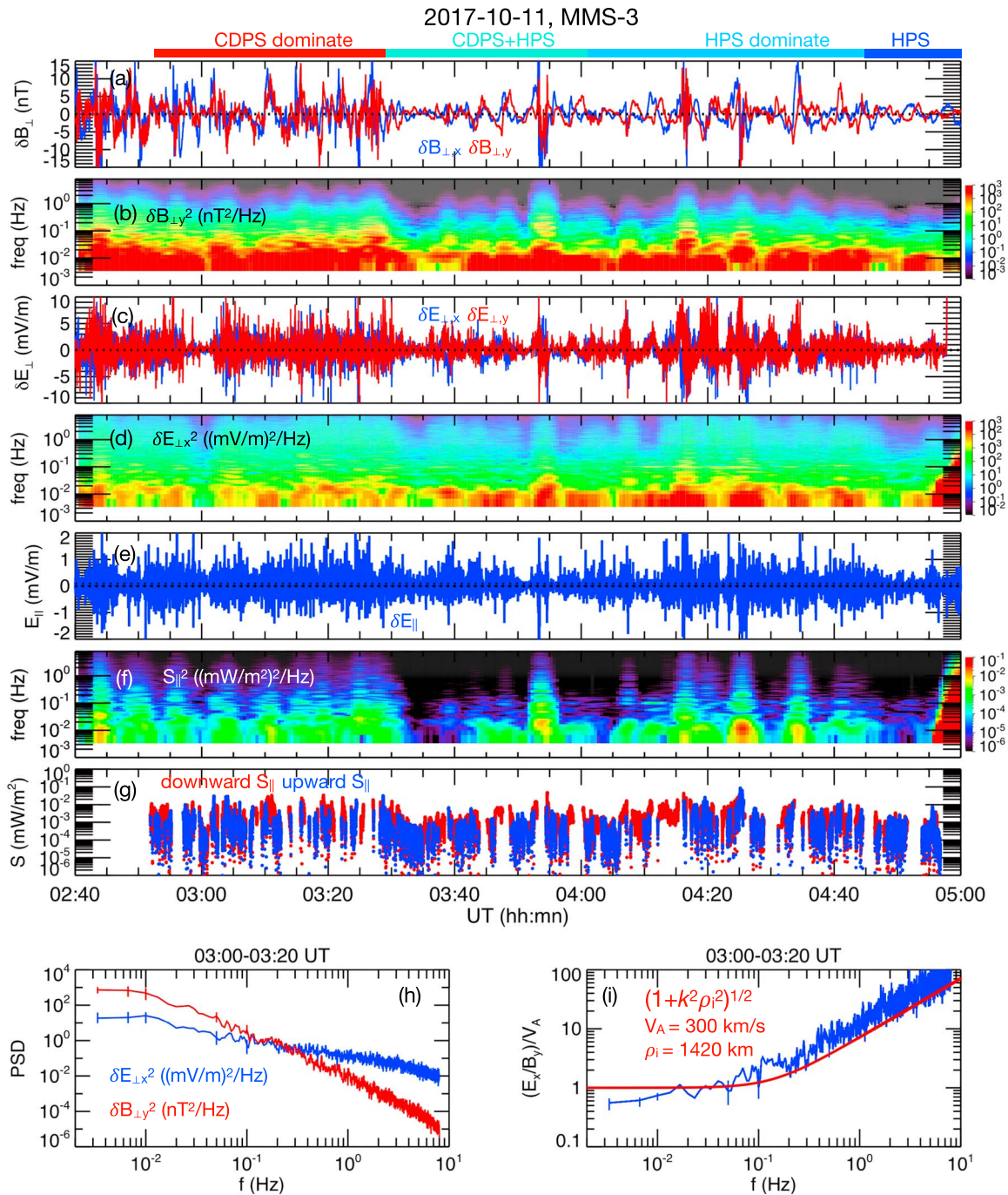
Figure 8. Event 2 on 11 October 2017. The MMS-3 observations of (a) magnetic field perturbations in the two perpendicular directions, \delta B_{\perp x} and \delta B_{\perp y} , (b) power spectrum of \delta B_{\perp y} , (c) electric field perturbations in the two perpendicular directions, \delta E_{\perp x} and \delta E_{\perp y} , (d) power spectrum of \delta E_{\perp x} , (e) electric field perturbations in the parallel direction, (f) power spectrum of parallel Poynting flux, and (g) the downward (red) and upward (blue) Poynting flux within the CDPS. Medium values of (h) PSD of \delta E_{\perp x} and \delta B_{\perp y} and (i) ratio of \delta E_{\perp x}/\delta B_{\perp y}/V_A within 03:00–03:20 UT. The red line in (i) is the KAW dispersion. CDPS = cold-dense plasma sheet; HPS = hot plasma sheet; MMS = Magnetospheric Multiscale; PSD = power spectral density.
