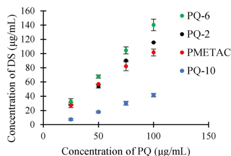
Fig. 6. Calibration curves of four different PQs. These data are calculated based on the titration curves found in Figure 5.
