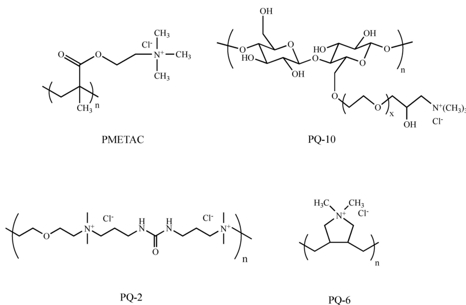
Fig. 4. Chemical structures of four different PQ species indirectly detected using all-solid-contact paper-based polyanion-sensitive ISEs.
