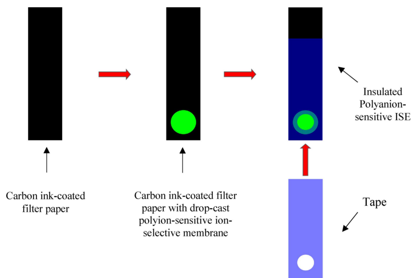
Fig. 1. Fabrication process of paper-based all-solid-contact polyanion-sensitive ISEs.
