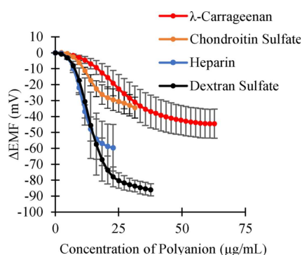
Fig. 3. Dose-response curves of four different polyanions. Each data point represents the \Delta EMF ( \pm s.d.) per concentration of polyanion from three different polyanion sensors placed in the same solution.
