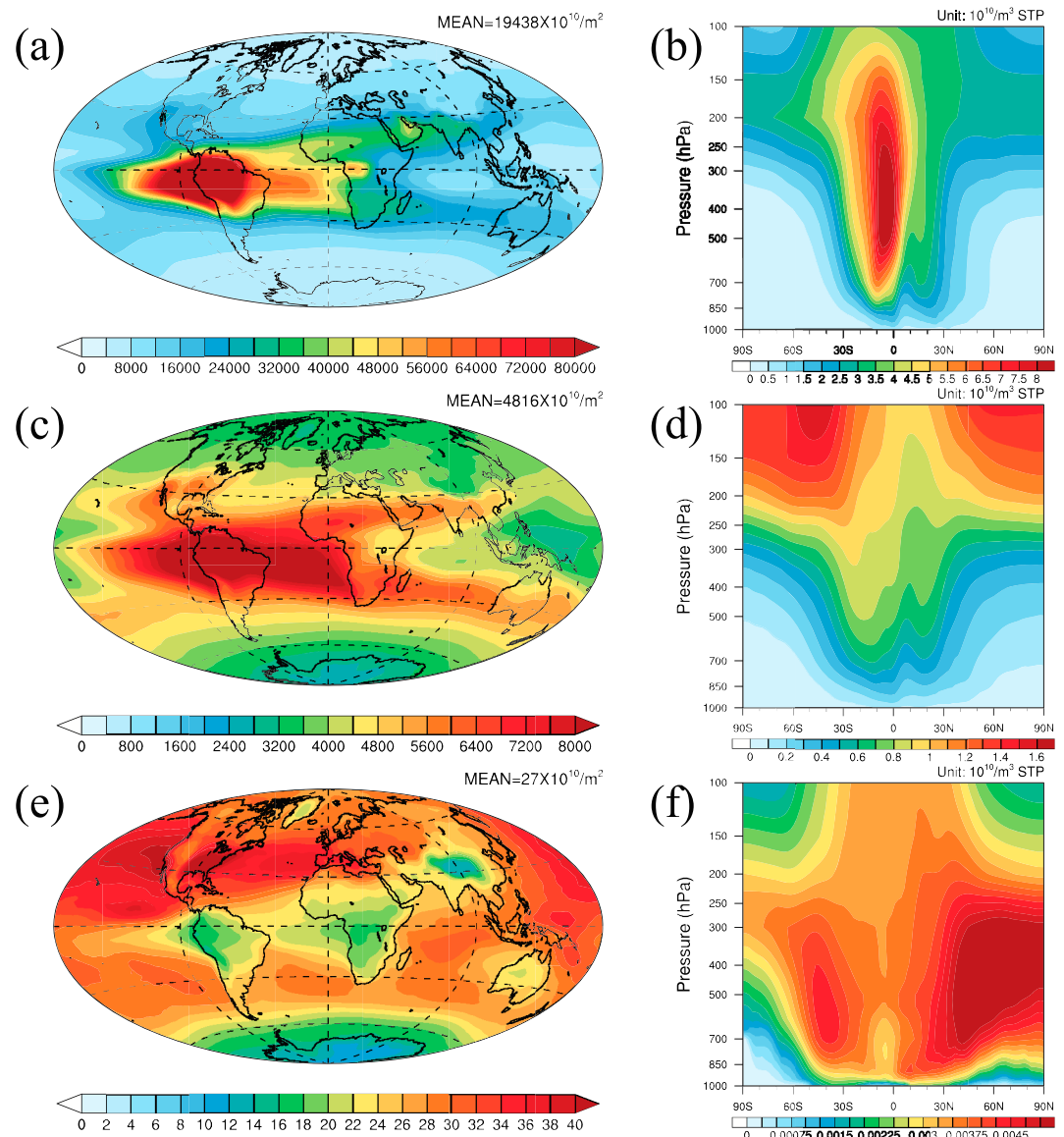
Figure 5. The annual average column number concentration (a, c, e) and zonal average number concentration (b, d, f) of newSOA in the nucleation mode (a, b), Aitken mode (b, d) and accumulation mode (e, f) for the BASE case. Note that the color bars limits vary for each mode.
