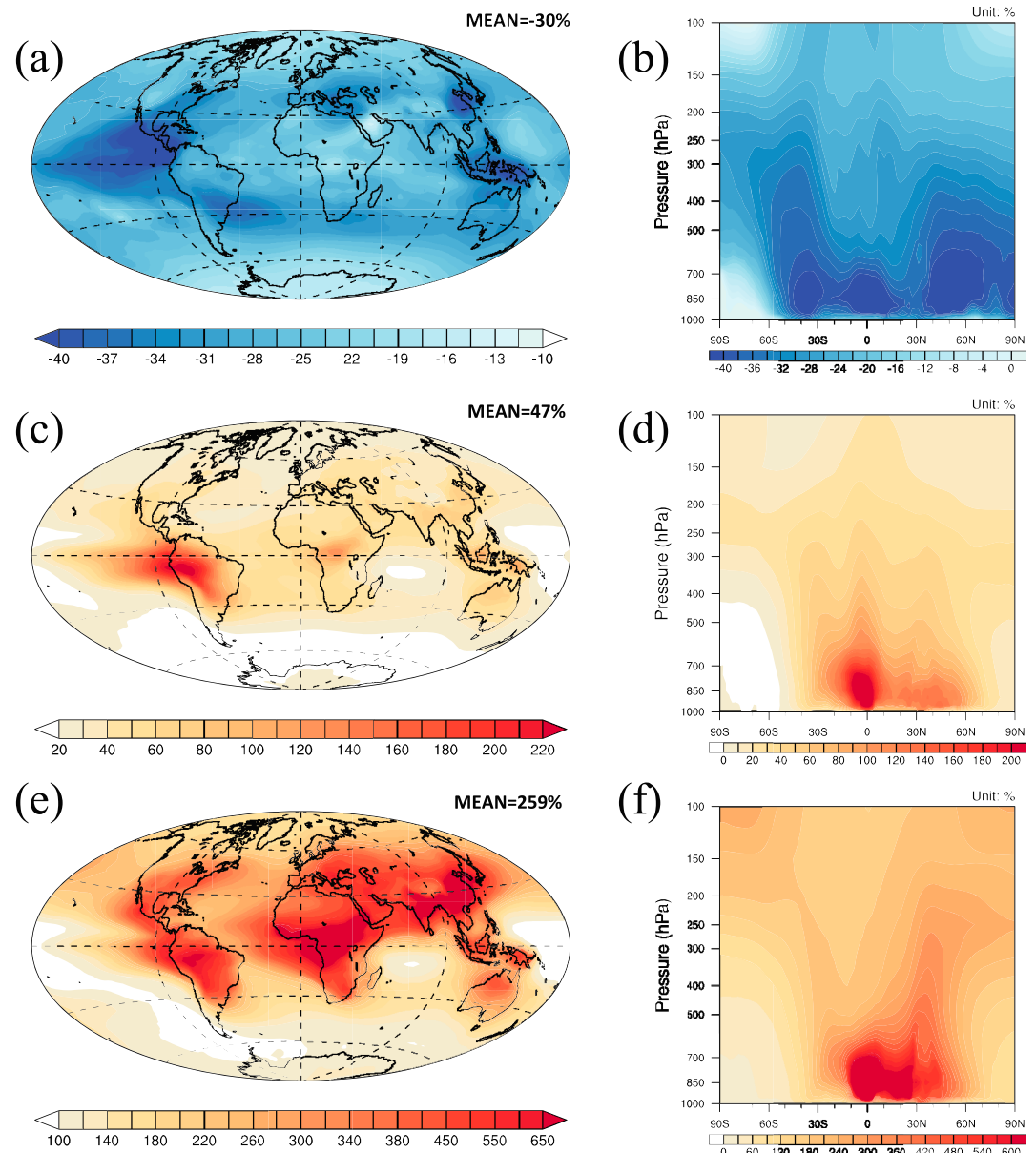
Figure 11. The annual average percentage difference in column number concentration (a, c, e) and zonal average number concentration (b, d, f) of newSOA in the nucleation mode (a, b), Aitken mode (b, d) and accumulation mode (e, f) between EX1 and the BASE case.
