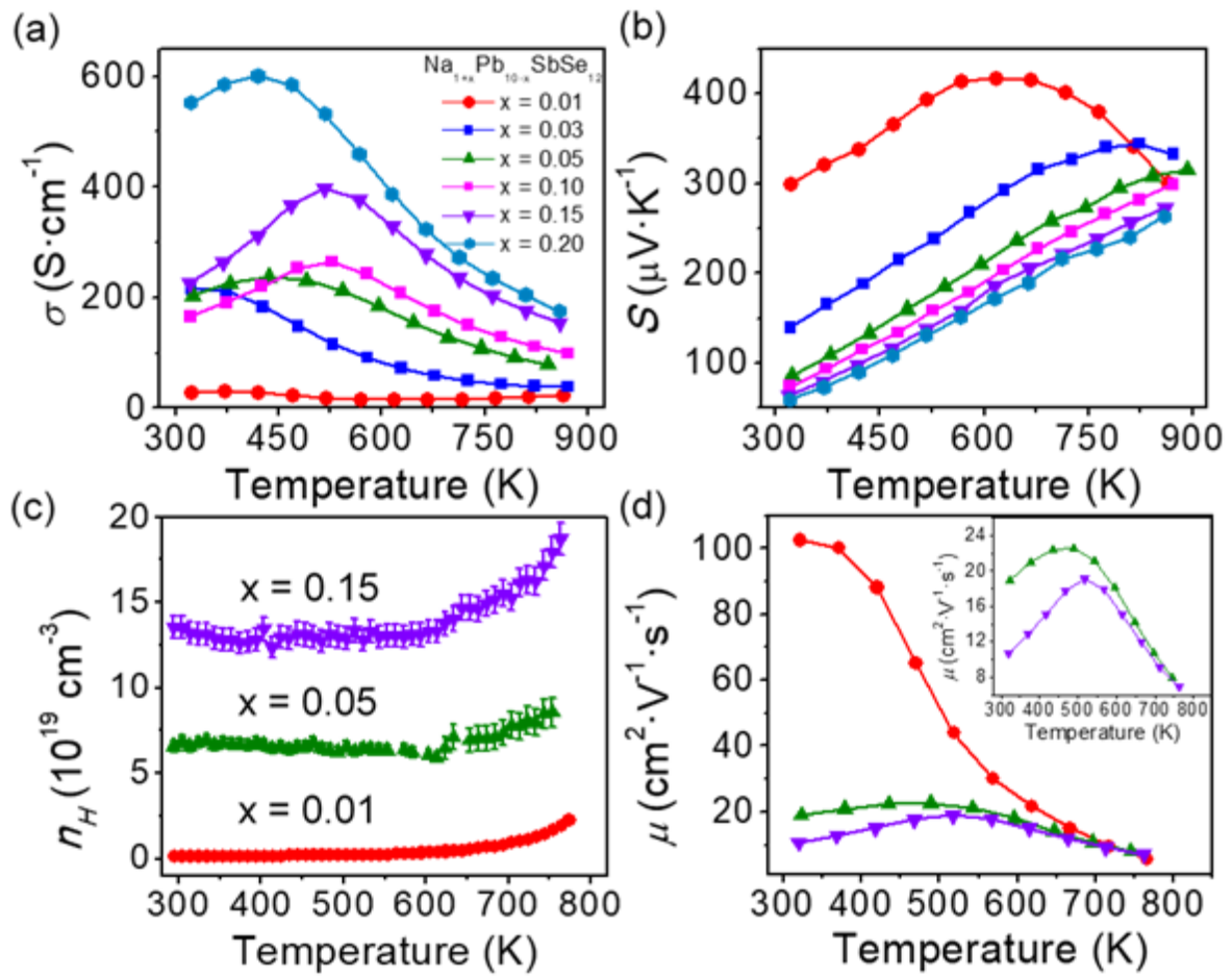
Figure 3. Temperature-dependent (a) electrical conductivities, (b) Seebeck coefficients, (c) Hall carrier densities, and (d) Hall carrier mobilities for \text{Na}_{1+x}\text{Pb}_{10-x}\text{SbSe}_{12} . The inset in (d) shows a close up of the mobilities of samples for which x = 0.05 and 0.15 , emphasizing the positive temperature dependence of \mu below 500 K.
