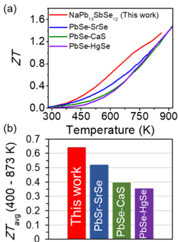
Figure 8. (a) Traces of the temperature-dependent ZT values for Na 1.10 Pb 10 Sb 0.90 Se 12 (this work, denoted as NaPb 10 SbSe 12 ), PbSe-SrSe, [17] and PbSe-CaS, [18] PbSe-HgSe. [16] The line for Na 1.10 Pb 10 Sb 0.90 Se 12 was obtained from the averages of 5 separate samples (see Figure S10). (b) Comparison of the estimated ZT avg for the compounds shown in (a), considering cold and hot side temperatures of 400 and 873 K respectively.
