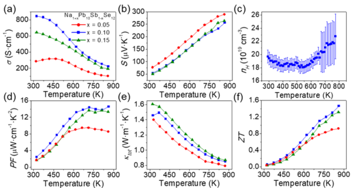
Figure 5. Temperature-dependent thermoelectric properties of \text{Na}_{1+x}\text{Pb}_{10}\text{Sb}_{1-x}\text{Se}_{12} . (a) electrical conductivity, (b) Seebeck coefficient, (c) Hall carrier concentration for x = 0.10 , (d) power factors, (e) total thermal conductivities, and (f) ZT.
