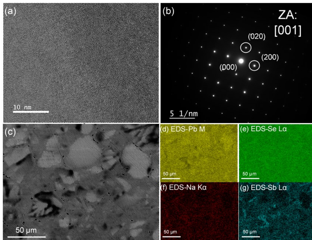
Figure 2. (a) A characteristic high-resolution TEM image of a sample with nominal composition \text{Na}_{1.15}\text{Pb}_{9.85}\text{SbSe}_{12} and (b) a selected area electron diffraction pattern, both confirming a clean rocksalt structure with no nanoscale precipitates. (c) Backscattered electron image showing noticeable micron-level Z-contrast, and (d-g) EDS elemental maps over the region shown in (c). The EDS maps confirm minor elemental segregation into Pb-rich regions and Na/Sb-rich regions.
