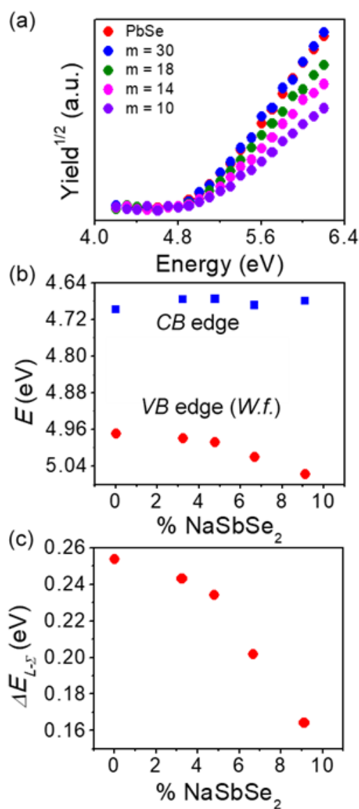
Figure 7. (a) Photoemission yield spectroscopy in air (PYS) spectra for nominally undoped samples of \text{NaPb}_m\text{SbSe}_{m+2} ( m = 10\text{--}30 , and pure PbSe). (b) Energies of the valence band edges (work functions) and conduction band edges for each sample extracted from the linear regions of the photoemission spectra, shown as red and blue points respectively. 9% NaSbSe 2 corresponds to the m = 10 sample discussed most thoroughly in the text. (c) Experimentally estimated energy differences between L - and \Sigma -valence band for each sample.
