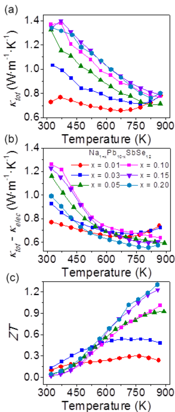
Figure 4. Temperature-dependent (a) total thermal conductivities, (b) estimated lattice thermal conductivities ( \kappa_{tot} - \kappa_{elec} ) and (c) ZTs for \text{Na}_{1+x}\text{Pb}_{10-x}\text{SbSe}_{12} .
