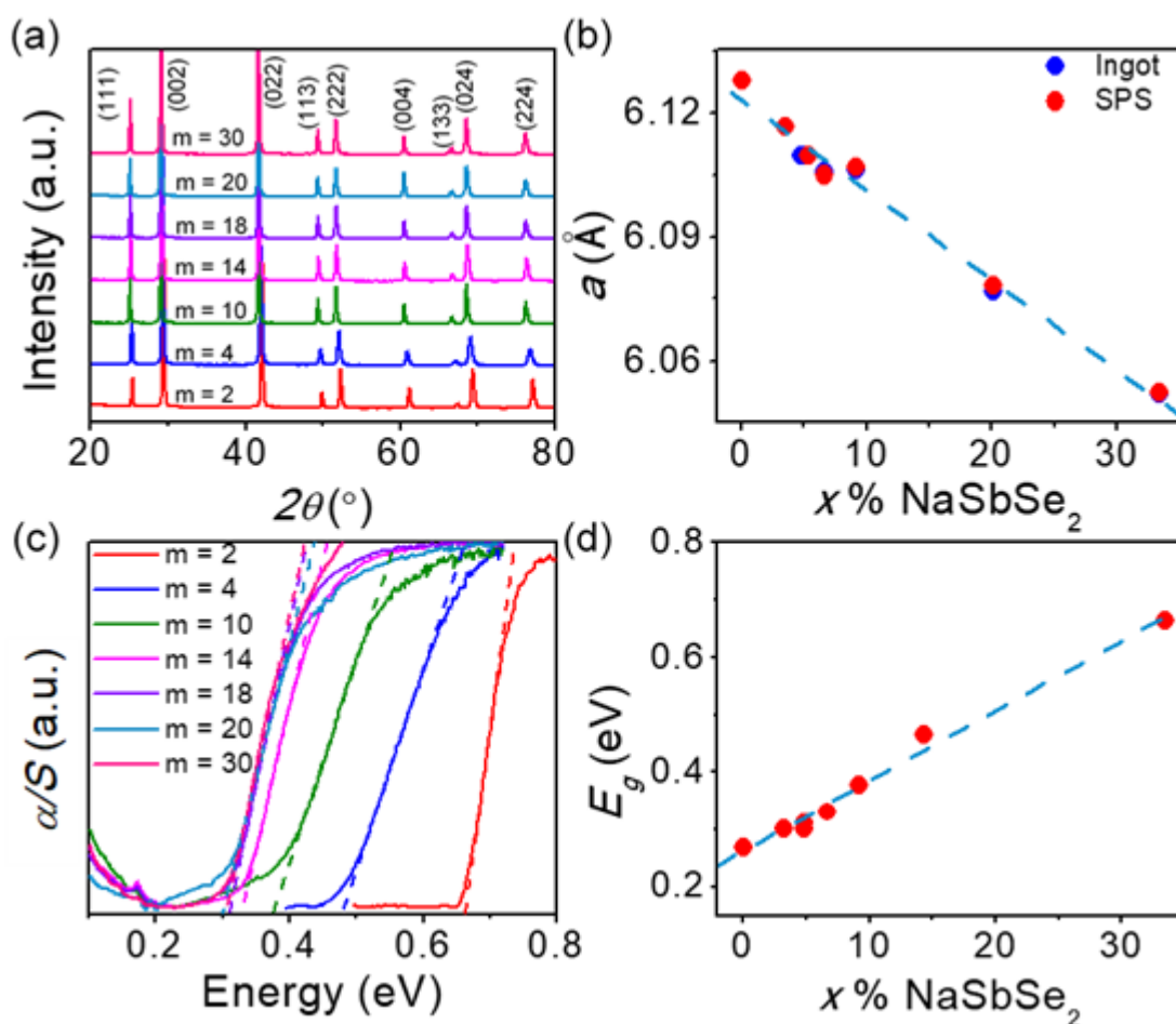
Figure 1. (a) Powder X-ray diffraction patterns for \text{NaPb}_m\text{SbSe}_{m+2} ( m = 2\text{--}30 ). (b) Refined lattice parameters for \text{NaPb}_m\text{SbSe}_{m+2} , represented as \text{PbSe} + x\% \text{NaSbSe}_2 . (c) Fourier transformed infrared spectroscopy spectra for the same \text{NaPb}_m\text{SbSe}_{m+2} compounds (the dashed lines show the extrapolation used to estimate the band gaps) and (d) the estimated band gaps. The dashed blue lines in (b) and (d) are guides to the eye showing the approximately linear trends in lattice parameter and band gap as functions of \text{NaSbSe}_2 content. Unless noted, the data shown above was obtained from samples after SPS sintering.
