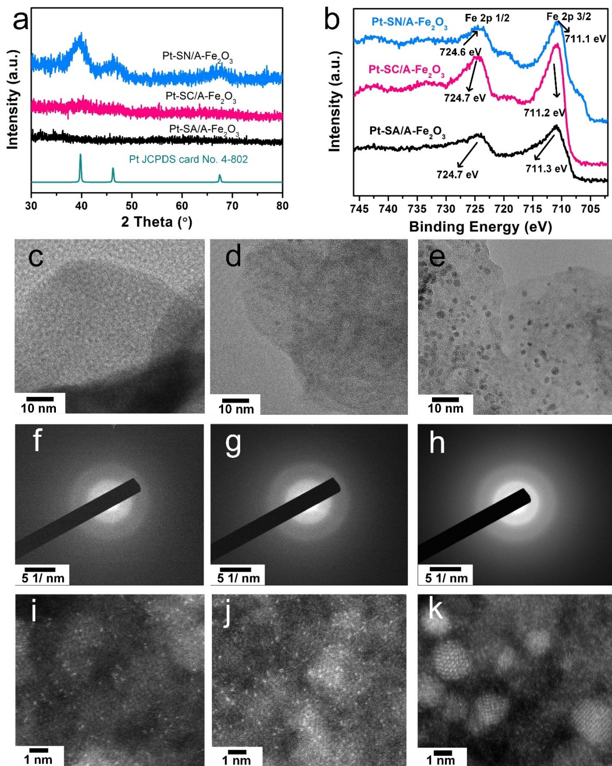
Figure 2. Nanoscale Structural characterizations of the three different Pt catalysts on the amorphous \text{Fe}_2\text{O}_3 support. (a) XRD and (b) XPS of as-prepared Pt-SA/A- \text{Fe}_2\text{O}_3 , Pt-SC/A- \text{Fe}_2\text{O}_3 , and Pt-
