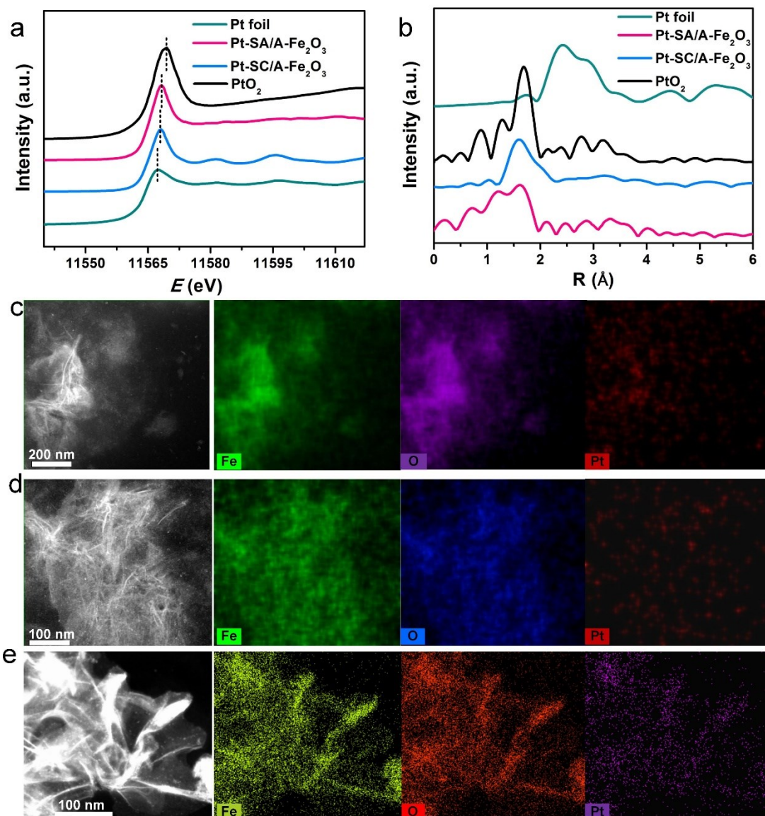
Figure 3. XAFS and EDX mapping study. Normalized (a) XANES and (b) EXAFS spectra of the Pt-SA/A-Fe 2 O 3 and Pt-SC/A-Fe 2 O 3 , and the HAADF and corresponding STEM-EDS elemental mapping, of (c) Pt-SA/A-Fe 2 O 3 , (d) Pt-SC/A-Fe 2 O 3 , (e) Pt-SN/A-Fe 2 O 3 , respectively.
