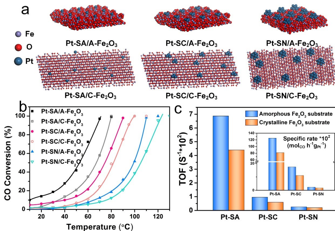
Figure 5. CO oxidation performance of the three different Pt catalysts on the two \text{Fe}_2\text{O}_3 supports. (a) Schematic of the different Pt/ \text{Fe}_2\text{O}_3 structures, different sizes were used to distinguish the elements, (b) CO conversion, the different color curves represent the fitting curves for the CO performances based on the temperatures of different catalysts, respectively, (c) TOFs and specific rates (inset).
