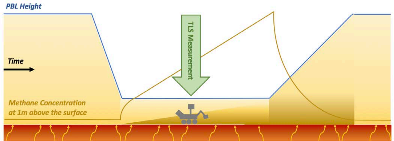
Figure 1: Schematic concept of how atmospheric concentrations of methane (shown by the Gold curve, not to scale) at 1 m should react to a constant low level of micro-seepage if the background concentration of methane in the atmosphere is close to zero. The PBL thickness, which corresponds to the layer of well-mixed air next to the surface is shown by the blue curve and is not to scale with nighttime values in meters compared to km during the day. Note how concentrations of methane rise overnight once atmospheric mixing can no longer distribute this material throughout the column. As indicated by the green arrow, it is at these times that the
