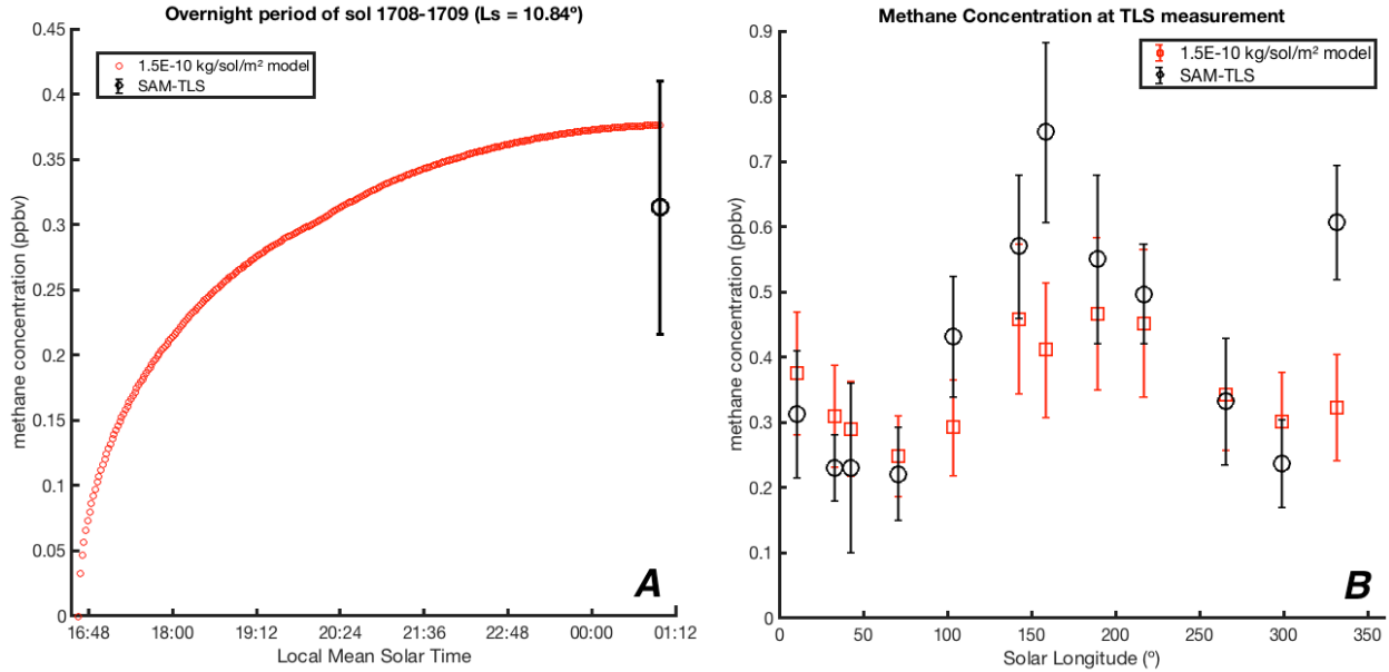
Figure 2: (A) A detailed examination of a single overnight simulation for the sol 1709 ( L_S = 10.8^\circ ) case from the time of PBL collapse up until the middle of the TLS ingest at 1:12 LMST. Note how levels of methane rise quickly near the surface once vigorous mixing ends. Error bars on the model are derived from REMS data as in Moores et al (2019), Error bars on the measurement are 1 SEM, and individual values do not include the 8% systematic uncertainty in the enrichment factor of 25 \pm 2 . (B) A comparison between modelled values of methane concentration using a modified version of the micro-seepage model of Moores et al (2019) with the enthalpy of adsorption set to 25 \text{ kJ mol}^{-1} and the seepage rate set to 1.5 \times 10^{-10} \text{ kg m}^{-2} \text{ sol}^{-1} . The quality of fit shown in this panel is \chi_v = 1.28 when the point at L_S = 331^\circ is excluded as an outlier that may represent a small plume.
