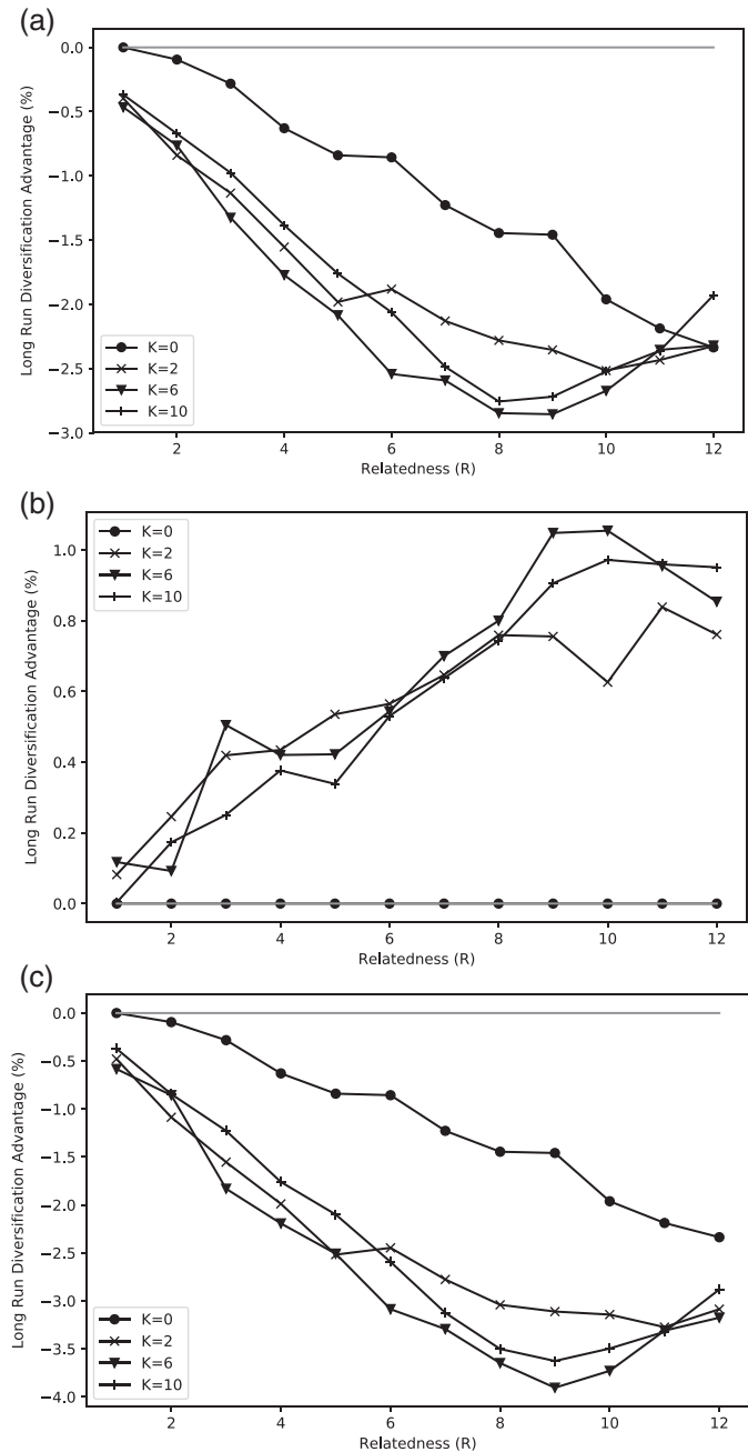
FIGURE 4 (a) Long run effects of coordination between businesses. (b) Cross-business learning benefits. (c) Rigidity effect
