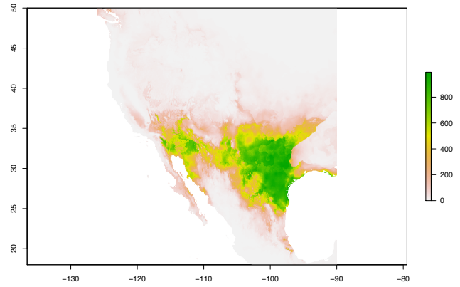
Crotalus scutulatus
