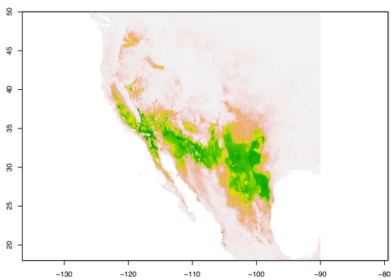
Rhinocheilus lecontei
