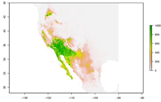
Salvador hexalepis
