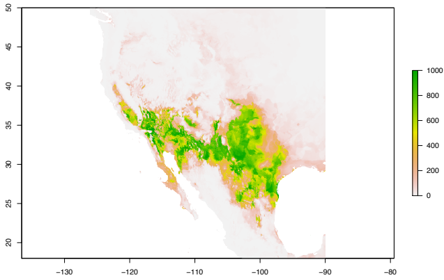
Crotalus molossus
