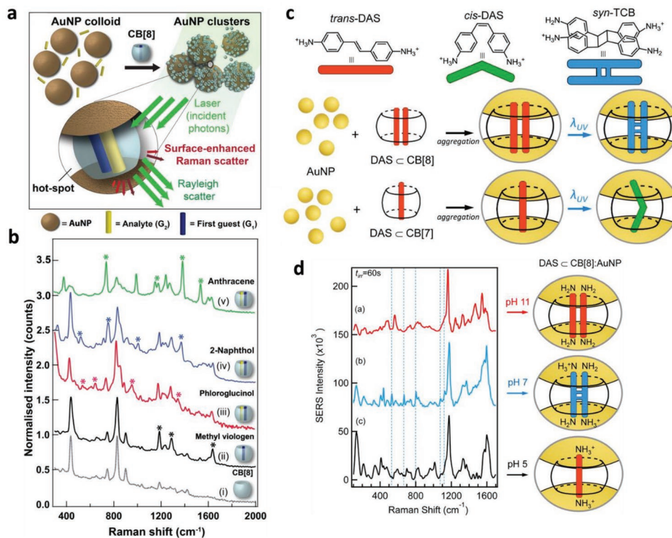
Figure 2. a) Schematic representation of Au NP aggregation induced by CB[8], which enables SERS detection of polyaromatic hydrocarbons through the formation of a ternary supramolecular complex. b) SERS spectra of CB[8] in i) the absence and ii–v) in the presence of different PAHs and a fixed electron-deficient guest ( 5 \times 10^{-6} M). Reproduced with permission. [41] Copyright 2012, American Chemical Society. c) Schematic of diaminostilbene (DAS) photodimerization and photoisomerization in the presence of CB[8] and CB[7], respectively. d) SERS spectra of DAS and the photodimerization product when encapsulated in CB[8] between NPs. Reproduced with permission. [43] Copyright 2013, American Chemical Society.
