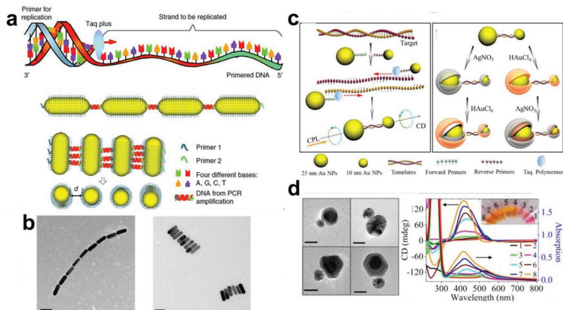
Figure 7. a) Schematic illustration of Au NR assemblies formed by PCR. b) TEM images of end-to-end (upper) and side-by-side (down) Au NR assemblies. Reproduced with permission. [66] Copyright 2013, Nature Publishing Group. c) Schematic illustration of Au NP dimers assembled by PCR and subsequent shell deposition. d) TEM images and CD spectra of Au NP dimers after Ag shell deposition. 1–8 correspond to Au NP dimers after deposition using 0, 5, 10, 20, 30, 50, 70, and 100 \mu\text{L} of 1 \times 10^{-3} M \text{AgNO}_3 solution. Reproduced with permission. [84] Copyright 2014, American Chemical Society.
