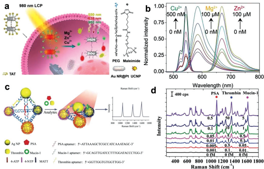
Figure 9. a) Schematic illustration of triple-ion aptamer-driven AuNR@Pt dimer-UCNP satellites. b) Fluorescence spectra of assemblies for the simultaneous detection of \text{Cu}^{2+} , \text{Mg}^{2+} , and \text{Zn}^{2+} . Reproduced with permission. [99] Copyright 2019, Wiley-VCH. c) Schematic illustration of three types of aptamer-driven Ag pyramids. d) SERS spectra of Ag pyramids for the simultaneous detection of PSA, Mucin-1, and thrombin. Reproduced with permission. [106] Copyright 2015, Wiley-VCH.
