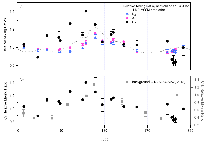
Figure 12. (a) The instantaneous mixing ratios of N_2 , Ar, and O_2 (Figure 7, Table S1) are normalized to their values at MY 31, L_S 344.9^\circ , and plotted on top of the MGCM output for relative Ar mixing ratio within Gale Crater. Similar models have produced seasonal variations in Ar at low latitudes that are on the same scale ( \pm 10\% ) (Lian et al., 2012). (b) The background seasonal CH_4 abundance reported in Webster et al. (2018) is shown here as the instantaneous mixing ratio (right axis), normalized to L_S 330^\circ (MY 32), which allows for comparison to the O_2 measurements (left axis, replotted as in the top panel). Correlations between CH_4 and O_2 are addressed in section 4.2.2.
