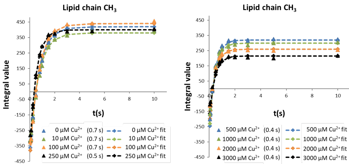
Figure S9: All the fitting for the lipid chain CH 3 peak inversion recovery experiment data recorded on polymer nanodisc samples with concentrations of Cu 2+ varying between 0 and 3000 \mu\text{M} . The triangles represent the data and the dashed lines are the fits. The spectra were recorded on a 500 MHz NMR spectrometer at 25 °C.
