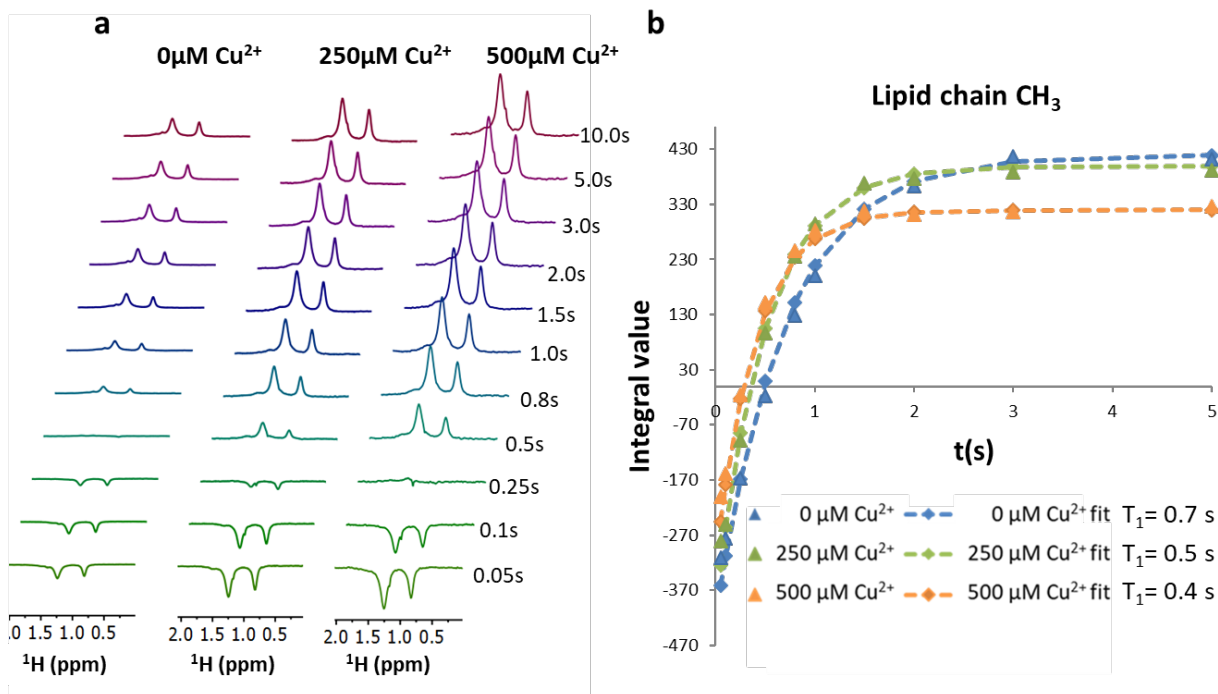
Figure S8: a) Inversion recovery experiments at different [Cu 2+ ] concentrations focused on the lipid chain CH 3 peak. b) Fitting of the lipid chain CH 3 peak inversion recovery experiment data and determination of the T 1 times. The experiments were conducted at 0, 250 and 500 \mu\text{M} concentrations. The triangles represent the data and the dashed lines are the fits. The spectra were recorded on a 500 MHz NMR spectrometer at 25 °C.
