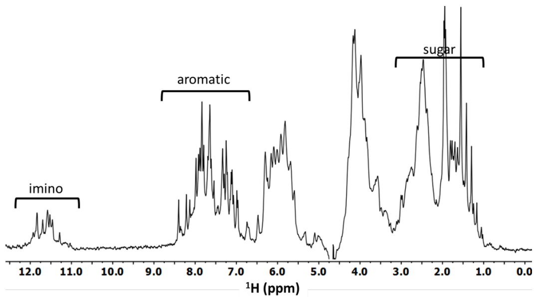
Figure S11: 1D 1 H NMR spectrum of the wtTel23 G-quadruplex. The spectrum was recorded at 0.1 mM oligonucleotide concentration per strand, 100 mM KCl, pH~7.0 and 25 °C on a 500 MHz spectrometer. The amino, aromatic, and sugar (H 2 '/H 2 '') regions are indicated in the above spectra.
