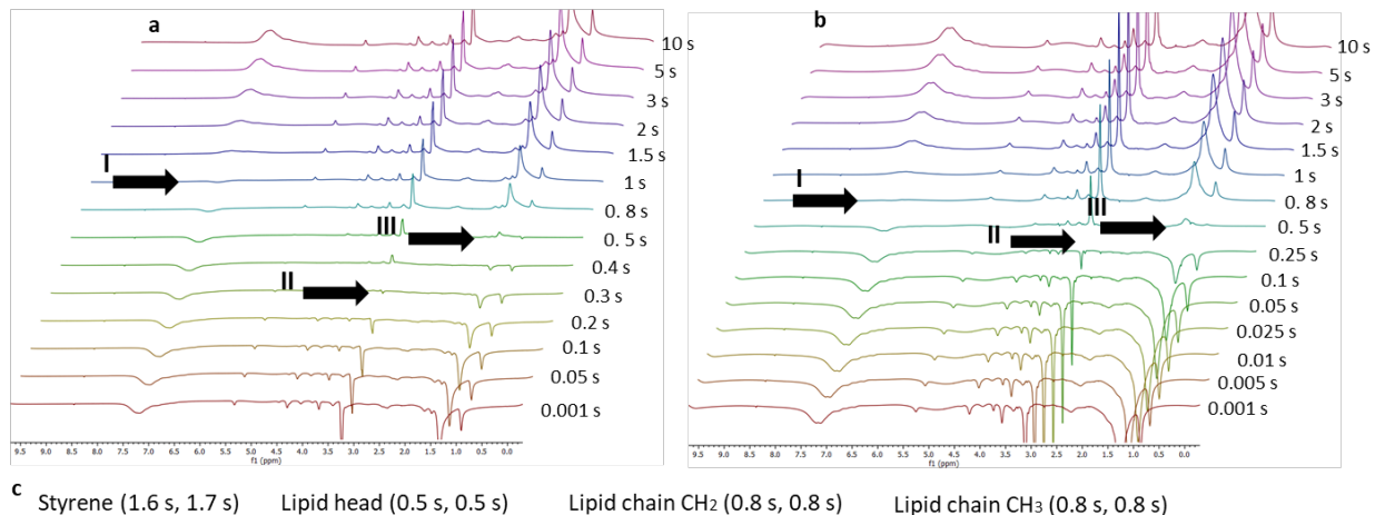
Figure S10: SMA EA nanodisc without the addition of the DOTA chelator in absence and presence of Cu 2+ ions. a) The SMA-EA nanodiscs in absence of Cu 2+ ions b) The SMA-EA nanodiscs in presence of 500 μM Cu 2+ ions. c) The T 1 values for styrene, lipid head, lipid chain CH 2 and lipid chain CH 3 signals. The first number is the value for the nanodisc in the absence of Cu 2+ ions. The second number is the value for the SMA-EA nanodiscs in presence of 500 μM Cu 2+ ions. Roman numerals I, II and III indicate where the intensities of styrene, lipid head and lipid chain peaks, respectively are close to or zero. The spectra were recorded on a 500 MHz NMR spectrometer at 25 °C.
