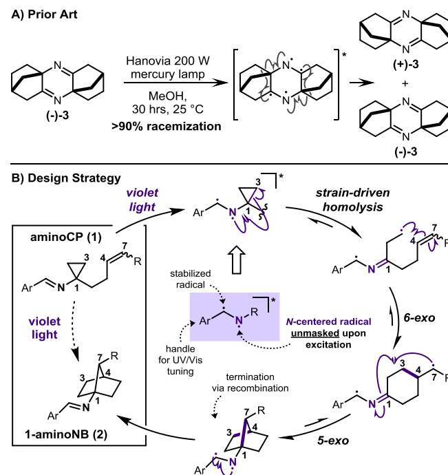
Figure 2. Imine-based photochemistry and the design of our masked N-centered radical strategy. A) Photo-racemization of dihydropyrazine (-)-3 with UV light 42 (of note, all necessary electron-pushing arrows are depicted, but this is not expected to be a concerted process); B) Design principles
