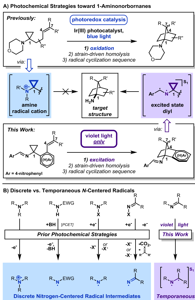
Figure 1. 1-Aminonorbornanes through Photochemical Innovation. A) Comparison of our photochemical strategies toward 1-aminonorbornanes. B) Comparison of existing approaches for the production of nitrogen-centered radicals with our masked N -centered radical strategy.
