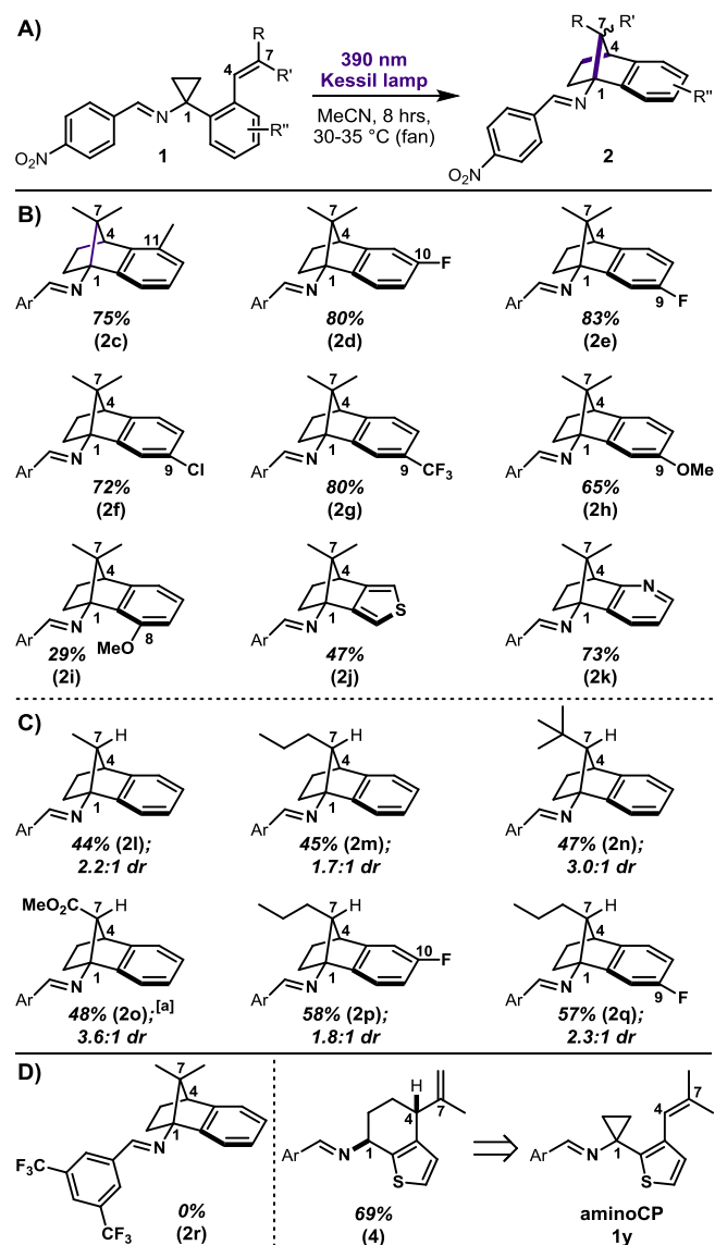
Figure 5. Reaction Scope. A) Generic reaction scheme; all reactions were run on ~200 \mu\text{mol} scale and degassed via three freeze-pump-thaw cycles prior to exposure to optimized conditions; Ar = 4-nitrophenyl. B) Arene modifications. C) C7-substitution effects; [a] C7-CO 2 Me substrate proceeded in 3.6:1 anti:syn dr based on crude 1 H NMR, but was isolated in 48% yield in >20:1 dr (an additional 10-15% of a 1:5 anti:syn mixture was collected along with minor impurities). D) Deviations from designed reactivity.
