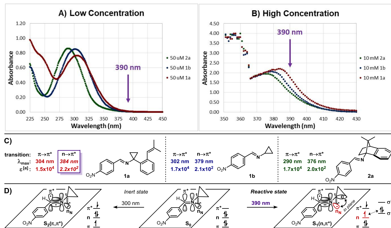
Figure 3. UV/Vis data and proposed mechanism of cyclopropane fragmentation. A) UV/Vis data for cyclopropylimines 1b and 1a and 1-aminoNB 2a collected at 50 \mu M in MeCN; B) UV/Vis data collected at 10 mM in MeCN; C) Structures and data summary; [a] molar absorptivities ( \epsilon ) estimated from peak absorbance at single concentration; D) Depiction of in-plane donation from cyclopropyl \sigma_{CC} to singly-occupied n_N orbital in S_1(n, \pi^*) state.
