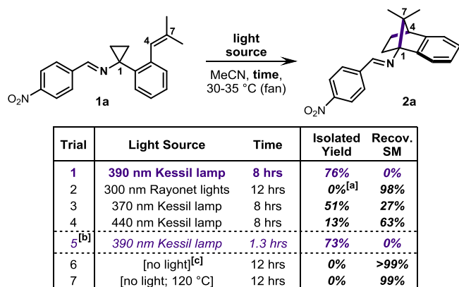
Figure 4. Optimization of light source for photochemical production of 1-aminoNBs. Reactions were run on ~200 \mu mol scale and degassed prior to irradiation via three freeze-pump-thaw cycles; all reactions run in 2 dram borosilicate vials except entry 2 (quartz tube) and entry 5 (TPFA tubing), see Supplementary Information; [a] No product was isolated, but an estimated 1-2% was detected by crude 1 H NMR; [b] Trial 5 was run in continuous flow (see Supplementary Information for details on flow apparatus); [c] Vial was wrapped in black electrical tape to exclude light prior to exposure to standard batch conditions.
