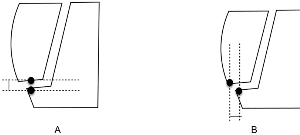
Fig. 4. A) Schematic representation of the vertical marginal fit to be evaluated in the Micro CT. B) Horizontal marginal fit.
