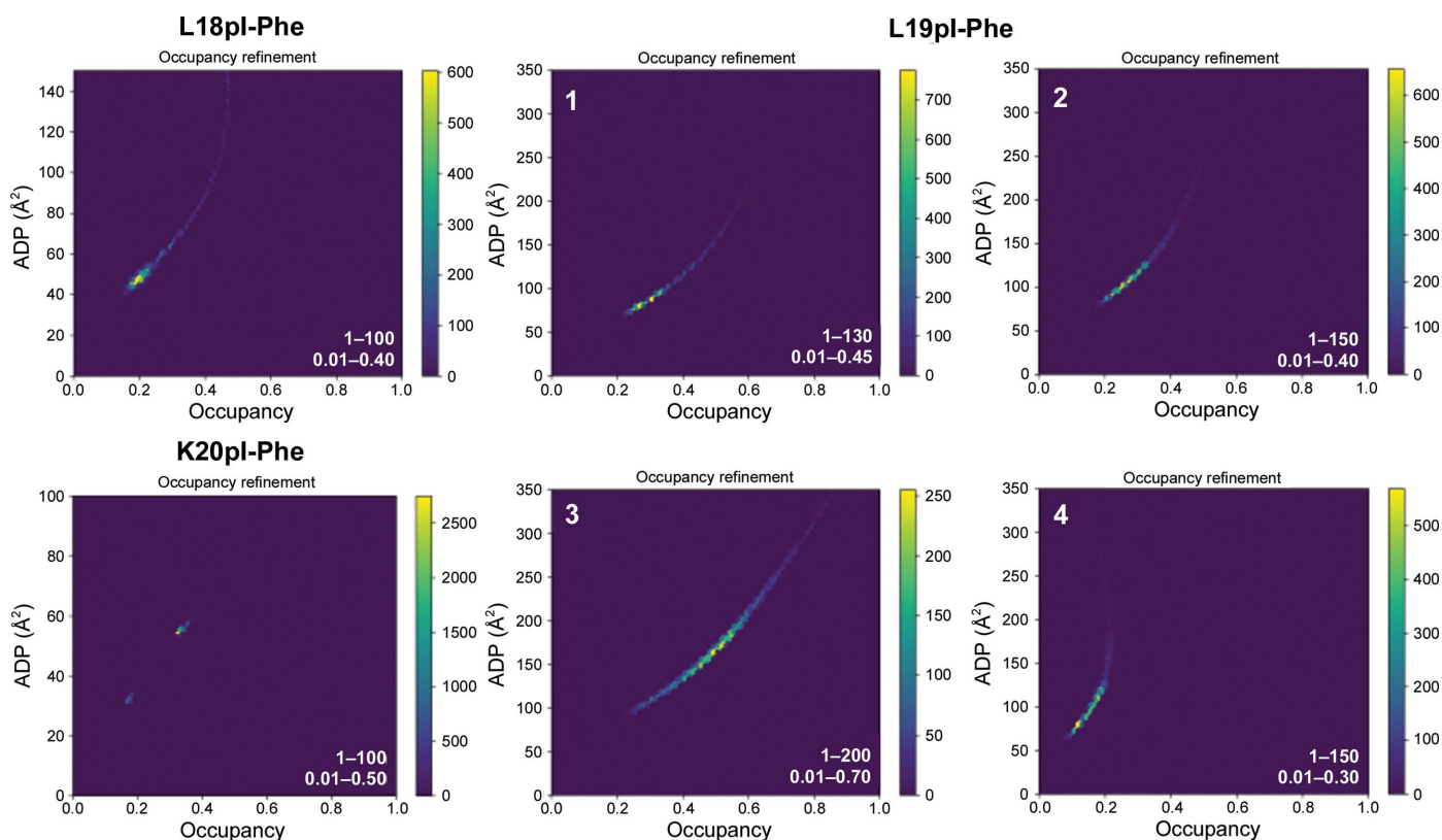
Figure 2 2D histogram showing occupancy refinement of the iodine positions in the three structures, L18pI-Phe (PDB entry 6owx), L19pI-Phe (PDB entry 6owz) and K20pI-Phe (PDB entry 6owv), after 50 rounds of refinement from 10 000 randomly assigned ADP/occupancy starting values (shown in Supplementary Fig. S3). The color scale represents the number of structures in the bin. The starting-value ranges for ADP and occupancy are shown in the bottom right corner of each plot.
