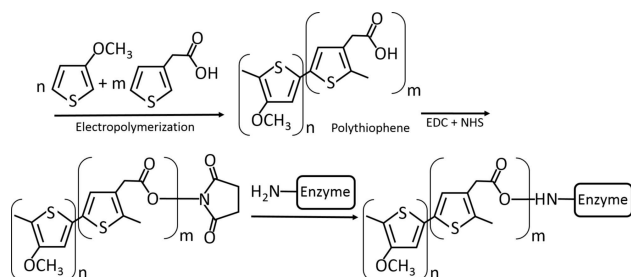
Figure 4. The scheme showing preparation of the electropolymerized polythiophene sub-layer, further modified with covalently bound enzymes. Note the ratio of the original thiophene-monomers n:m=2:1 .
