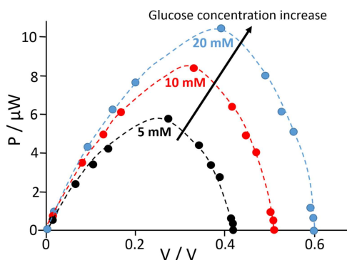
Figure 7. Power release function measured with the biofuel cell filled with 50 mM phosphate buffer, pH 7.4, containing 100 mM \text{Na}_2\text{SO}_4 and different concentrations of glucose: 5 mM, 10 mM, and 20 mM. Oxygen was always present under equilibrium with air. The circles in the plots reflect the experimental distribution of the measured parameters.
