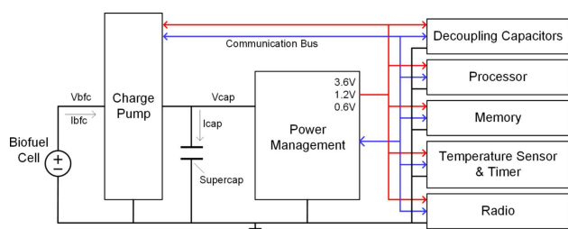
Figure 2. The electronic block scheme of the microelectronic temperature-sensing device powered by the biofuel cell. A charge pump chip converts the low voltage of the biofuel cell to voltage acceptable for operating electronic circuits. The power management chip (also containing up/down charge pumps internally) generates three stabilized voltages for the different load circuits.
