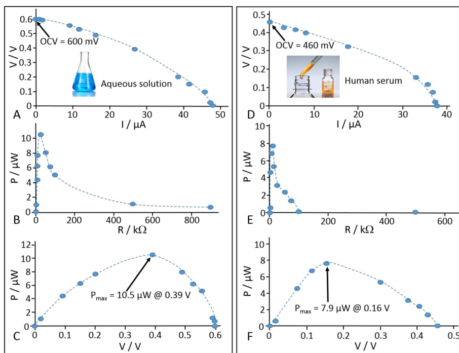
Figure 6. Biofuel cell polarization curves and power release measured: A–C) with 50 mM phosphate buffer, pH 7.3, containing 100 mM \text{Na}_2\text{SO}_4 and 20 mM glucose; D–F) with human serum containing ca. 6 mM glucose. Oxygen was always present under equilibrium with air. The circles in the plots reflect the experimental distribution of the measured parameters.
