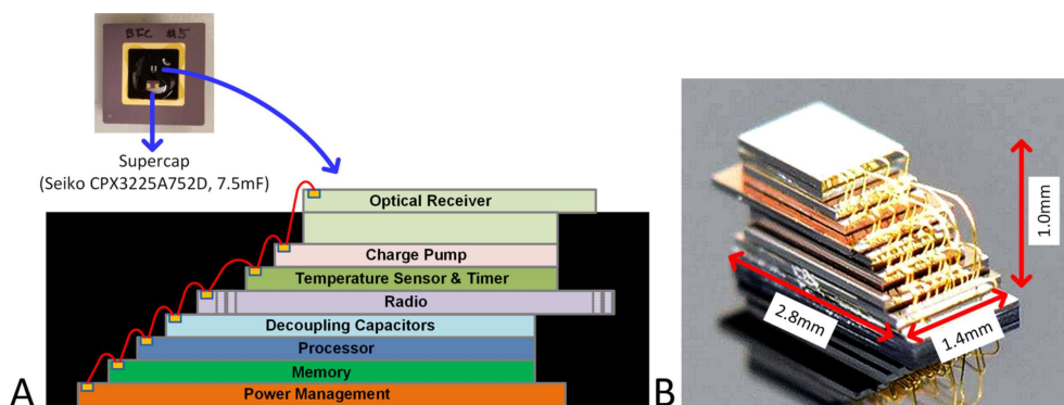
Figure 1. A) The microelectronic temperature-sensing device schematic composition. B) The stack of the chips (without encapsulation).
