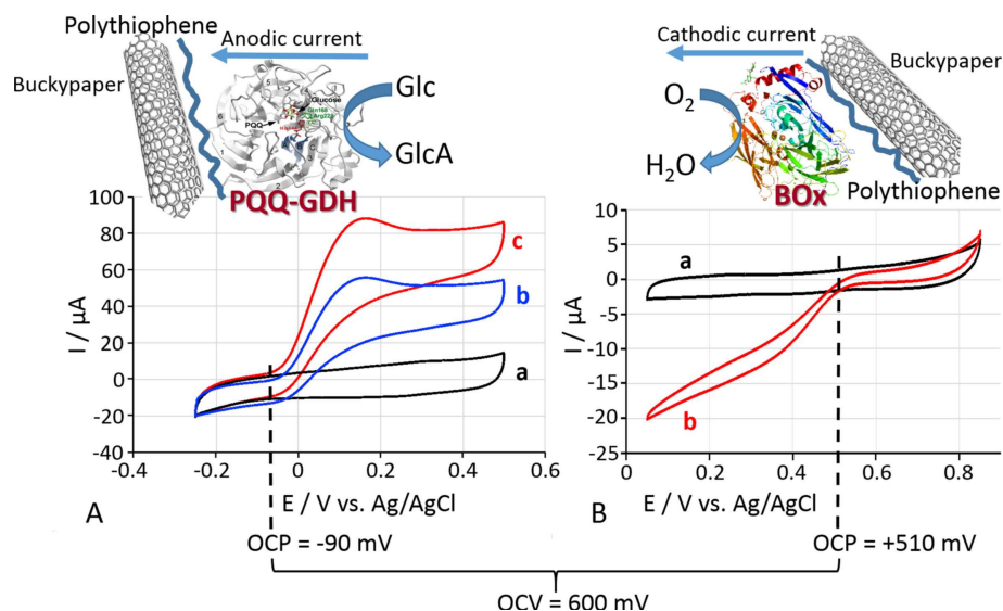
Figure 5. A) Cyclic voltammograms obtained with the PQQ-GDH-modified electrode measured in the absence (a) and presence of glucose, 5 mM (b) and 20 mM (c). B) Cyclic voltammograms obtained with the BOx-modified electrode measured under a) anaerobic conditions and b) in the presence of O_2 (in equilibrium with air). Background electrolyte was 50 mM phosphate buffer, pH 7.4, containing 100 mM Na_2SO_4 . Potential scan rate was 1 mV s -1 . Abbreviations used: PQQ-GDH: PQQ-dependent glucose dehydrogenase; BOx: bilirubin oxidase; Glc: glucose; GlcA: gluconic acid (product of Glc biocatalytic oxidation); OCP: open circuit potential (measured vs. the reference electrode); OCV: open circuit voltage (measured between two biocatalytic electrodes).
