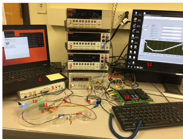
Figure 3. The experimental setup for studying the microelectronic device operation and characterizing its different components. The numbered parts of the experimental setup are as follows: (1) power supply (Agilent E3630A); (2) source meter (Keithly 2401 Sourcemeter) used in preliminary experiments (data not reported) to mimic the real biofuel cell; (3) source meter (Keithly 2400 Sourcemeter) needed to charge the supercapacitor (Seiko CPX3225A752D, 7.5 mF); (4) electrometer (Keithly 6514 System Electrometer) to monitor voltages of the M3 sensor; (5) universal software radio peripheral (USR) (Ettus, USRP X310); (6) laptop (Lenovo P51) equipped with custom programming software; (7) biofuel cell operating with a model aqueous solution, replaced with a live slug in the final system test; (8) anti-static wrist (ESD) strap used by an operator; (9) microelectronic sensor device; (10) custom light programming module; (11) custom printed circuit board (PCB) antenna for base station; (12) desktop computer using a LABVIEW program; (13) analog-to-digital converter module (National Instruments, NI-9229 & NI cDAQ-9171); (14) analog buffer PCB (Texas Instruments, OPA4354AIDR).
