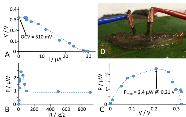
Figure 8. Biofuel cell polarization curve (A) and power release functions (B, C) measured with the biocatalytic electrodes implanted in a living slug (D). The circles in the plots reflect the experimental distribution of the measured parameters.
