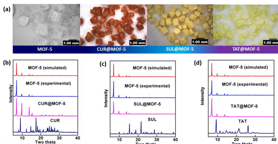
Figure 2. (a) Optical images of MOF-5 and drug@MOF-5 composite crystals. (b), (c), and (d) PXRD patterns of drug@MOF-5 composites compared with their starting materials (MOF-5 and respective drug).
