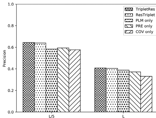
FIGURE 3 Mean precisions of long-range top L and top L/5 contacts of TripletRes and ResTriplet on FM targets, compared to the predictors trained on the component features from the covariance matrix feature (COV), the precision matrix feature (PRE) and the coupling matrix of the inverse Potts model feature (PLM)
