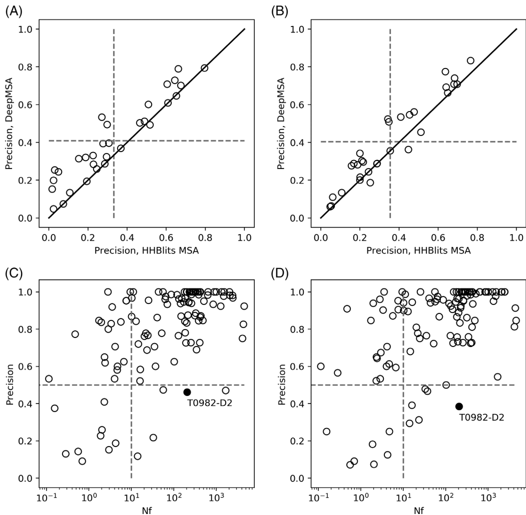
FIGURE 2 Illustration of the effect of MSAs on the performance of TripletRes and ResTriplet. A and B, Comparison of top L long-range contact prediction results using MSAs by DeepMSA vs those by the routine HHblits search for TripletRes and ResTriplet, respectively. C and D, Precision of long-range top L/5 contact prediction vs N_f of MSAs for TripletRes and ResTriplet, respectively
