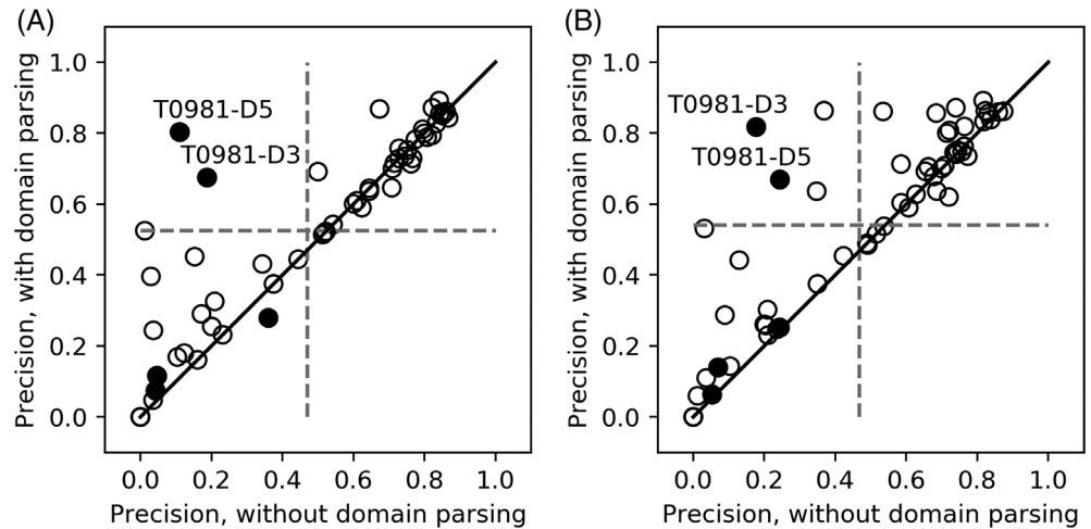
FIGURE 4 Comparison of precisions of long-range top L contact predictions with domain partitioning vs those without using domain partitioning. A, TripletRes; B, ResTriplet
