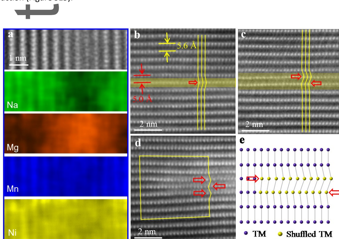
Figure 3 | Elemental reorganization induced precipitates. a , Atomic resolution EDS mapping of the P2-NMM10 cathode after 50 cycles at 2.0-4.5 V, showing the distribution of Na, Mg, Mn and Ni. (b-d) high resolution scanning electron microscopy-high angle annular dark field images. b , A single layer thick precipitate. c , A two-layer thick precipitate. Yellow regions highlight the phase transition layers whose stacking sequence is different from the P2 structure as indicated by the yellow lines. d , A multi-layer precipitate with one end terminated in the P2 structured matrix. The yellow circuit highlights a zigzag stacking sequence due to displacement along the red arrows. e , Atomic model to show the formation of a two-layer precipitate, yellow balls represent the TM cations shuffled along red arrows.
