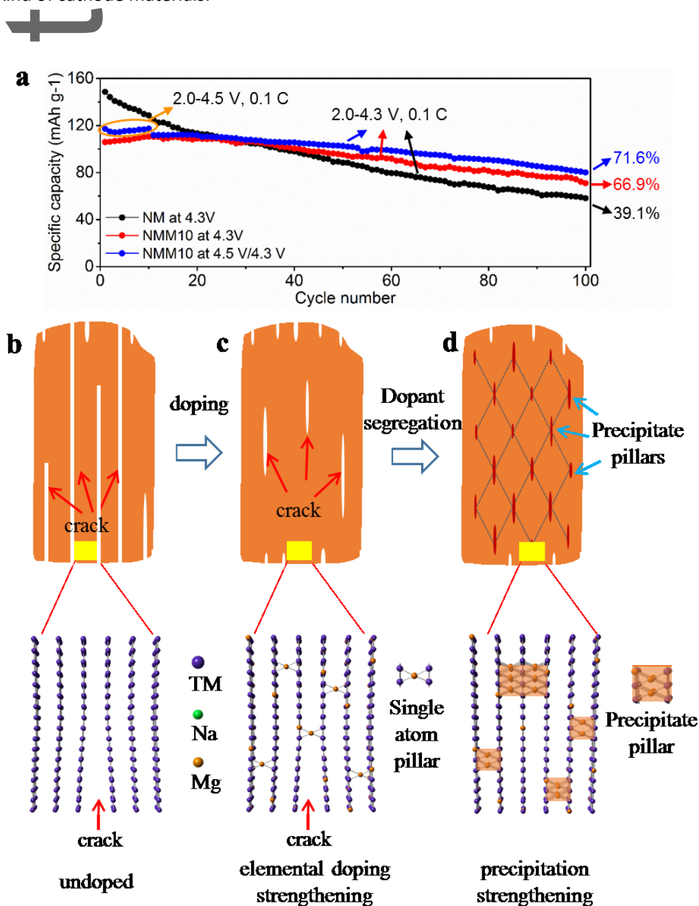
Figure 6 | Precipitation strengthening mechanism to enhance cyclability. a, Capacity retentions as a function of cycle numbers. For the undoped P2-NM sample, capacity decay is fast as shown by the black dots. For the Mg-doped P2-NMM10 sample, introducing precipitates by cycling at 4.5 V for 10
