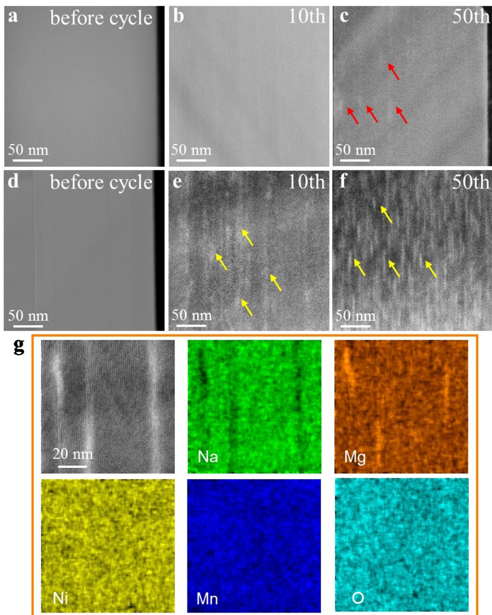
Figure 2. Electrochemical cycling inducing dopant segregation. STEM-HAADF images of the (a-c) P2-NMM05 and (d-f) P2-NMM10 cathode cycled at 2.0-4.5 V. a , Typical image from the P2-NMM05 cathode before cycle, showing a uniform contrast in grain bulk. b , No bright stripes in the P2-NMM05 cathode after 10 cycles, (c) Some bright stripes (red arrows) in the P2-NMM05 cathode after 50 cycles. d , Uniform contrast in grain bulk of the P2-NMM10 cathode before cycle. e , Low density of bright stripes (yellow arrows) in the P2-NMM10 cathode after 10 cycles. f , High density of
