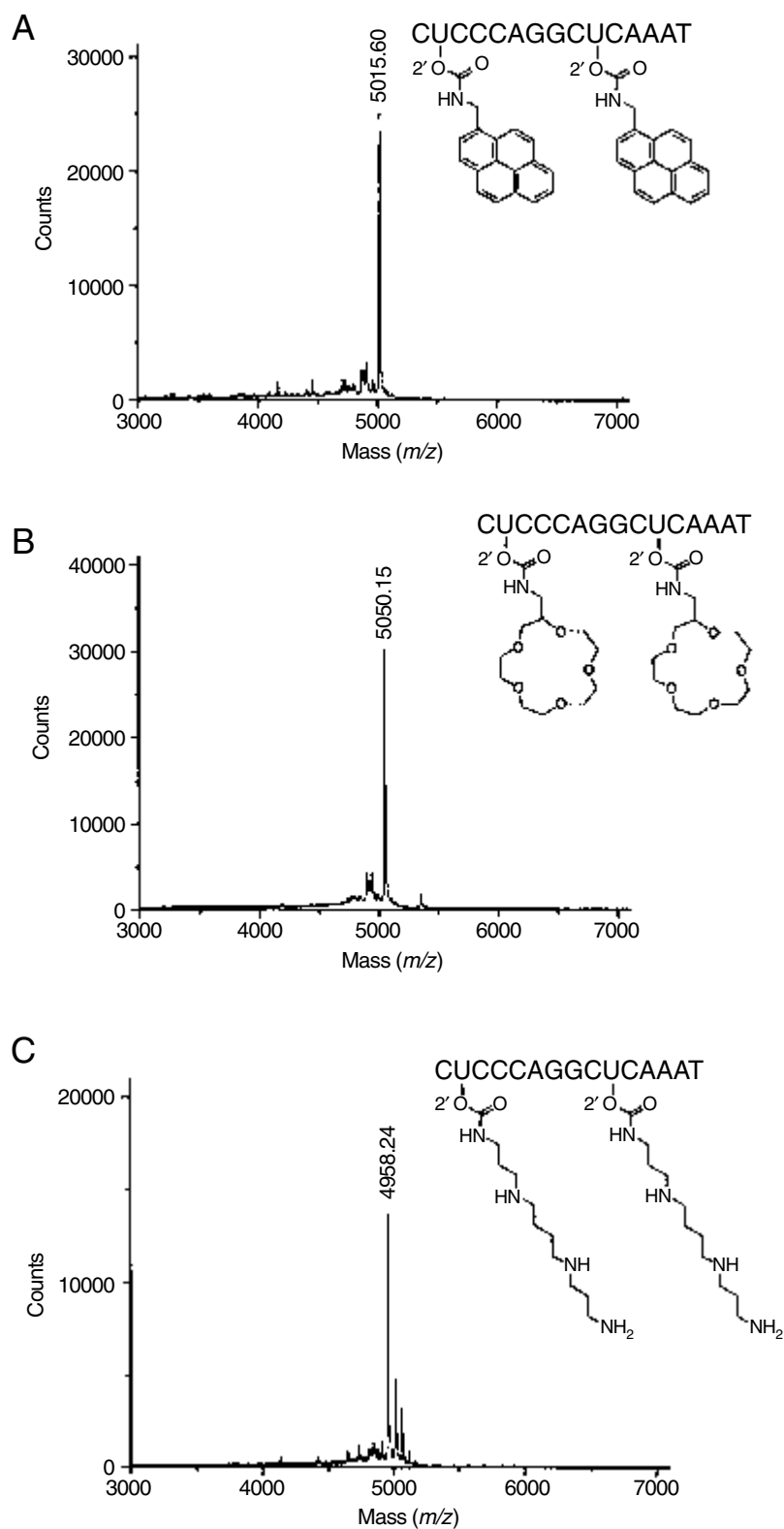
Figure 4.21.4 MALDI-TOF mass spectra of 2'-carbamate oligodeoxyribonucleotides containing two modified uridines CU*CCCAGGCU*CAAAT, where U* is from phosphoramidites S.7d (A), S.7e (B), and S.7h (C) (see Figures 4.21.1 and 4.21.2 and Table 4.21.1).
