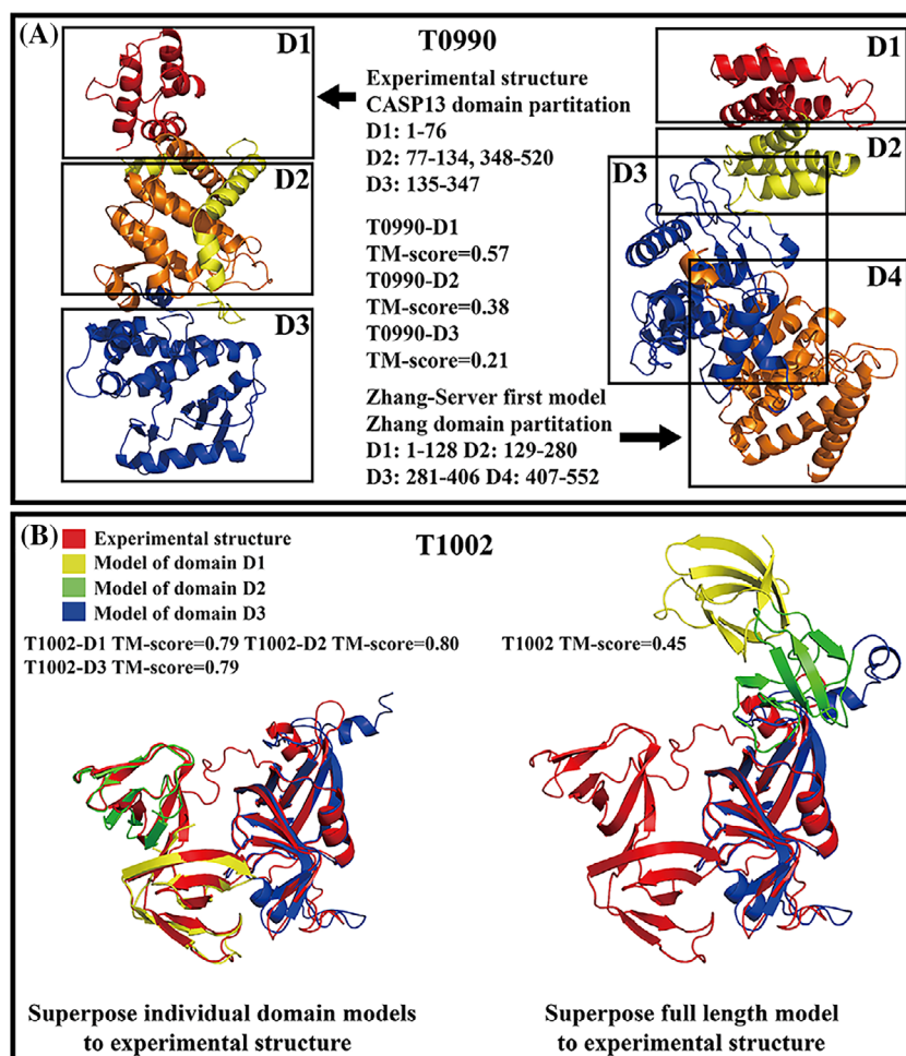
FIGURE 7 A, The structures of different domains for target T0990. Different colors represent different domains or different parts of discontinuous domains. B, The structures of different domains for target T1002. The red, yellow, green, and blue structures correspond to the experimental structure and the first C-I-TASSER model of the T1002-D1 domain, T1002-D2 domain, and T1002-D3 domain, respectively
