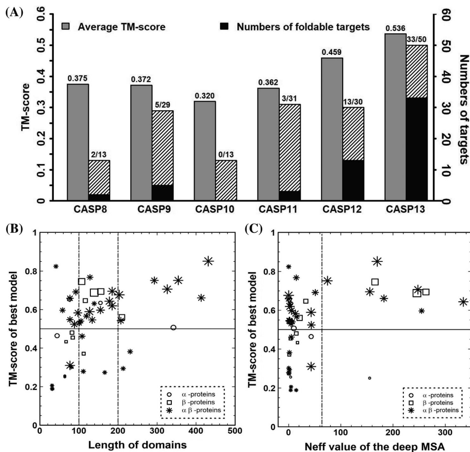
FIGURE 6 A, The folding performance for FM targets based on the best models that were submitted by “Zhang-Server” or “QUARK” from CASP8 to CASP13, the gray bar represents the average TM-score of the best “Zhang-Server” model, the black bar indicates the numbers of foldable targets (TM-score \geq 0.5 ) and the hatched bar depicts the number of non-foldable targets. B, The TM-scores of the best “Zhang-Server” or “QUARK” models for the 50 FM targets in CASP13 vs the domain lengths. C, The TM-scores of the best “Zhang-Server” or “QUARK” models for the 50 FM targets in CASP13 vs the Neff value of the deep MSA. The size of the points in B and C is proportional to the precision of the top L long-range contact prediction by NeBcon
