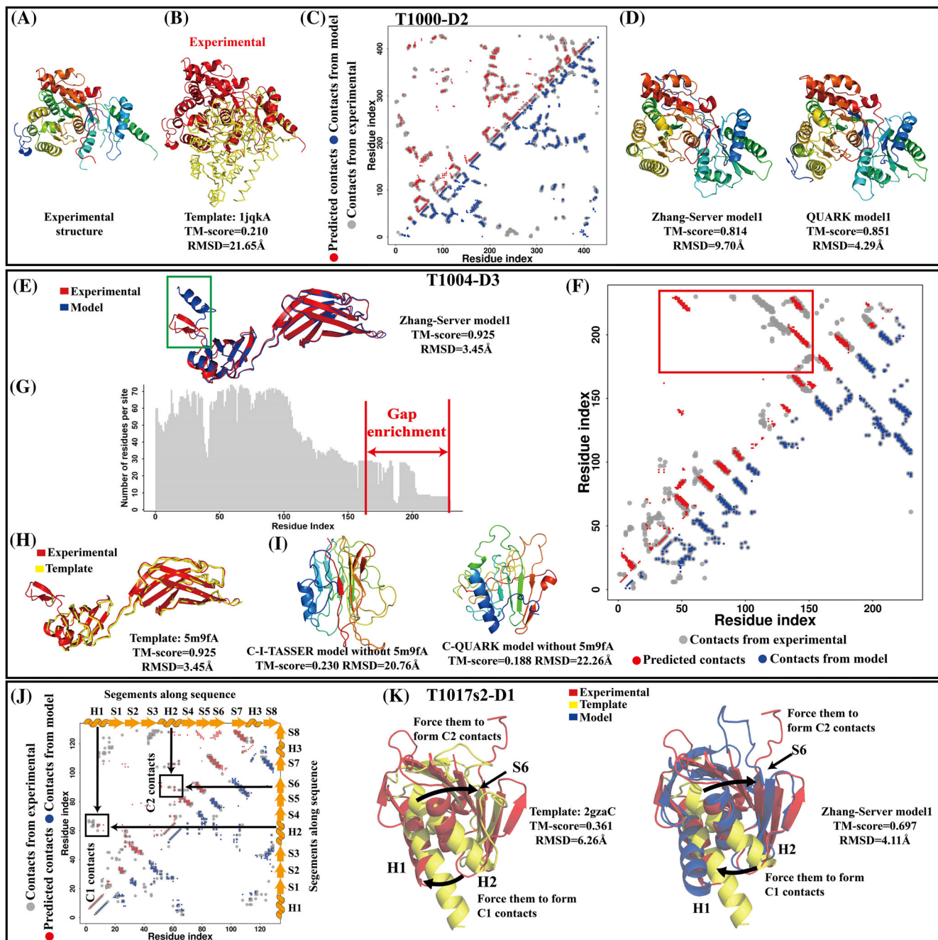
FIGURE 5 Case studies for the advantages and disadvantages of integrating predicted contacts with template information. The top panel from (A) to (D) shows the analyses for target T1000-D2, including the experimental structure (A), superposition of the experimental structure (red) and the first LOMETS template (yellow) (B), contact-map (C) and “Zhang-Server” and “QUARK” models (D). The middle panel from (E) to (I) shows the analyses for target T1004-D3, including the superposition of the experimental structure (red) and the “Zhang-Server” model (blue) (E), contact-map (F), number of effective residues in each sequence position of the deep MSA (G), superposition of the experimental structure (red) and the first LOMETS template (yellow) (H) and models generated by the control test which removed template 5m9fA (I). The false positive contacts between the terminal regions are highlighted using the red box, while the incorrect secondary structure prediction is shown using the green box in the model. The bottom panel from (J) to (K) shows the analyses for target T1017 s2-D1, including the contact-map (J) and structure superposition of the “Zhang-Server” model (blue) and first LOMETS template (yellow) with the experimental structure (red). The red points in the contact-map are the predicted contacts by NeBcon, the gray points are contacts derived from the experimental structure, and the blue points are the contacts calculated from the first model built by “Zhang-Server” in C, F, and J
