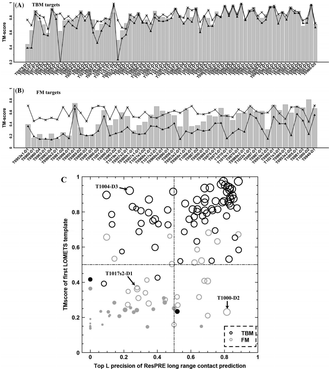
FIGURE 4 TM-scores of the first models built by “Zhang-Server” (bar), TM-align templates (crosses), and the first LOMETS templates (triangles) for the 71 TBM targets (A) and 50 FM targets (B), where the targets are sorted by the precision of the top L long-range predicted contacts. C, The relationship between folding success and TM-scores of the templates identified by LOMETS and the top L long-range contact precision by NeBcon. An empty circle means that the target is foldable (TM-score \geq 0.5 for the first “Zhang-Server” model), while a solid point means the target is not foldable (TM-score < 0.5 ). The point size is proportional to the value of the TM-score. The 71 TBM targets are shown in black and the 50 FM targets are shown in gray
