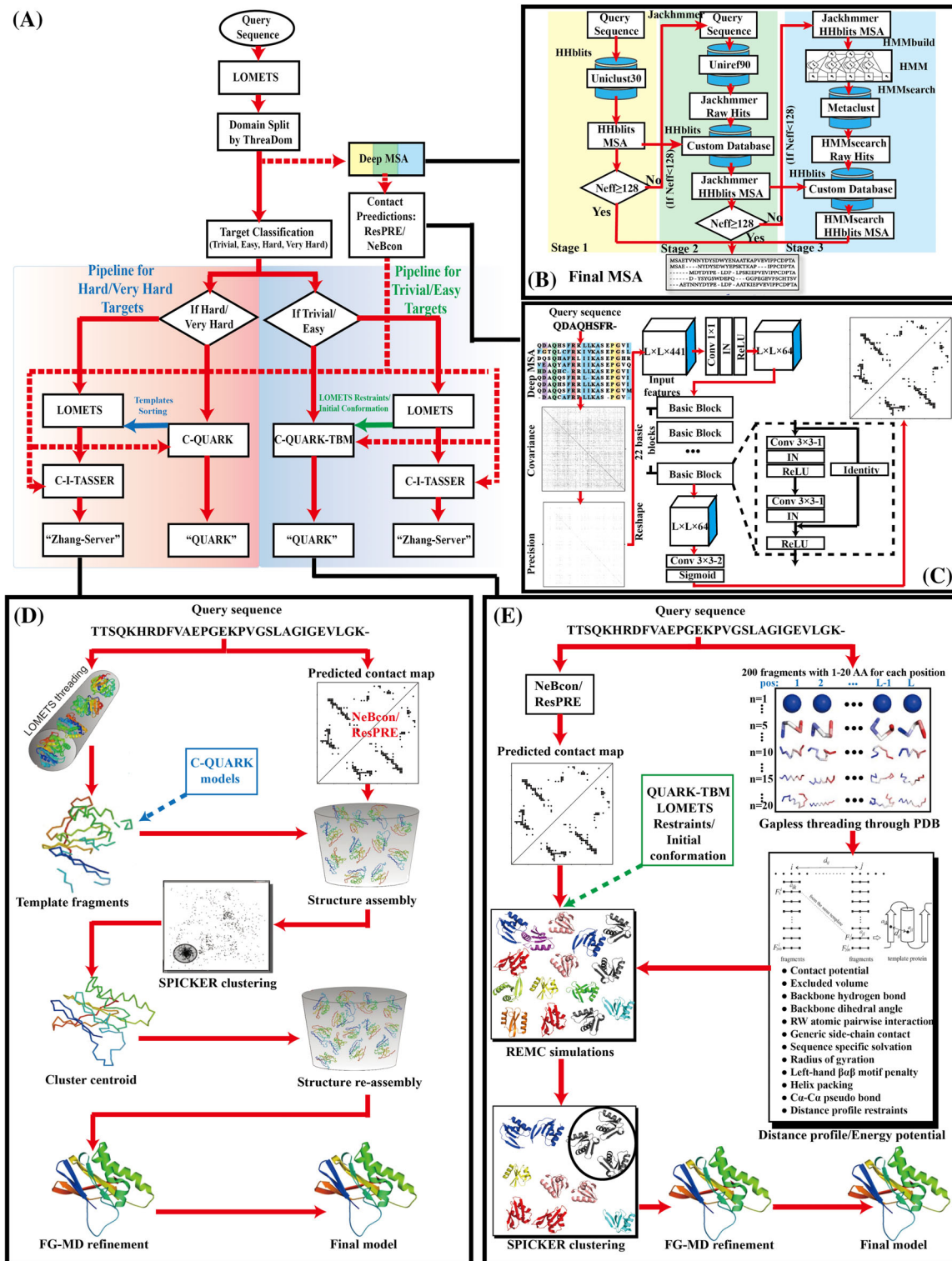
FIGURE 1 A, Automated "Zhang-Server" and "QUARK" protein structure prediction pipelines used in CASP13, including. B, MSA generation. C, ResPRE Contact prediction. D, The C-I-TASSER pipeline. E, The C-QUARK pipeline. MSA, multiple sequence alignment
