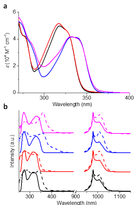
Figure 2. (a) Absorption spectra in solution (50 \mu\text{M} , DMF), and (b) corrected and normalized (left) excitation ( \lambda_{\text{em}} = 980 nm) and (right) emission ( \lambda_{\text{ex}} = 320 –350 nm) spectra collected in the solid state (dashed traces) and in solution (50 \mu\text{M} , DMF; solid traces) of Yb-I x MCs ( x = 0, 4, 8, 12 ) at room temperature. Black : Yb-I 0 ; red : Yb-I 4 ; blue : Yb-I 8 ; magenta : Yb-I 12 .
