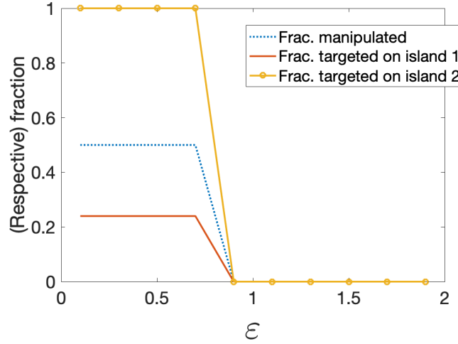
Figure 15. The principal's optimal strategy for various values of \varepsilon under some inequality. Depending on the curve, (Respective) fraction refers to either the fraction of the entire population manipulated, or the fraction of a given island that is targeted.
