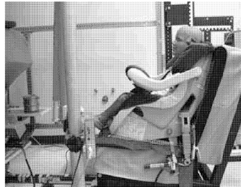
B. Convertible, forward-facing, 75° belt angle
