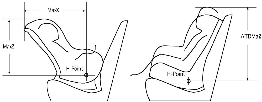
Figure 17. Schematic of dependent measures representing in-seat child restraint position.
