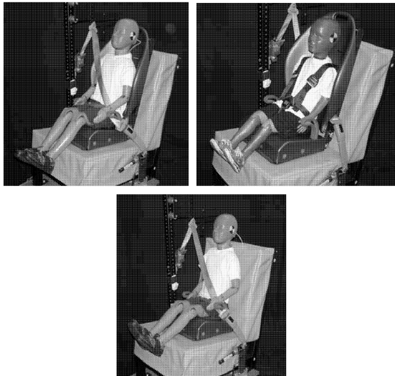
Figure 13. Final booster surrogate, from top to bottom, as a high-back booster, forward-facing-only restraint, and backless booster.
