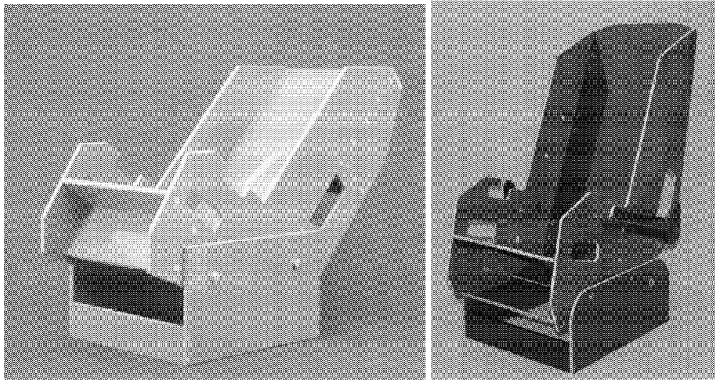
Figure 11. The first (left) and second (right) prototypes of the convertible surrogate.
