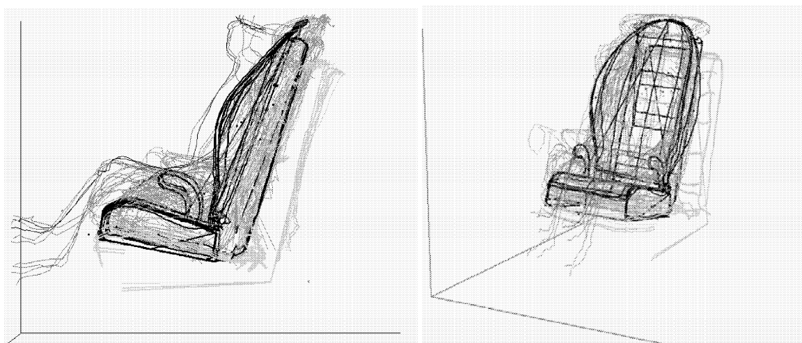
Figure 16. Overlay of booster surrogate geometry (thick lines) with data from commercial child restraints tested with the 6YO ATD and vehicle belt.
