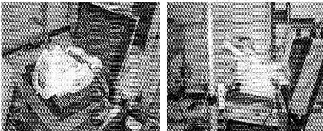
Figure 6. Xsensor pressure distribution measurement mats installed under a child restraint and on seatback.
