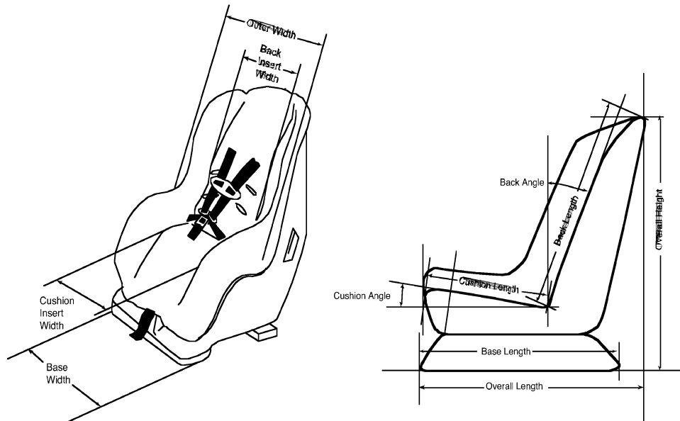
Figure 10. Definitions of child restraint dimensions in Table 6.
