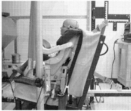
A. Convertible, forward-facing, 13° belt angle
