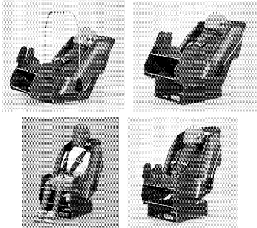
Figure 12. Final convertible surrogate prototype, from top to bottom, as a rear-facing infant seat without base, rear-facing infant/convertible with base, and forward-facing convertible with 3YO and 12-month ATDs.
