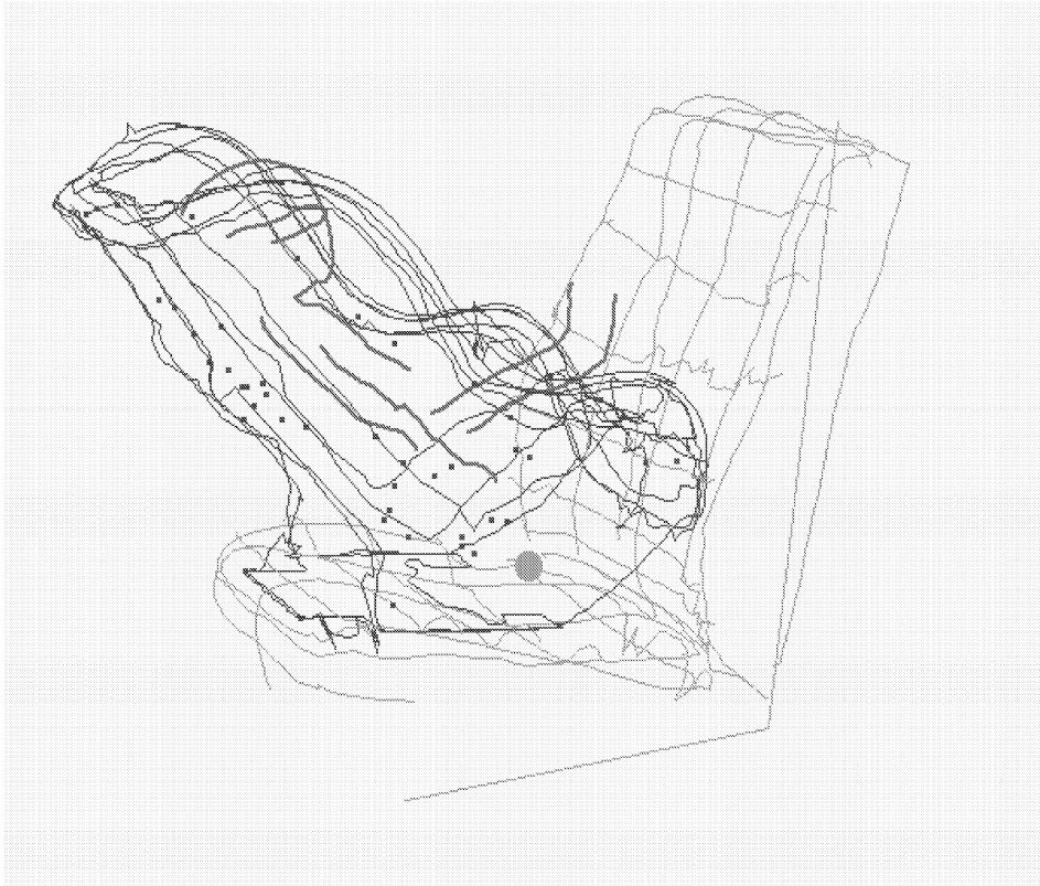
Figure 9. Geometric data from one in-seat trial obtained by combining in-seat measurements with previously measured restraint geometry aligned to reference points. Contour streams on ATD and seat surface contours are also shown. Large dot is seat H-point.
