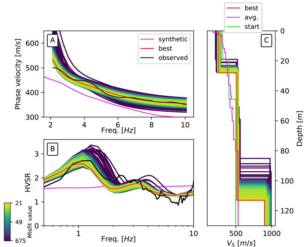
Figure 7. Joint inversion result for channel 85. (a) Dispersion curves. (b) D-HVSR. (c) V_s profiles. Starting velocity model is shown in lime green and is an harmonically averaged version of the model of Thomas et al. (2014) shown in pink. For comparison, synthetic dispersion curve and HVSR computed from the model of Thomas et al. (2014) are shown in pink in (a) and (b), respectively. Due to the absence of strong velocity contrast in this model, synthetic HVSR appear more flat.
