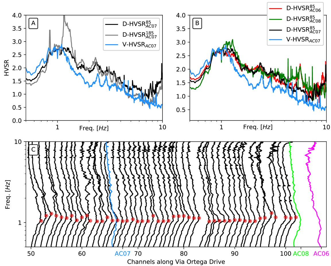
Figure 5. Comparison between DAS and velocimeter H/V spectral ratios. (a) D-HVSR computed with channels 85 and 185 and V-HVSR for station AC07. (b) Comparison between the V-HVSR at station AC07 and the D-HVSR at channel 85 computed with the vertical component of the three different velocimeters on campus. (c) All the D-HVSR computed along Via Ortega (black) along with the three V-HVSR (color). The frequency of the main D-HVSR peaks are highlighted by a red dot.
