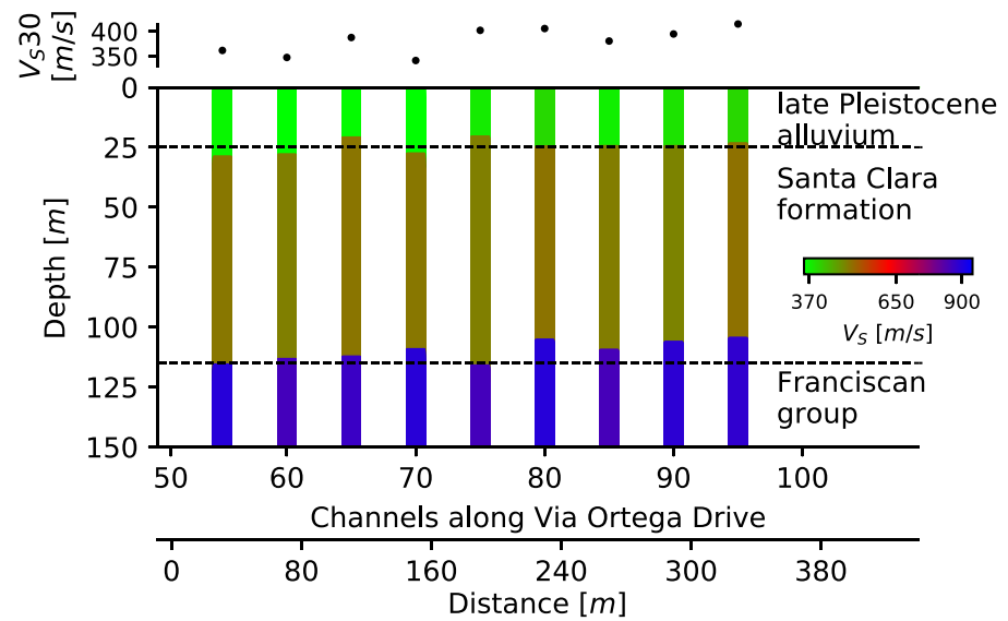
Figure 8. Joint inversion results and ground truth comparison. The black dashed lines correspond to lithological horizons as described in Thomas et al. (2014). The upper panel shows the V_{S30} estimates extracted from the joint inversion results.
