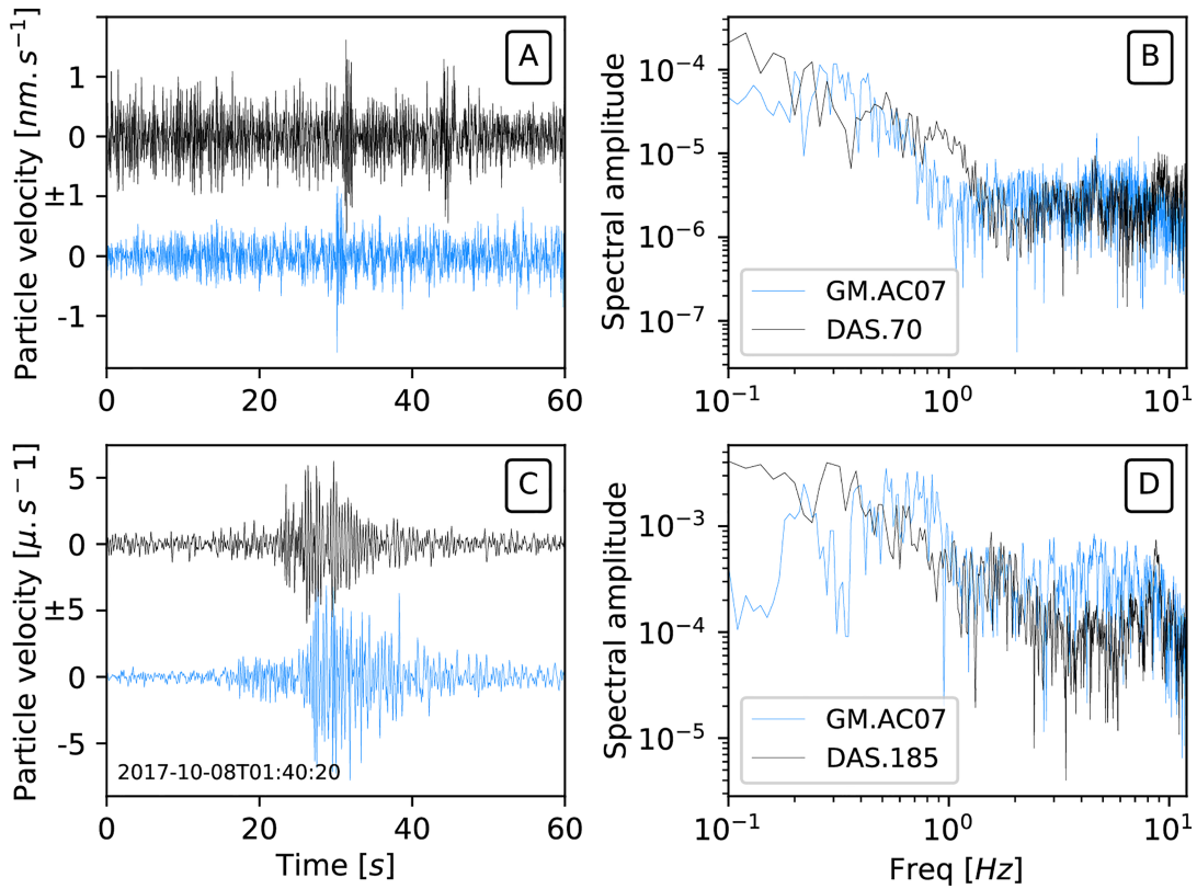
Figure 3. Velocity-converted waveforms. Velocity-converted waveforms from DAS (black) and station AC07 (blue). DAS waveforms are converted from strain to velocity using equation (1), and the geophone waveforms are corrected for instrument response and rotated according to the orientation of the DAS measurement. (a) Sixty seconds of ambient seismic field recording (with DAS channel 70), bandpass filtered between 0.8 and 8 Hz. (b) Amplitude spectra of the unfiltered waveforms shown in (a). (c) M_d 2.8 earthquake (recorded with DAS channel 185), bandpass filtered between 0.8 and 8 Hz. (d) Amplitude spectra of the unfiltered waveforms shown in (c). The velocity waveforms computed from strain are comparable in amplitude and shape to those of the velocimeter station.
