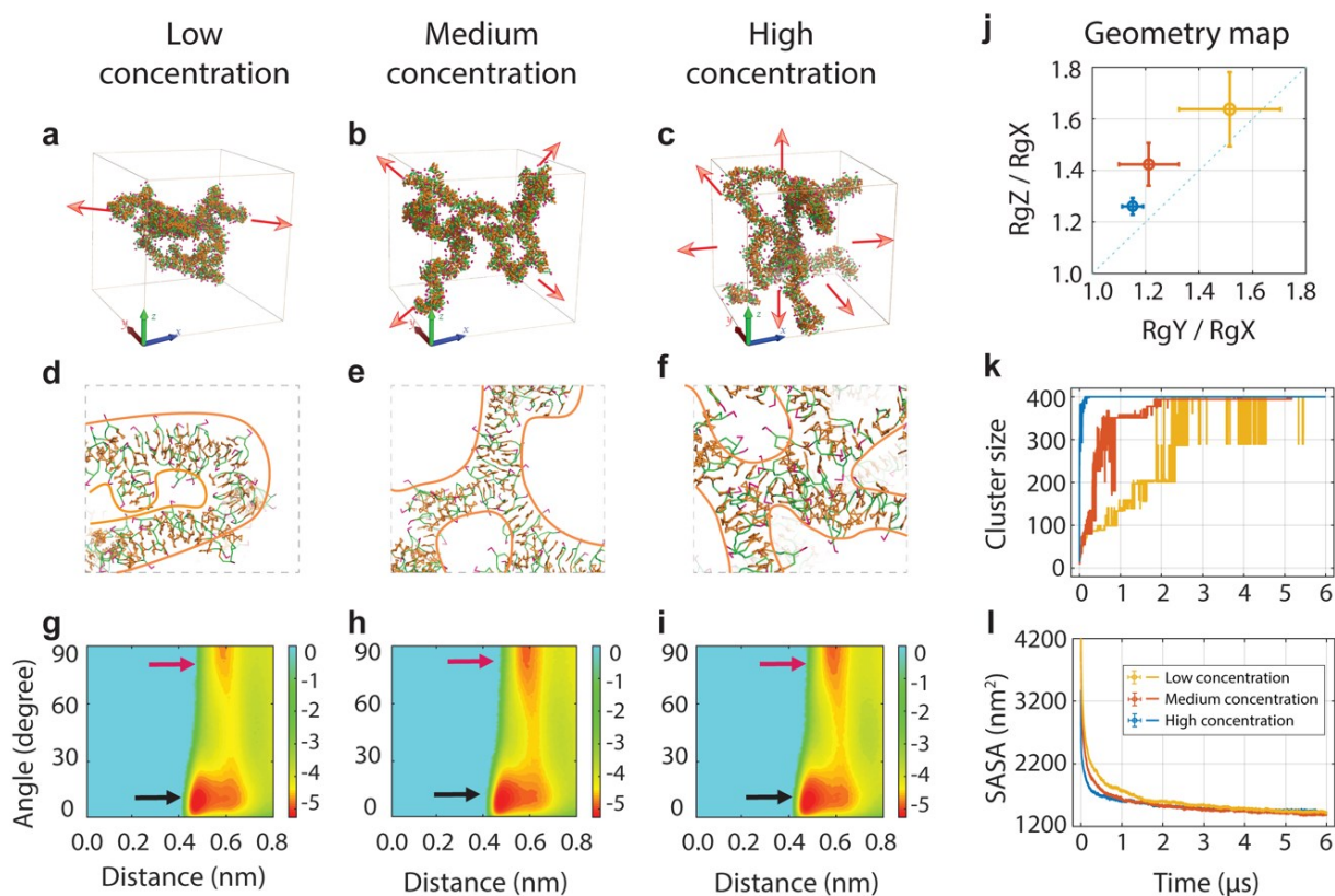
Figure 4. Analyses of structures and self-assembly pathways of Fmoc-Lys(Fmoc)-Asp hydrogels at different peptide concentrations. (a-c) Snapshots of Fmoc-Lys(Fmoc)-Asp hydrogels. (d-f) Detailed local structures of Fmoc-Lys(Fmoc)-Asp hydrogels. (g-i) The free energy landscapes of the intermolecular Fmoc stacking plotted as a function of the centroid distance and the angle between two aromatic rings. (j) Geometry map of the Fmoc-Lys(Fmoc)-Asp hydrogels formed. The dotted line indicates the diagonal of the map. (k-l) Time evolution of the size of the largest cluster (k) and the SASA of the aggregates (l).
