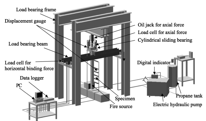
FIGURE 2 Experimental setup in Kamikawa et al 10
