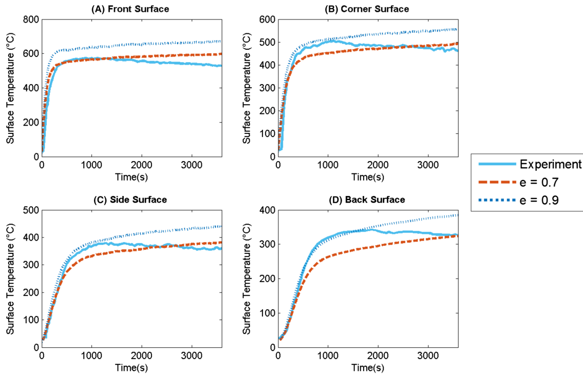
FIGURE 18 Thermal results for case 1 based on varying emissivity ( e ) assumptions: A, front surface; B, corner surface; C, side surface; D, back surface [Colour figure can be viewed at wileyonlinelibrary.com ]
