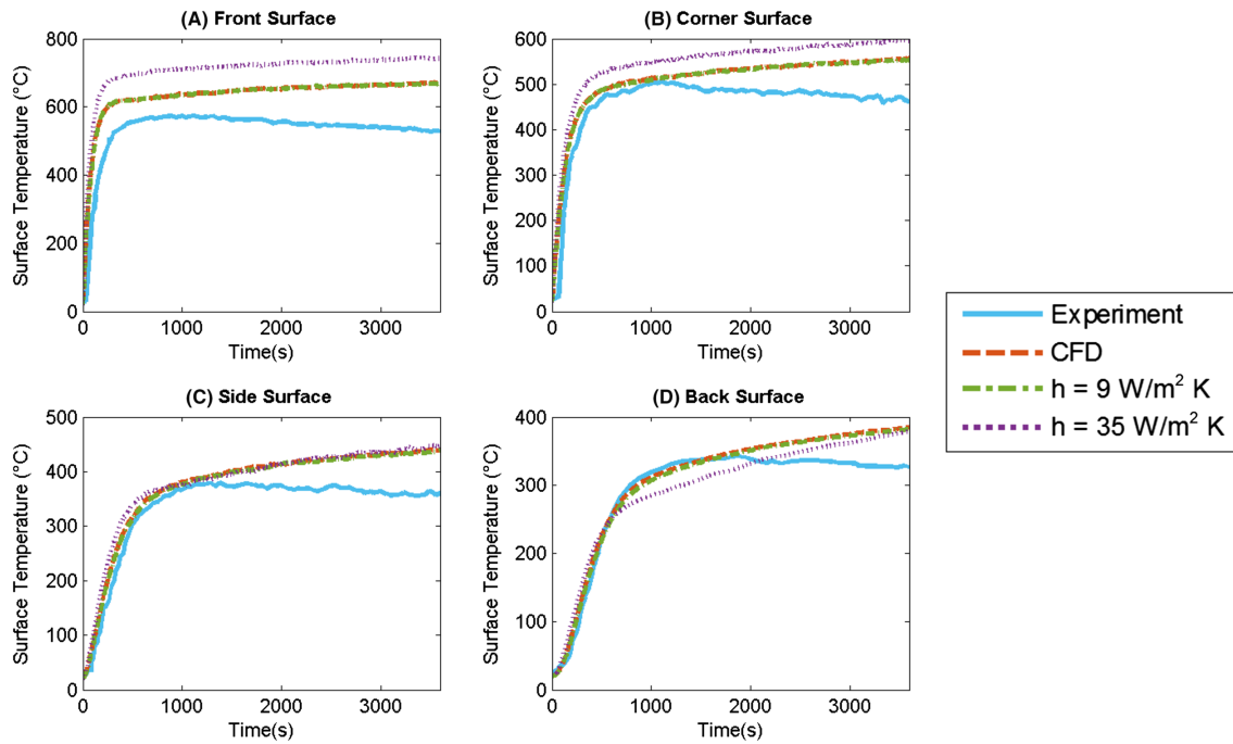
FIGURE 14 Thermal results for case 1 based on varying heat transfer coefficient ( h ) assumptions: A, front surface; B, corner surface; C, side surface; D, back surface [Colour figure can be viewed at wileyonlinelibrary.com ]
