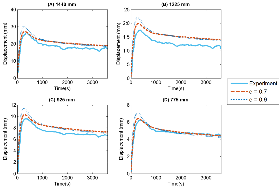
FIGURE 20 Displacement results for case 1 based on varying emissivity ( e ) assumptions: A, 1440 mm; B, 1225 mm; C, 925 mm; D, 775 mm [Colour figure can be viewed at wileyonlinelibrary.com ]
