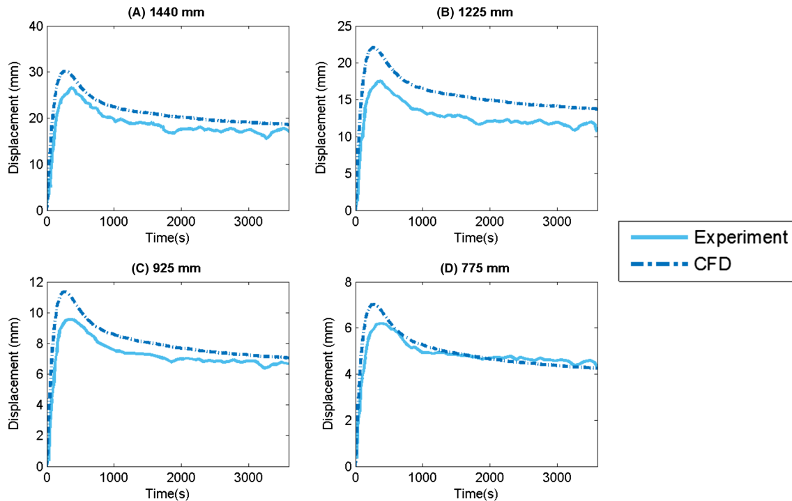
FIGURE 13 Displacement results for case 1 considering a CFD solid temperature model: A, 1440 mm; B, 1225 mm; C, 925 mm; D, 775 mm [Colour figure can be viewed at wileyonlinelibrary.com ]
