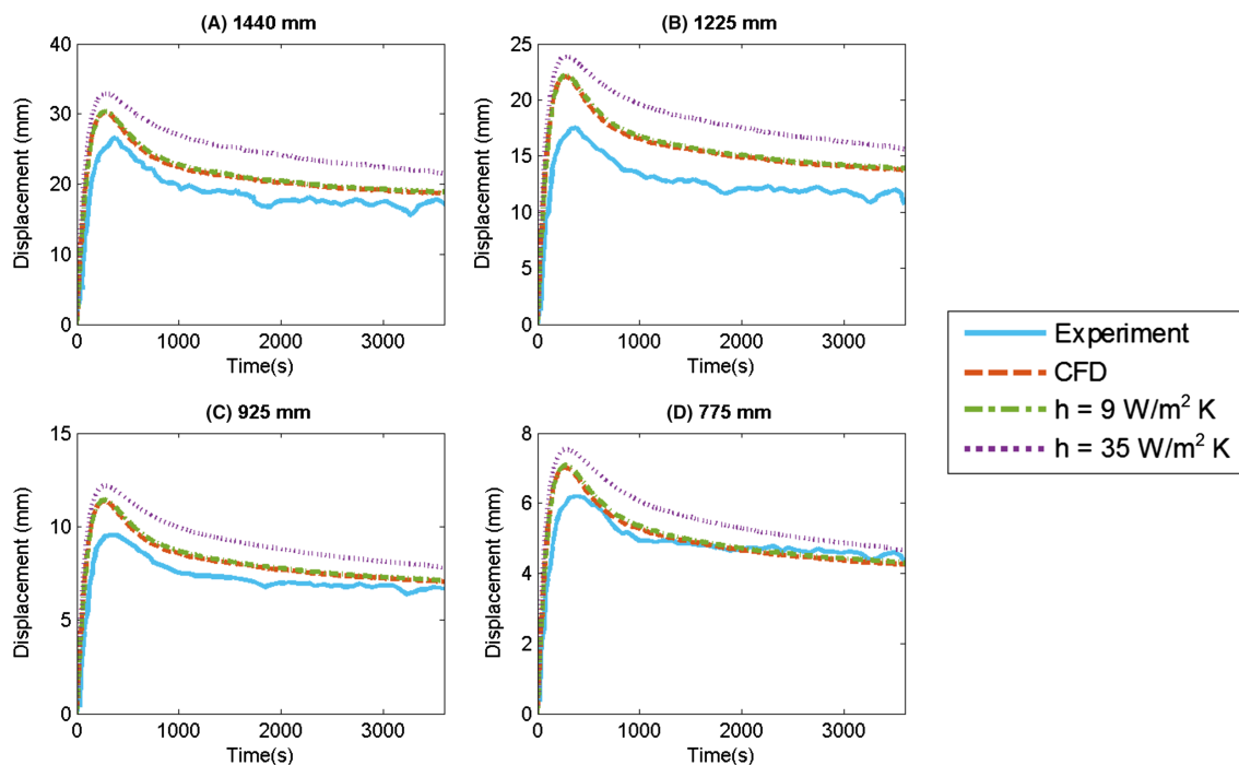
FIGURE 16 Displacement results for case 1 based on varying heat transfer coefficient ( h ) assumptions: A, 1440 mm; B, 1225 mm; C, 925 mm; D, 775 mm [Colour figure can be viewed at wileyonlinelibrary.com ]
