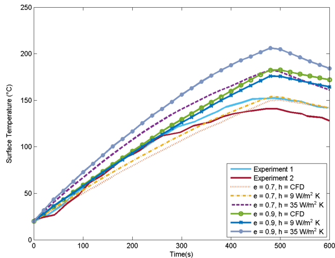
FIGURE 21 Thermal results for case 2 based on varying heat transfer coefficient ( h ) and emissivity ( e ) assumptions [Colour figure can be viewed at wileyonlinelibrary.com ]
