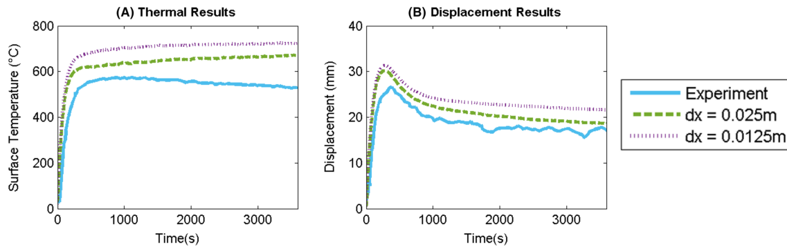
FIGURE 5 Computational fluid dynamics mesh study: A, thermal results and B, displacement results [Colour figure can be viewed at wileyonlinelibrary.com ]
