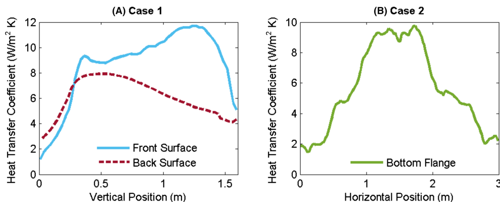
FIGURE 17 Heat transfer coefficients predicted by the CFD code: A, case 1 and B, case 2 [Colour figure can be viewed at wileyonlinelibrary.com ]
