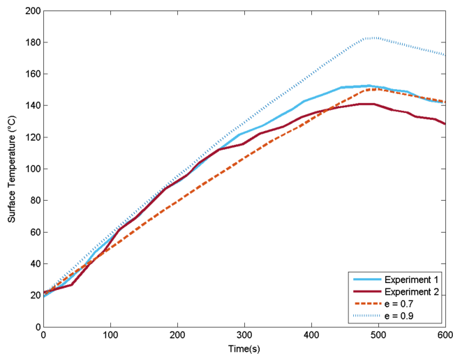
FIGURE 19 Thermal results for case 2 based on varying emissivity ( e ) assumptions [Colour figure can be viewed at wileyonlinelibrary.com ]
