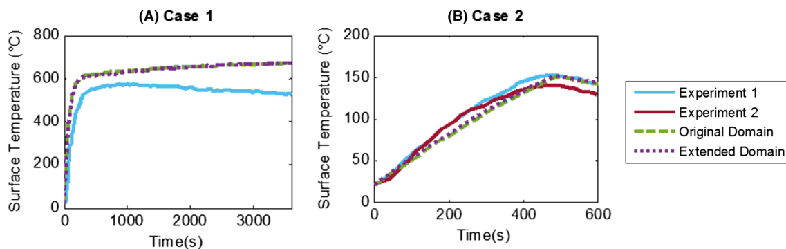
FIGURE 6 CFD computational domain comparison: A, case 1 and B, case 2 [Colour figure can be viewed at wileyonlinelibrary.com ]
