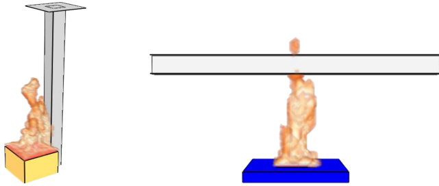
FIGURE 7 CFD simulation of A, case 1 and B, case 2 [Colour figure can be viewed at wileyonlinelibrary.com ]
