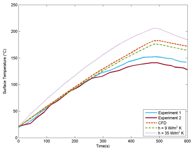
FIGURE 15 Thermal results for case 2 based on varying heat transfer coefficient ( h ) assumptions [Colour figure can be viewed at wileyonlinelibrary.com ]
