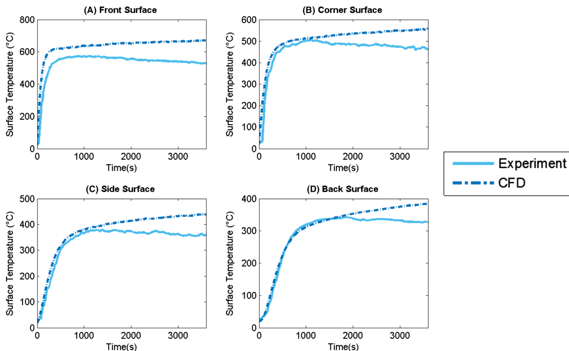
FIGURE 11 Thermal results for case 1 considering a CFD solid temperature model: A, front surface; B, corner surface; C, side surface; D, back surface [Colour figure can be viewed at wileyonlinelibrary.com ]
