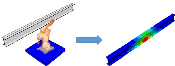
FIGURE 1 CFD-FE coupling schematic [Colour figure can be viewed at wileyonlinelibrary.com ]
