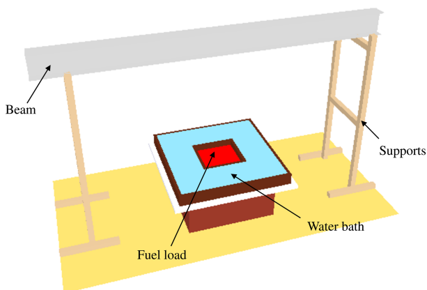
FIGURE 3 Experimental setup in Higginson et al 11 [Colour figure can be viewed at wileyonlinelibrary.com]
