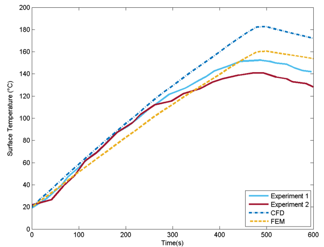
FIGURE 12 Thermal results for case 2 based on varying solid temperature models [Colour figure can be viewed at wileyonlinelibrary.com ]
