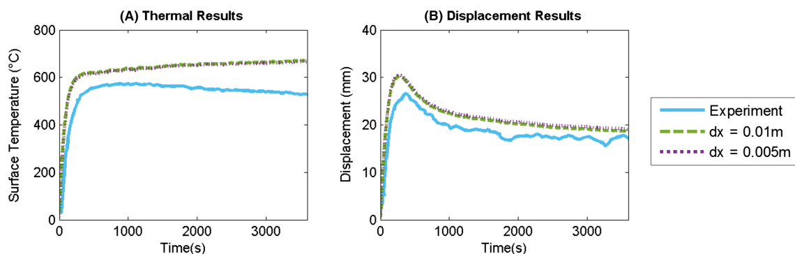
FIGURE 8 Finite element mesh sensitivity study: A, thermal results and B, displacement results [Colour figure can be viewed at wileyonlinelibrary.com ]
