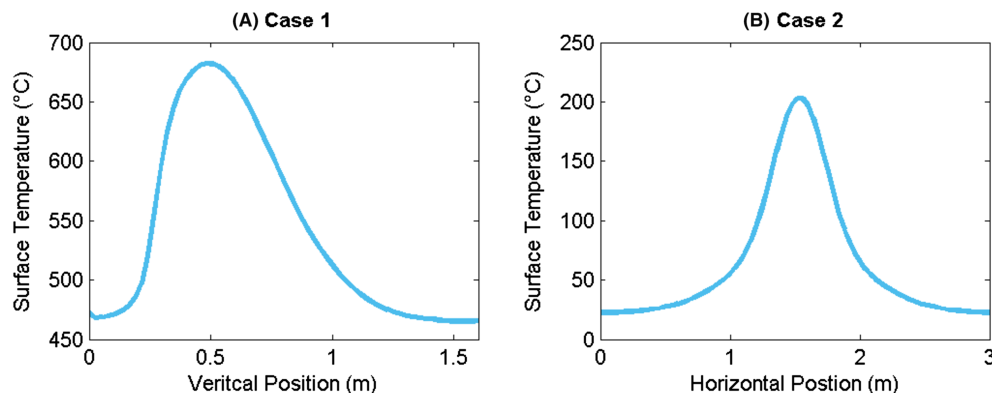
FIGURE 10 Spatially varying temperature analysis: A, case 1 and B, case 2 [Colour figure can be viewed at wileyonlinelibrary.com ]
