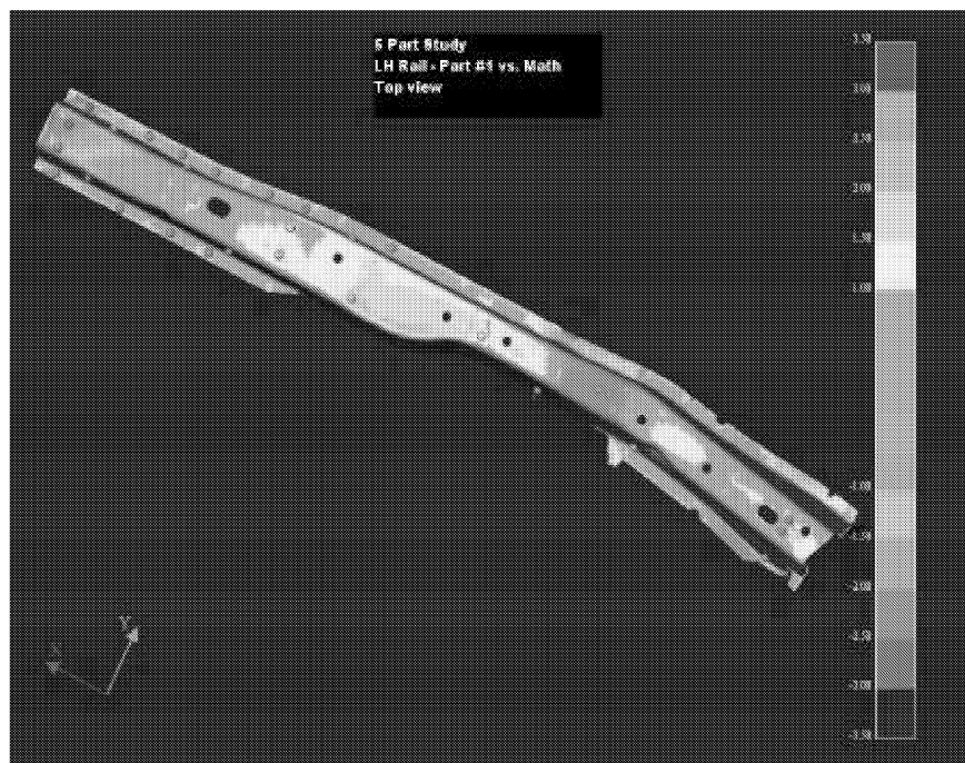
Figure 4. Measurement Results Relative to CAD Design Nominals
