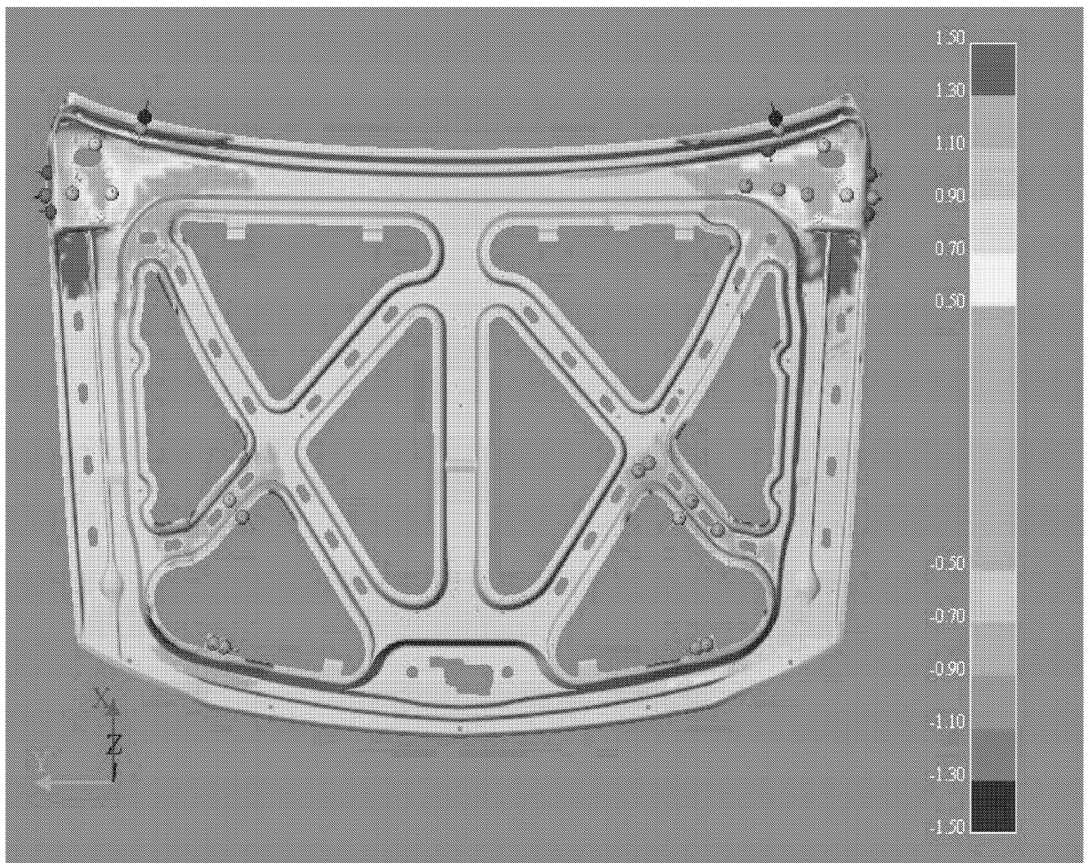
Figure 2. Sample Output from a CogniTens Optigo 200 System
