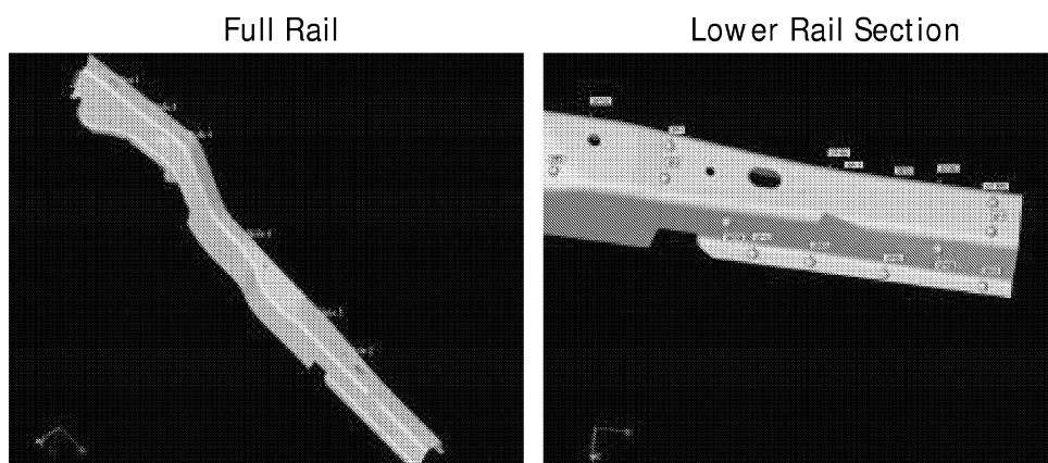
Figure 10. Rail Measurements
