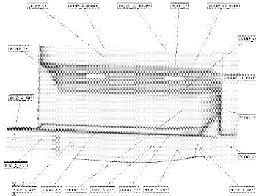
Figure 11. Structural Reinforcement Panel with Discrete Point Dimensions
