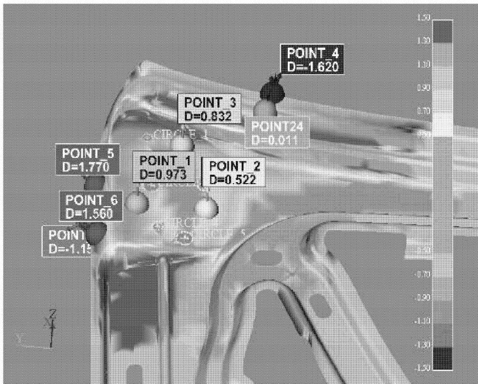
Figure 5. Hood Inner Panel Measurement Results with Discrete Points
