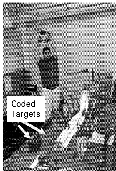
Figure 3. Measuring a Stamping Rail Panel Using Targets
