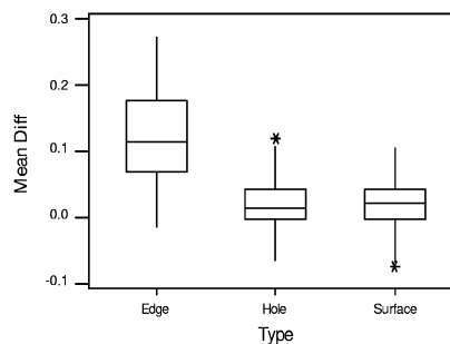
Figure 13. Mean Differences for Each Set of Panel Measurement by Feature Type
