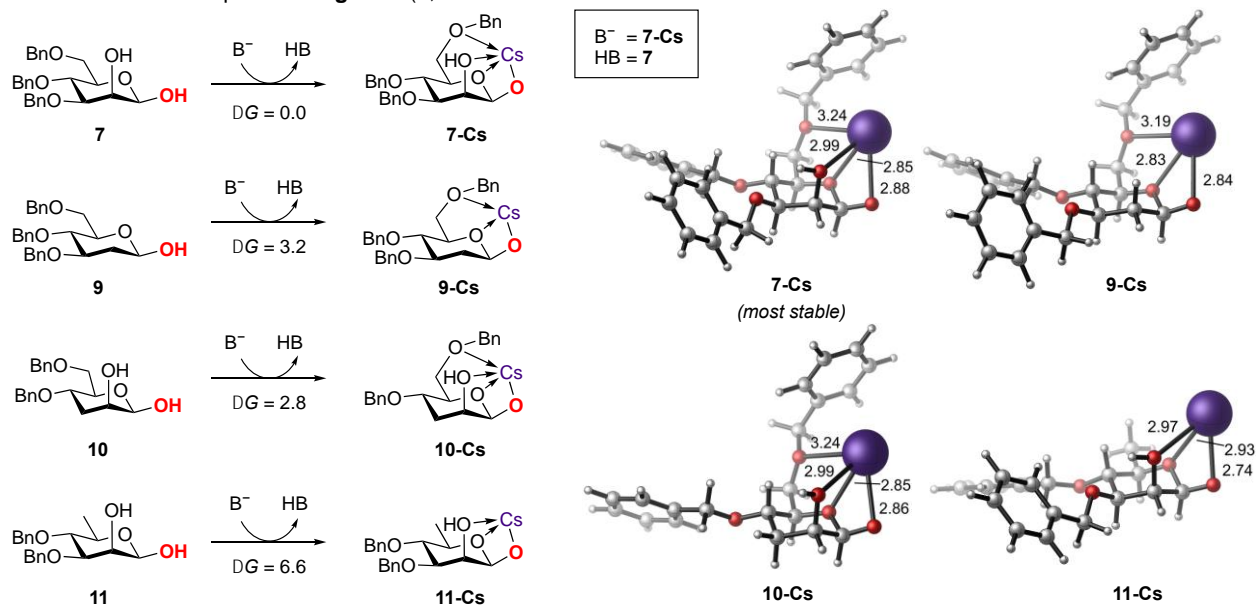
Figure 3. Relative acidity of anomeric OH of D-mannose 7 and deoxy-D-mannoses 9 , 10 , and 11 . Cesium alkoxide 7-Cs is used as the base to calculate the reaction energies of all deprotonation reactions. All energies are in kcal/mol. Bond lengths are in angstrom.
