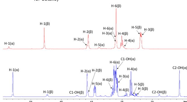
Figure 1. Comparison of ^1\text{H} NMR spectra of 3,4,6-tri- O - \text{CD}_3 - D -mannose ( 44 , \alpha/\beta = 5.2/1 , colored in blue, bottom spectrum) and its corresponding cesium alkoxide 45 ( \alpha/\beta = 1/5.0 , colored in red, top spectrum).
