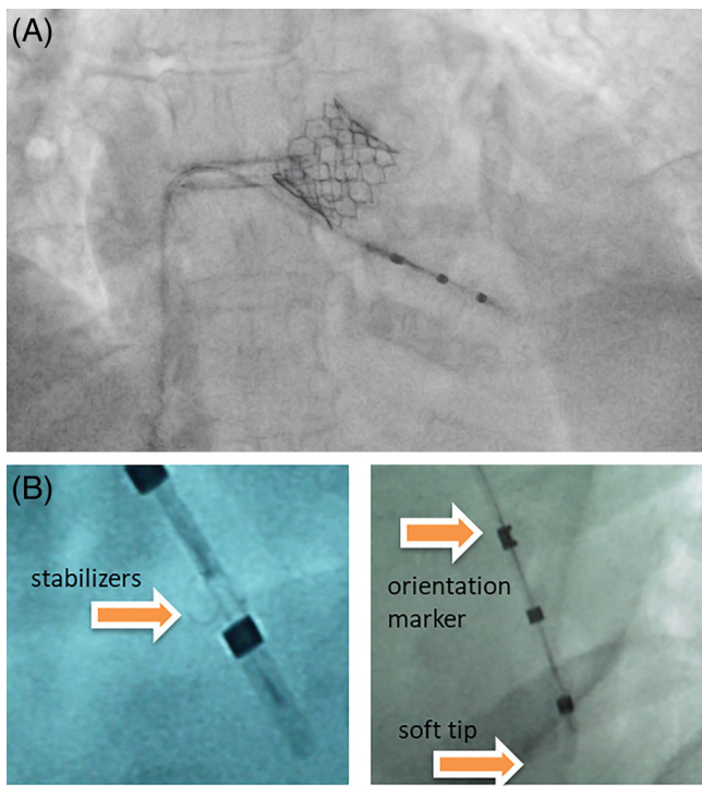
FIGURE 3 (a) Fluoroscopic view of the Tempo lead in the right ventricular apex. (b) Fluoroscopic view of the Tempo lead demonstrating the soft tip in the right ventricular apex, the orientation marker, and the deployed active fixation stabilizer loops [Color figure can be viewed at wileyonlinelibrary.com ]
