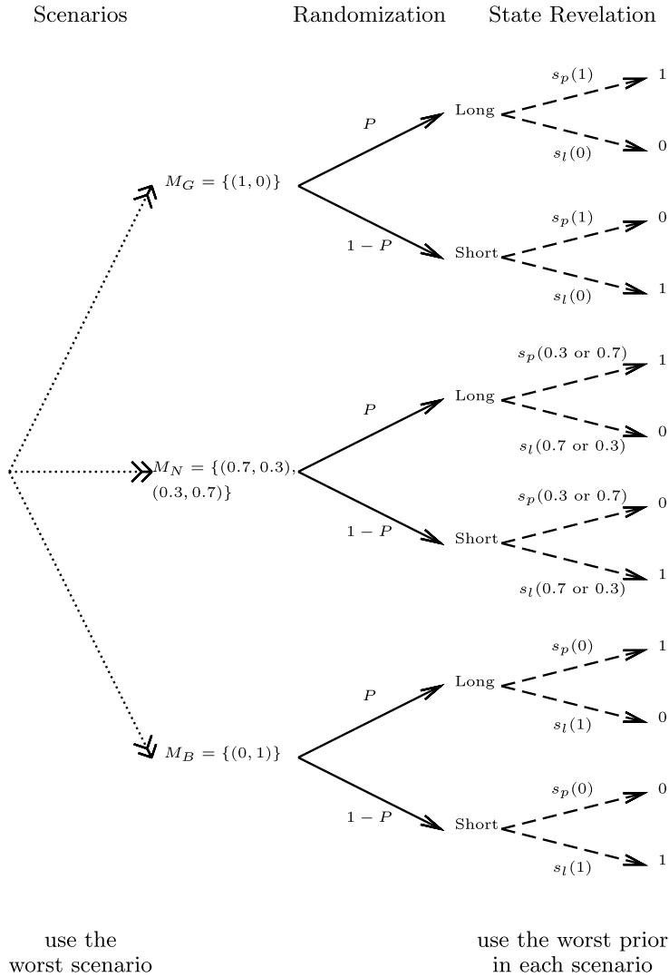
FIGURE 5.—In the good scenario M_G , the firm will profit (state s_p ) with probability 1. In the bad scenario M_B , the firm will profit with probability 0. In the neutral scenario M_N , the probability that the firm profits is either 0.3 or 0.7, which will be determined after randomization.
