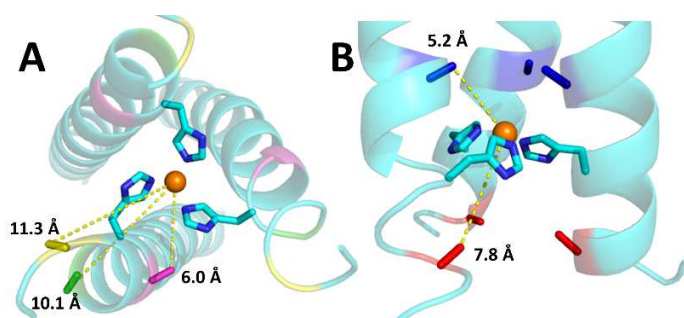
Figure 6: Model of CuNiR highlighting the location of outer sphere (A) and inner sphere (B) residue substitutions near the Cu binding site of TRI-H based on the crystal structure of \text{Zn}^{\text{II}}\text{Ni}^{\text{II}}(\text{CSL9PenL23H})_3 (PDB code 3PBJ). The copper is shown as an orange sphere, distances to the \beta -carbon of the residues being substituted are indicated for outer sphere substitutions: K22 (magenta), E24 (green) and K27 (yellow), and inner sphere: L19 (blue), and L26 (red).
