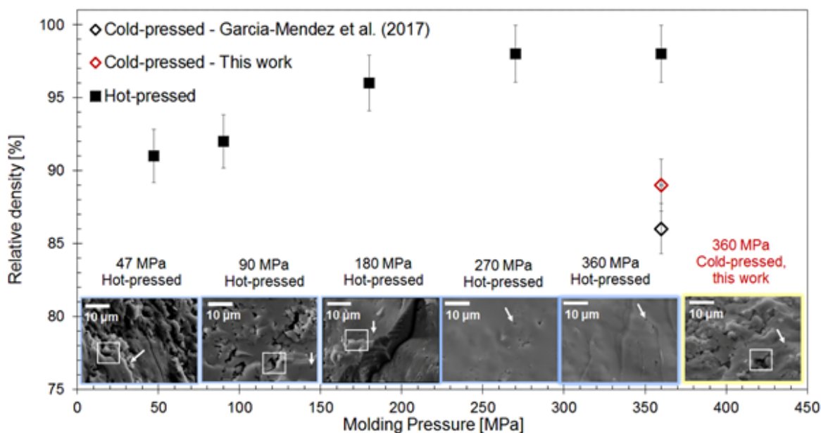
Figure 2. Relative density as a function of molding pressure of LPS 75-25 with a theoretical density of 1.88 \text{ g}\cdot\text{cm}^{-3} . Fracture surfaces and density measurements of LPS 75-25. Insets of Secondary Electron Microscope (SEM) images correspond to fracture surfaces with particle boundaries and porosity highlighted using white boxes and arrows, respectively.
