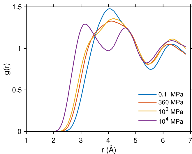
Figure S5. Calculated partial pair distribution function of Li-Li in LPS 75-25 at 25 °C for 0.1, 360, 10^3 , 10^4 MPa.
