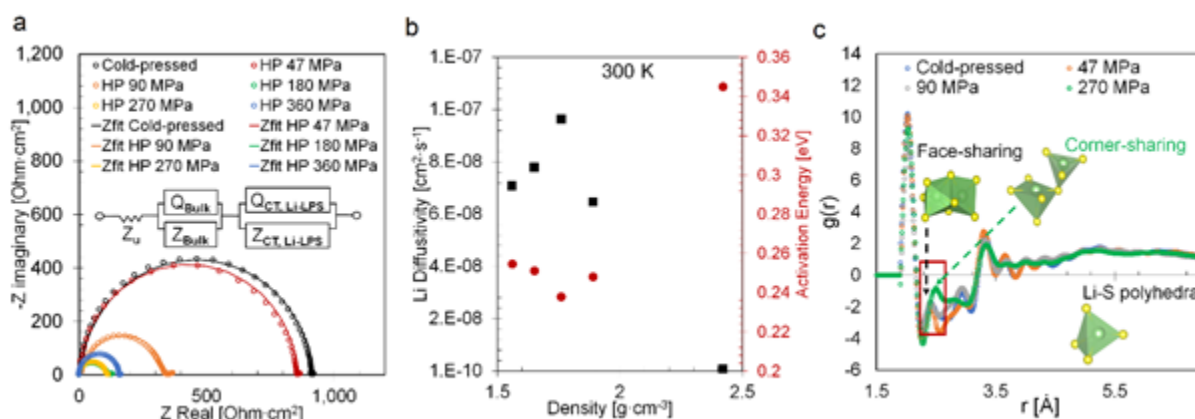
Figure 5. Measured and calculated ionic transport of LPS 75-25 (a) Electrochemical Impedance Spectroscopy (EIS) spectra of Li-LPS-Li cells at room temperature with their corresponding fit (b) Calculated lithium self-diffusivity at 300K and activation energy as a function of density. (c) Pair
