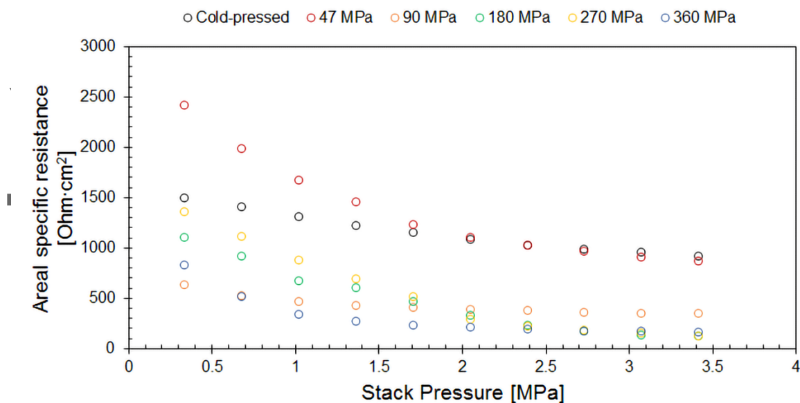
Figure S3. Effect of cell stack pressure on areal specific resistance for the bulk contribution in LPS 75-25 at room temperature
