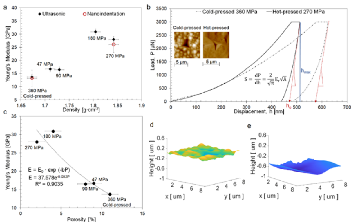
Figure 4. Elastic and plastic behavior of LPS 75-25. Young's Moduli of LPS 75-25 as a function of molding pressure via ultrasonic velocity measurements and nanoindentation (a and b). Inset in b shows the Atomic Force Microscope (AFM) 2D images acquired from cold-pressed and hot-pressed LPS at 270 MPa 200 °C. (c) Young's Moduli as a function of porosity where E_0 denotes the Young's Modulus at 0 porosity, P the volume fraction of porosity and b is a dimensionless constant. LPS Atomic Force Microscopy (AFM) 3D maps of (d) cold-pressed sample and (e) hot-pressed sample at 270 MPa, 200°C
