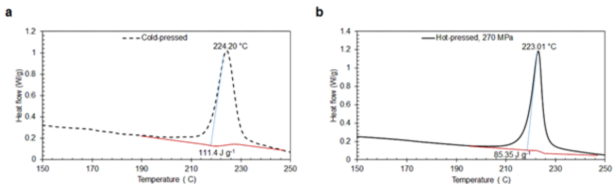
Figure S1. LPS 75-25 latent heat of crystallization of (a) cold-pressed sample (b) hot-pressed sample at 270 MPa 200°C
