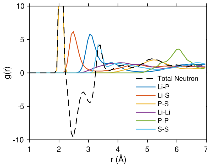
Figure S4. Local ordering of amorphous LPS 75-25 at 25 °C. Calculated partial pair distribution functions (solid lines) and total neutron weighted PDF (black dashed line).
