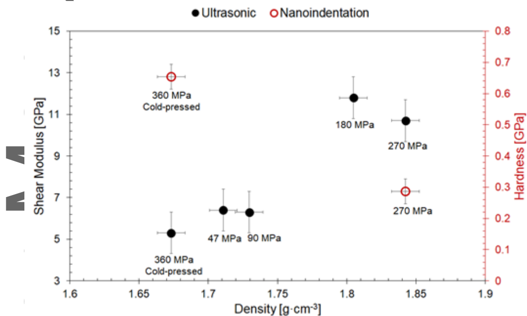
Figure S2. Shear Moduli of LPS 75-25 as a function of molding pressure via ultrasonic velocity measurements and Hardness values measured via nanoindentation
