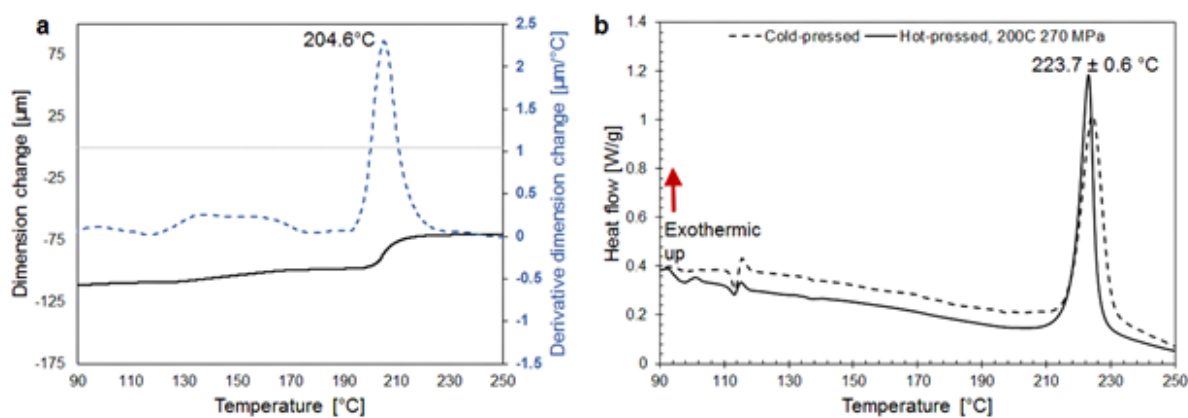
Figure 1. Measurement of glass transition and crystallization temperature for LPS 75-25 via (a) thermomechanical analysis (TMA) and (b) Differential Scanning calorimetry (DSC), respectively.
