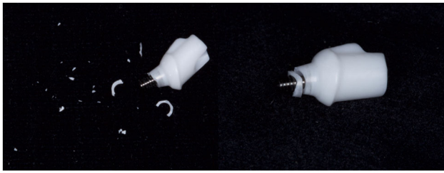
Figure 4 Representative fracture pattern of specimens.
