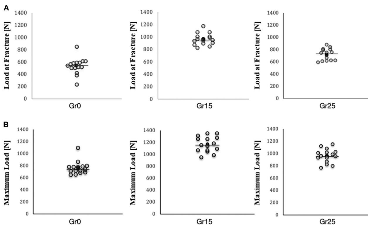
Figure 3 Scatter graphs of (A) Load at Fracture (N) (Mean; solid black dot, Observations; circles, Median; black line) and (B) Maximum Load (N) (Mean; solid black dot, Observations; circles, Median; black line) data distribution of the observations and means of the experimental groups.
