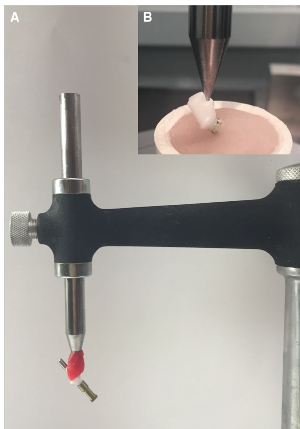
Figure 2 (A) Custom-made mounting transfer jig, and (B) the specimen positional relation to indenter.
