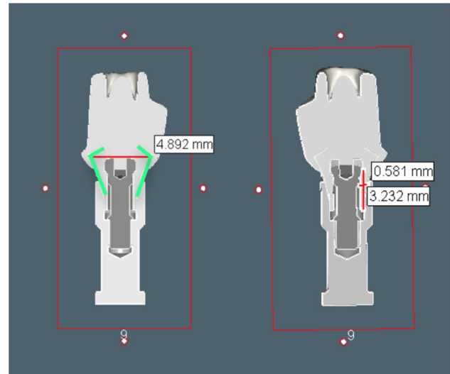
Figure 5 Digital measurements of the internal joint connection and standardized cervical dimensions using ProCera software (NobelBiocare).
