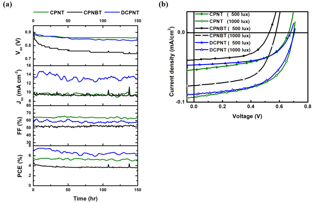
Figure 7. (a) Characteristics of CPNT-, CPNBT- and DCPNT-based devices under continuous AM 1.5G illumination in ambient room. (b) J - V characteristics of CPNT-, CPNBT- and DCPNT-based devices under illumination of TLD-840 fluorescent lamp with 500 and 1000 lux.
