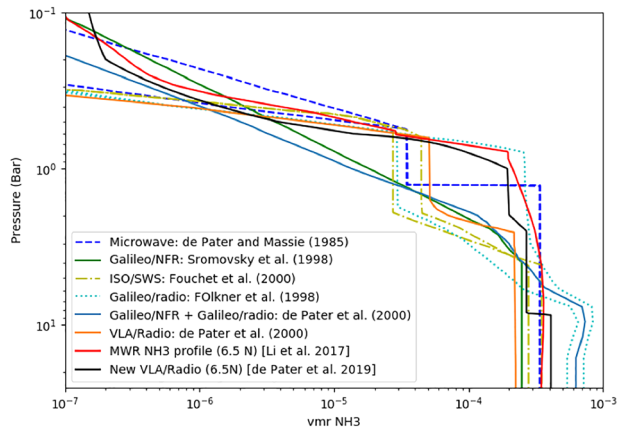
Figure 13. Ammonia abundance distribution profiles from all previous observations around 6.5^\circ N. Except for Li et al. (2017), all other ammonia profiles are considered reaching uniform deep ammonia abundance below \sim 20 bars.
