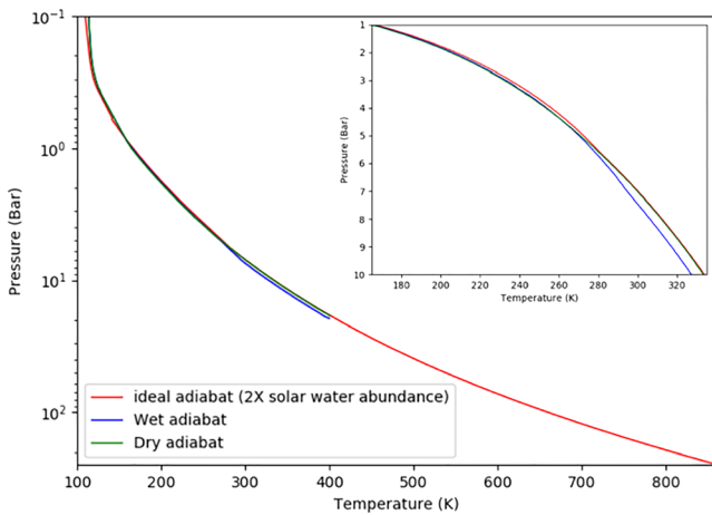
Figure 9. Temperature profiles used in the test cases. (red) Ideal adiabatic temperature profile assuming two solar water abundance in the deep atmosphere. (blue and green) Wet and dry adiabatic temperature profile proposed by de Pater et al. (2019). The inserted figure shows a blowup of these temperature pressure profiles at 1–10 bars in linear scale of pressure.
