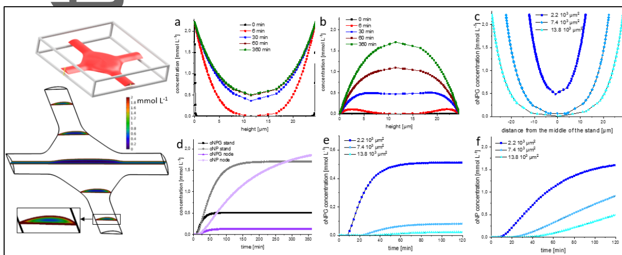
Figure 6. Simulating the diffusion of the reactant oNPG and product oNP visualizes the reactant and product distribution within the scaffold. Time dependent oNPG (a) and oNP (b) concentration over the strand height represented for a scaffold with a cross sectional area of 2.2 \cdot 10^3 \mu\text{m}^2 . c) Comparison of the oNPG concentration for different scaffold architectures after reaching steady state. Scaffold with a cross section area of 2.2 \cdot 10^3 \mu\text{m}^2 had the highest reactant concentration throughout. d) Time dependent concentration patterns in the middle of the strand and node showing of scaffold with a cross section area of 2.2 \cdot 10^3 \mu\text{m}^2 . e) The comparison of the temporal progression of the reactant for scaffolds with different architectures shows a significantly higher oNPG concentration, the smaller the cross-sectional area of the strand. The high accessibility of the reactants to enzymes results in high conversion rates and a rapid increase in the product concentration as shown in f)
