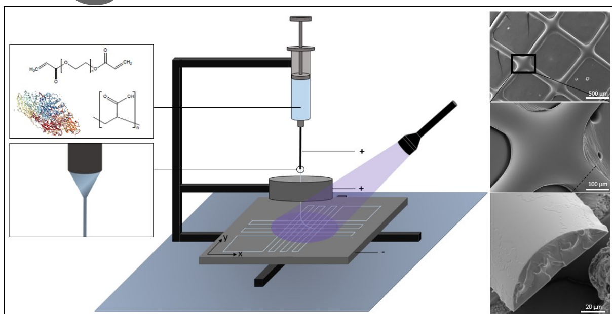
Figure 1. 3D jet writing setup for hydrogel fibers. The process allows to yield precisely oriented hydrogel fibers loaded with biological active material. Elongation of the jetting ink through an applied electric field results in 6.5 times thinner patterned filaments compared to extrusion-based printing.
