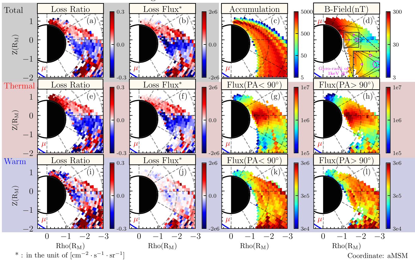
Figure 4. Loss ratio for different energy channels. (a,e,i) Normalized loss ratio for the all, thermal, and warm parts of proton; (b,f,j) the average loss flux for the three parts of proton; (c) accumulation of FIPS's measurements; (d) mean magnetic field intensity measured by MAG; and (g,h,k,l) integrated flux of thermal and warm components with pitch angle larger (less) than 90^\circ .
