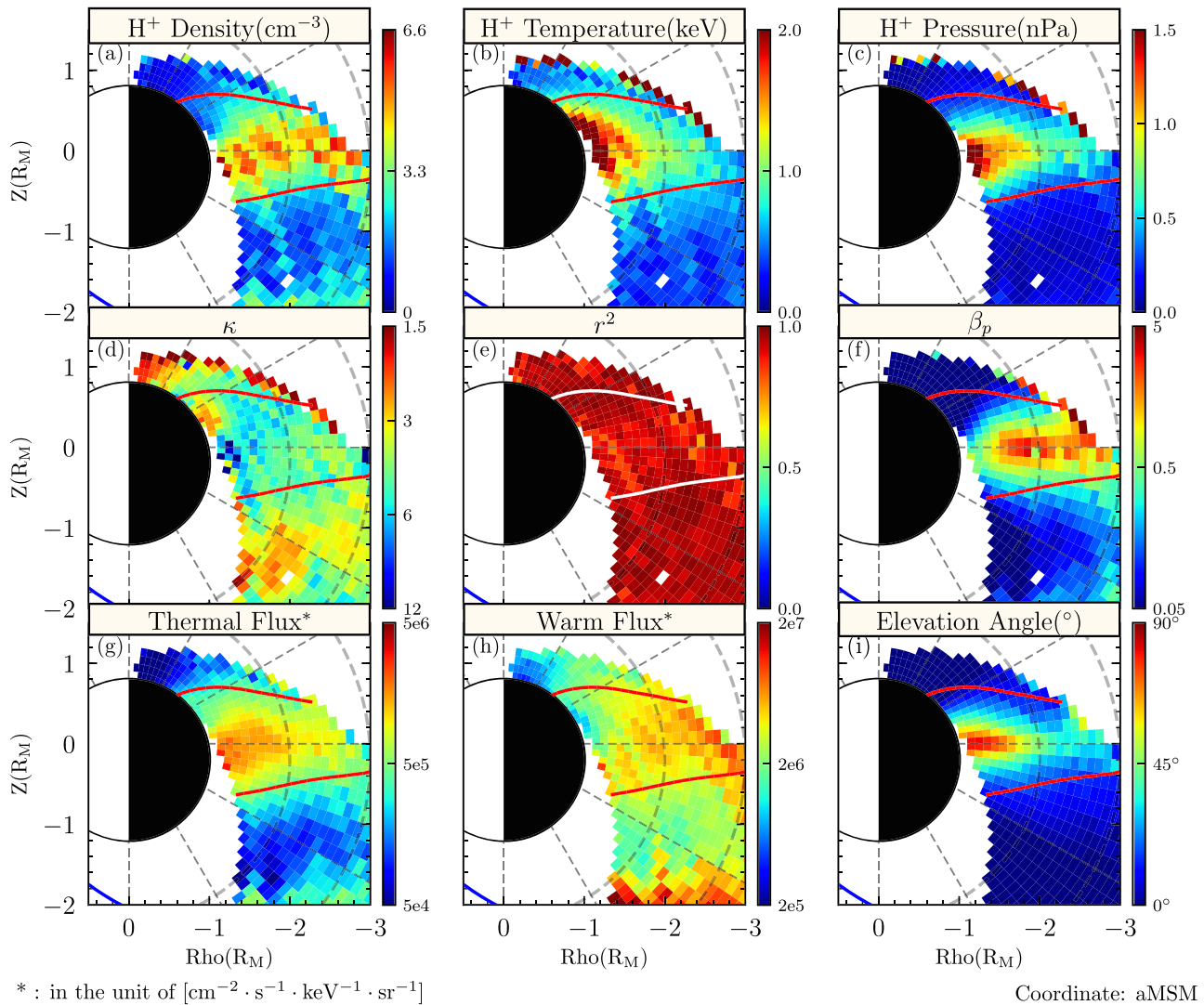
Figure 3. Same format as Figure 2 excluded the last three subplots in Figure 2.
