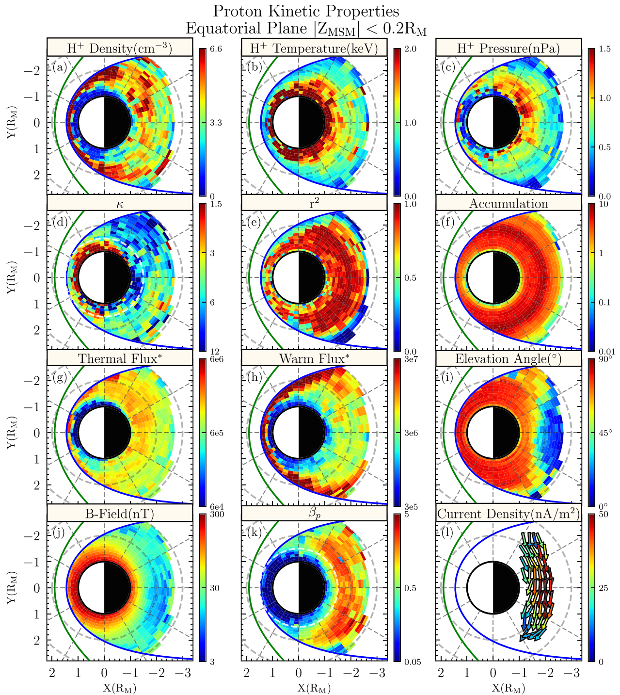
Figure 2. Proton kinetic properties in the magnetic equatorial plane with |Z| < 0.2R_M , (a–d) number density, temperature, thermal pressure, and Kappa estimated from Gaussian-Kappa model; (e) goodness of model fitting; (f) accumulations of FIPS’s measurements; (g,h) differential energy flux in the combined two energy channels; (i) elevation angle; (j) mean magnetic field measured by MAG; (k) proton beta as a ratio of fitted thermal pressure and mean magnetic pressure; and (l) current density and direction obtained from finite difference of superposed \vec{B} .
