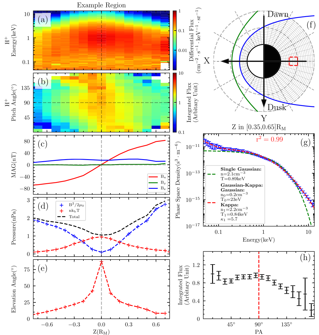
Figure 1. An example of superposed observation by FIPS (proton) and MAG. (a) Differential energy flux, (b) PAD normalized by average, (c) magnetic field, (d) pressure (magnetic and thermal), (e) elevation angle, (f) grid division schematic, (g) mean PSD at the selected regions, and (h) mean PAD normalized by maximum.
