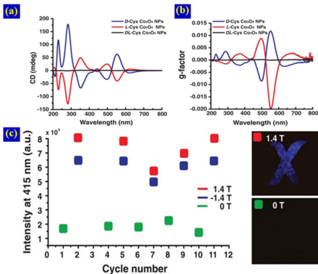
Figure 12. a) CD spectra and b) g-factor of synthesized chiral \text{Co}_3\text{O}_4 NPs. c) Cycling profile of emission intensity at 415 nm of gels with and without magnetic fields and corresponding photographs of blue-emitting light from fluorescent paper. Reproduced with permission. [22b] Copyright 2018, American Association for the Advancement of Science.
