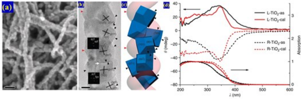
Figure 6 a) SEM image of the right-handed helical TiO 2 nanofibers. b) A HRTEM image and corresponding Fourier diffractograms of two TiO 2 nanocrystals. c) Structural model of helical stacking of anatase TiO 2 nanocrystals. d) UV-Vis and CD spectra for chiral lipid-TiO 2 hybrid (L-TiO 2 -as and R-TiO 2 -as) and double-helical TiO 2 nanofiber (L-TiO 2 -cal and R-TiO 2 -cal). Reproduced with permission. [120] Copyright 2012, Springer Nature.
