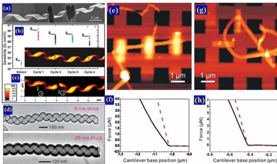
Figure 13. a) SEM image of a FIB-cut ZnO nanohelix with shape preservation. b) AFM contact-mode measurement of the sensitivity of the photodetector for the silicon substrate and the four turns of a ZnO nanohelix. c) Fracture of the nanohelix at two consecutive turns by the AFM tip, showing preservation of helical shape in the sectioned region. Reproduced with permission. [60a] Copyright 2005, American Association for the Advancement of Science. d) TEM images of helical NTs with different thicknesses. e) AFM image and f) F–D curves of a helical Al 2 O 3 NT with an outer diameter of 123 nm. g) AFM image and h) F–D curves of a helical NT with an outer diameter of 131 nm. Reproduced with permission. [57] Copyright 2010, Wiley-VCH Verlag GmbH & Co.
