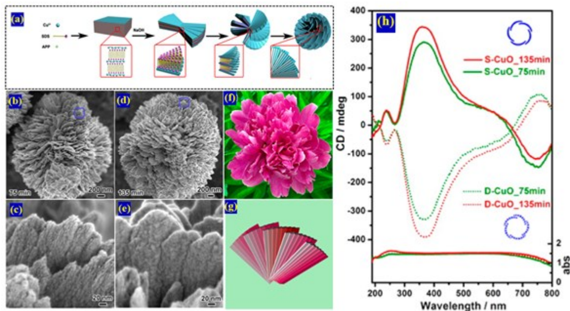
Figure 8. a) Schematic illustration for the preparation of a chiral CuO flower. SEM images and corresponding schematic drawings of sinistrorse CuO flower-like superstructures ( S -CuO) synthesized with ( S )-(–)-APP with different reaction times. b,d,f) Peony-like CuO flower-like superstructures with randomly stacked nanopetals. c,e,g) Nanoscale petals with helically arranged subnanopetals. h) Diffused reflection UV–Vis absorption and CD spectra of the antipodal chiral CuO flower-like superstructures. Reproduced with permission. [88] Copyright 2014, American Chemical Society.
