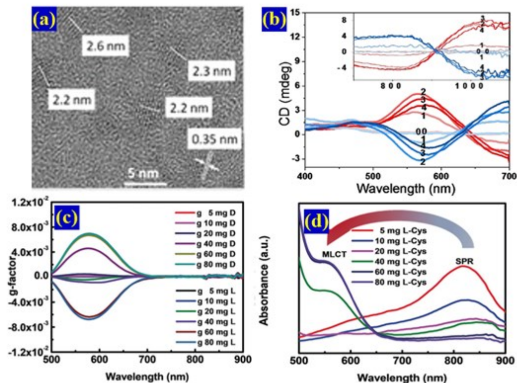
Figure 9. a) HRTEM image for l -Asp-capped \text{WO}_{3-x} NPs. b) CD spectra of l -Asp-capped \text{WO}_{3-x} NPs (red) and d -Asp-capped \text{WO}_{3-x} NPs (blue) (inset: NIR range of corresponding CD spectra). c) g -factor spectra of chiral molybdenum oxide NPs with different amounts of l - or d -cysteine. Reproduced with permission. [39] Copyright 2018 Wiley-VCH Verlag GmbH & Co. KGaA, Weinheim. d) Absorption spectra of l -cysteine-capped molybdenum oxide NPs. Reproduced with permission. [39] Copyright 2018 Wiley-VCH Verlag GmbH & Co. KGaA, Weinheim.
