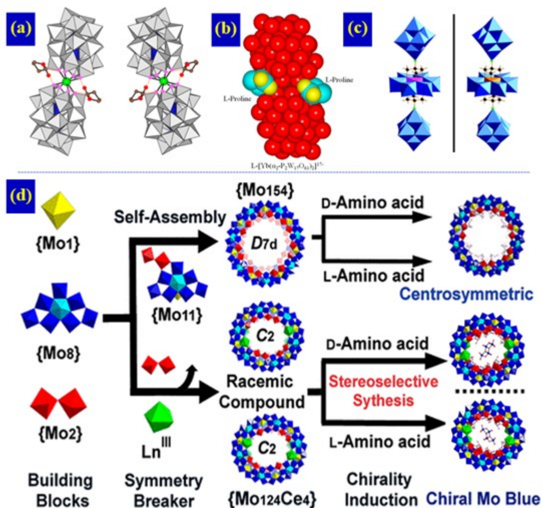
Figure 10. a) Combined polyhedral and ball-and-stick representation of two enantiomers of the [\text{Ln}(\alpha_2\text{-P}_2\text{W}_{17}\text{O}_{61})_2]^{17-} polyanion ( l -form; left, d -form; right). b) Space-filling model of the association composed of l\text{-}[\text{Yb}(\alpha_2\text{-P}_2\text{W}_{17}\text{O}_{61})_2]^{17-} and two l -Pro molecules. Reproduced with permission. [140] Copyright 2018, American Chemical Society. c) Combined polyhedral and ball-and-stick representation of noncovalently assembled chiral rod-like molecular triads of [\text{Mo}_6\text{O}_{18}\text{NC}(\text{OCH}_2)_3\text{MMo}_6\text{O}_{18}(\text{OCH}_2)_3\text{CNMo}_6\text{O}_{18}]^{7-} , metals are \text{Mn}^{\text{III}} (left) and \text{Fe}^{\text{III}} (right). Reproduced with permission. [146] Copyright 2009, American Chemical Society. d) Stereoselective synthesis of chiral Mo blue POM clusters with "symmetry breaker". Reproduced with permission. [149] Copyright 2019, American Chemical Society.
