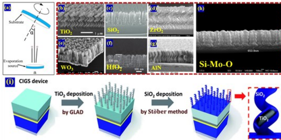
Figure 2. a) Schematic of the GLAD deposition. Reproduced with permission. [70d] Copyright 2015, Elsevier Ltd. Cross-sectional SEM images of b) a helical \text{TiO}_2 thin film. Reproduced with permission. [73] Copyright 2015, Elsevier Ltd. c) A random array of \text{SiO}_2 helices growing at the ratio of the substrate rotation rate to the deposition rate: 22.7 \text{ nm rad}^{-1} . Reproduced with permission. [73] Copyright 2012, Elsevier Ltd. d) Nanostructured \text{ZrO}_2 films (substrate rotational speed: 0.14 rpm). Reproduced with permission. [75] Copyright 2012, Springer-Verlag. e) Pillar-type structures of \text{WO}_3 film onto W/Si substrate. Reproduced with permission. [76] Copyright 2007, Elsevier Ltd. f) A \text{HfO}_2 sample with four spirals per column. Reproduced with permission. [77] Copyright 2007, Chinese Physical Society and IOP Publishing Ltd. g) \text{AlN} nanorod structures at helical depositions. Reproduced with permission. [78] Copyright 2012, Lung-Chien Chen et al. h) the helical-shaped Si-Mo-O films. Reproduced with permission. [81] Copyright 2019, Springer Nature B.V. i) Schematic diagram of preparing \text{TiO}_2 - \text{SiO}_2 core-shell helical nanostructured coatings on \text{Cu(In,Ga)Se}_2 . Reproduced with permission. [82] Copyright 2019, Royal Society of Chemistry.
