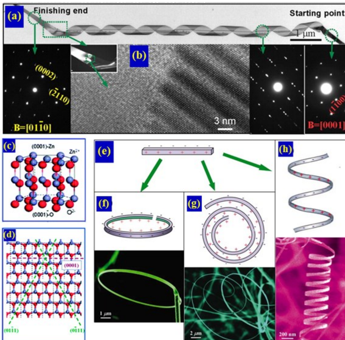
Figure 7. a) Low-magnification TEM image of a helical ZnO nanobelt with three typical SAED patterns of different regions. b) HRTEM image of a local area of the helical ZnO nanobelt. Reproduced with permission. [60a] Copyright 2005, American Association for the Advancement of Science. c,d) Wurtzite structure model of ZnO showing the \pm(0001) polar surfaces. Reproduced with permission. [60b] Copyright 2004, Elsevier Ltd. e–h) Polar-surface-induced formation of nanorings, nanospirals, and nanohelices of ZnO and their formation processes. Reproduced with permission. [127c] Copyright 2004, Elsevier Ltd.
