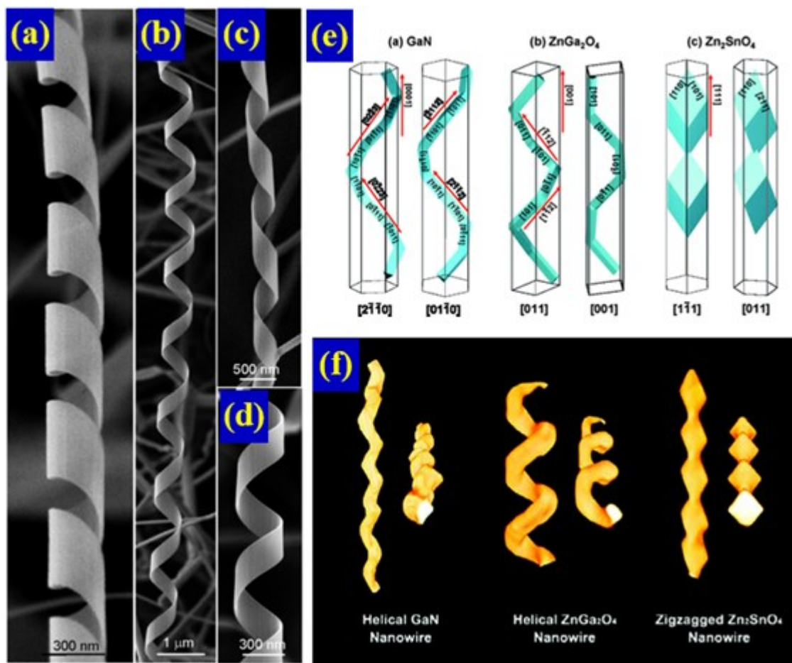
Figure 1. a–d) Typical SEM images of helical ZnO nanobelts. Reproduced with permission. [60a] Copyright 2005, American Association for the Advancement of Science. e) Schematic model constructed for helical GaN and ZnGa 2 O 4 NWs and zigzagged Zn 2 SnO 4 NWs. Reproduced with permission. [69] Copyright 2008, American Chemical Society. f) Images of the helical GaN ZnGa 2 O 4 Zn 2 SnO 4 NW obtained through tomographic 3D reconstruction. Reproduced with permission. [69] Copyright 2008, American Chemical Society.
