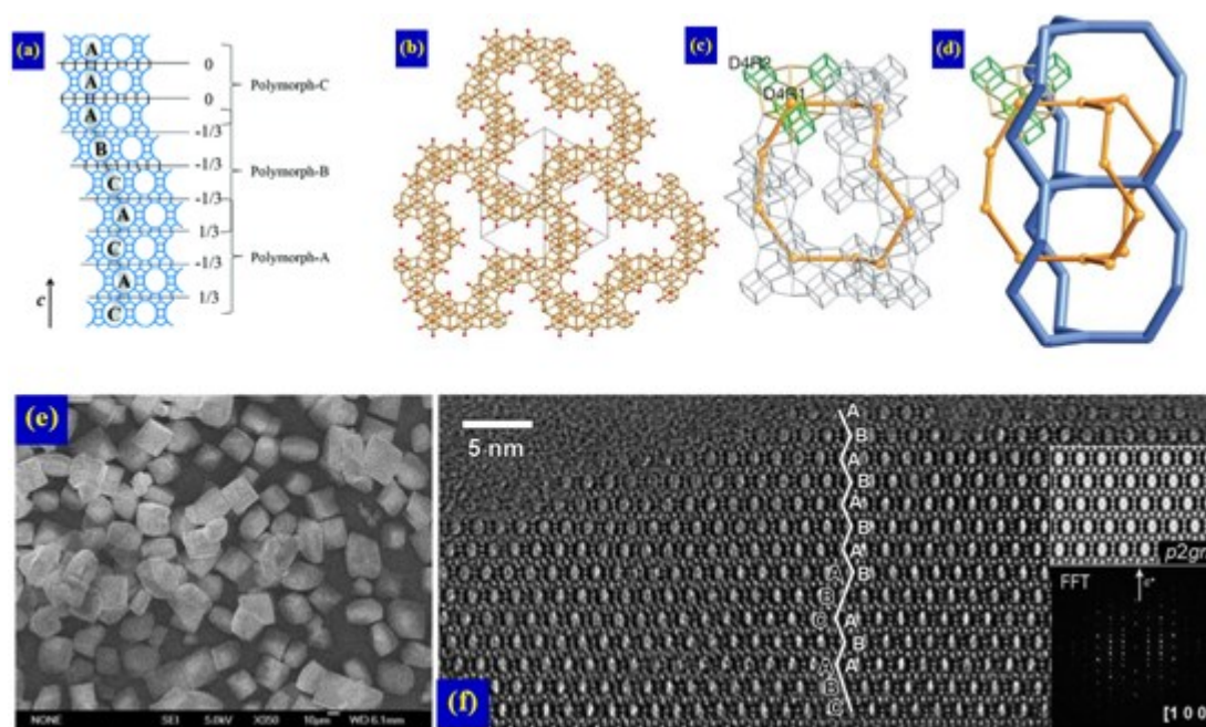
Figure 11. a) (010)-projection of intergrowth structure of \beta -zeolite. Reproduced with permission. [156] Copyright 2019, The Royal Society of Chemistry. The framework and corresponding nets of germanosilicate mesoporous chiral zeolite. b) a slice (15.3 Å thick) viewed down the (111) direction. Double 4-rings are composed of one (D4R1) or two (D4R2) terminal hydroxyl groups. c) The 30-ring built from ten tertiary building units, where each unit is linked to three neighboring units. d) The large cavity defined by three 30-rings. Reproduced with permission. [152] Copyright 2009, Springer Nature. e) SEM image of \beta -tetraethylammonium hydroxide. f) HRTEM image of the beta-tetraethylammonium hydroxide crystal. Reproduced with permission. [156] Copyright 2015, 2018 Springer Nature.
