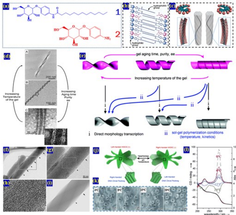
Figure 5 a) Chemical structures of gelators 1 and 2. b) A possible self-assembling model for bi-layered chiral fiber. Reproduced with permission. [100] Copyright 2002, American Chemical Society. c) Molecular origin of chiral mesoporous silica derived from the helical packing of chiral amphiphiles. Reproduced with permission. [107] Copyright 2008, American Chemical Society. d) TEM images of A) twisted ribbon and B) helical ribbons. C) Tubules self-assembled from CTA with tartrate. Reproduced with permission. [103] Copyright 2008, American Chemical Society. e) Schematic representation of the diversity of inorganic silica chiral ribbons. Reproduced with permission. [103] Copyright 2008, American Chemical Society. f–h) TEM images for chiral mesoporous silicas with hexagonally ordered chiral channels. i) A simulated TEM image shows two types of fringes. Reproduced with permission. [52d] Copyright 2004, Nature Publishing Group. j) Illustration of the macroscopic enantiomeric helical morphologies and corresponding opposite DNA chiral packing of impeller-like helical DNA–silica complexes. Reproduced with permission. [113] Copyright 2012, WILEY-VCH Verlag GmbH & Co. KGaA, Weinheim. k) SEM images for the IHSDCs obtained from different temperatures (left-handed: + ; right-handed: –). Reproduced with permission. [113] Copyright 2012, WILEY-VCH Verlag GmbH & Co. KGaA, Weinheim. l) CD and UV–Vis spectra for the IHSDCs obtained from different temperatures. Reproduced with permission. [113] Copyright 2012, WILEY-VCH Verlag GmbH & Co. KGaA, Weinheim.
