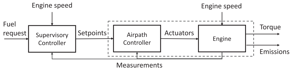
FIGURE 3 A high-level control architecture diagram
