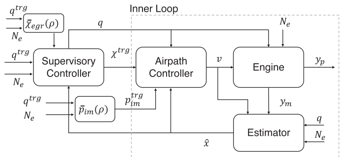
FIGURE 7 A schematic of the MPC control architecture; see Section 1.2 for notation. In this article the supervisory controller is a supervisory MPC (SMPC) controller and the airpath or inner-loop controller is a nonlinear MPC (NMPC) controller
