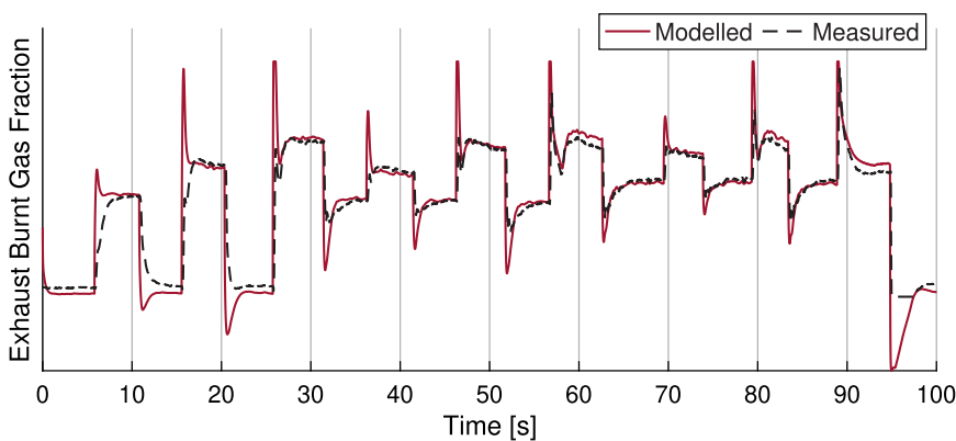
FIGURE 6 Comparison of the burnt gas fraction model against experimental data obtained from a wideband oxygen concentration sensor downstream of the VGT. The model is in good agreement with the measurements; the placement of the sensor induces a filtering effect which accounts for the error in transients [Colour figure can be viewed at wileyonlinelibrary.com ]
