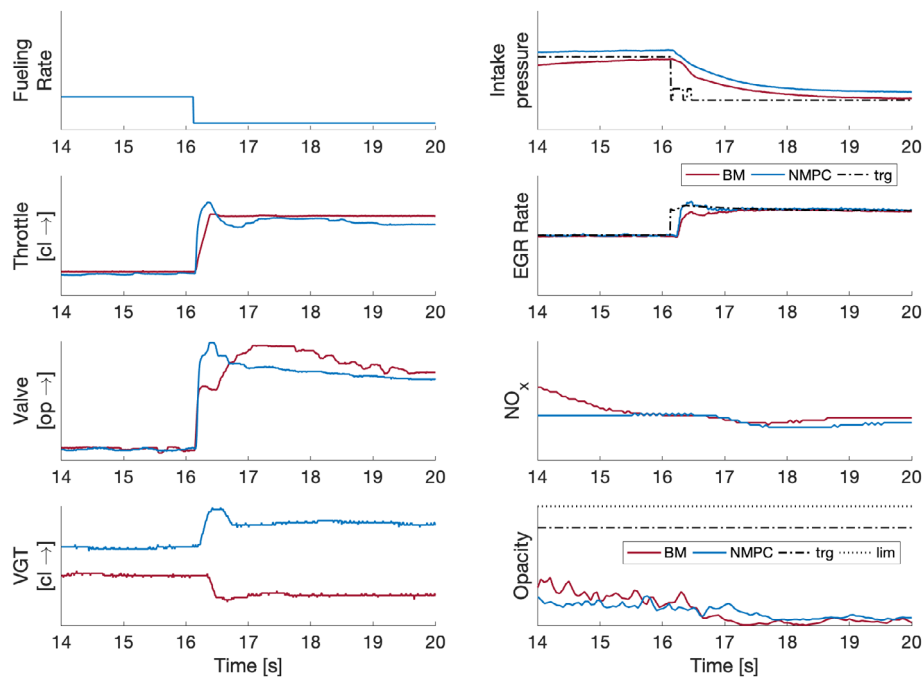
FIGURE 12 A comparison between the benchmark (BM) and NMPC controllers during a fuel step-down maneuver at a constant engine speed. The NMPC controller more closely tracks EGR rate leading to reduced \text{NO}_x production. The y-axis scales have been removed to preserve data confidentiality [Colour figure can be viewed at wileyonlinelibrary.com ]
