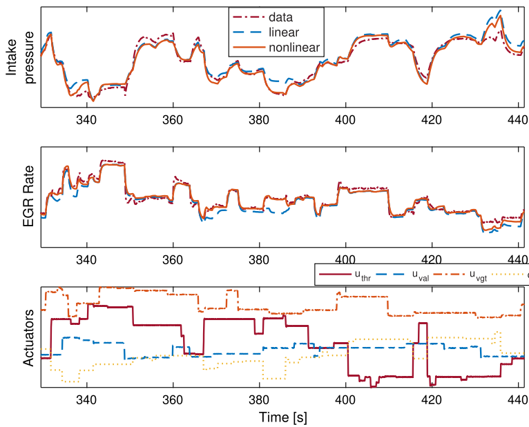
FIGURE 4 Validation of the nonlinear open-loop airpath model at 1800 rpm. The model output matches the validation data well and the inclusion of the nonlinear terms improves overall accuracy [Colour figure can be viewed at wileyonlinelibrary.com ]
