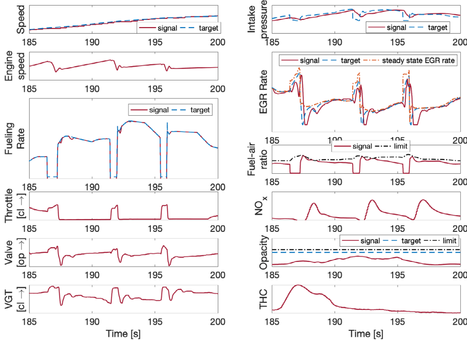
FIGURE 19 A close-up of an acceleration event with the MPC controller in closed loop with the engine during the WLTC. During the tip ins following the gearshifts the supervisory layer commands the NMPC controller to quickly reduce the EGR rate and limits the fuel to satisfy the fuel-air ratio constraint, preventing visible smoke. The inner loop relies on its feedforward module to track the aggressive commands from the supervisory layer, leading to a very fast EGR rate response which minimizes fuel limiting and NO x production. The y-axes scales have been removed to preserve data confidentiality [Colour figure can be viewed at wileyonlinelibrary.com ]
