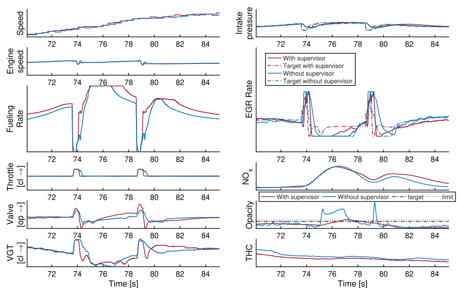
FIGURE 18 A comparison between the MPC controller with and without the supervisory controller. Without the supervisor large amounts of visible smoke is produced; the opacity limit is where the smoke becomes visible. The enforcement of the smoke constraint leads to a torque delay which is undesirable but necessary to prevent excessive smoke. Minimization of this torque delay is part of the SMPC formulation via the fuel tracking term. The y-axes scales have been removed to preserve data confidentiality [Colour figure can be viewed at wileyonlinelibrary.com ]
