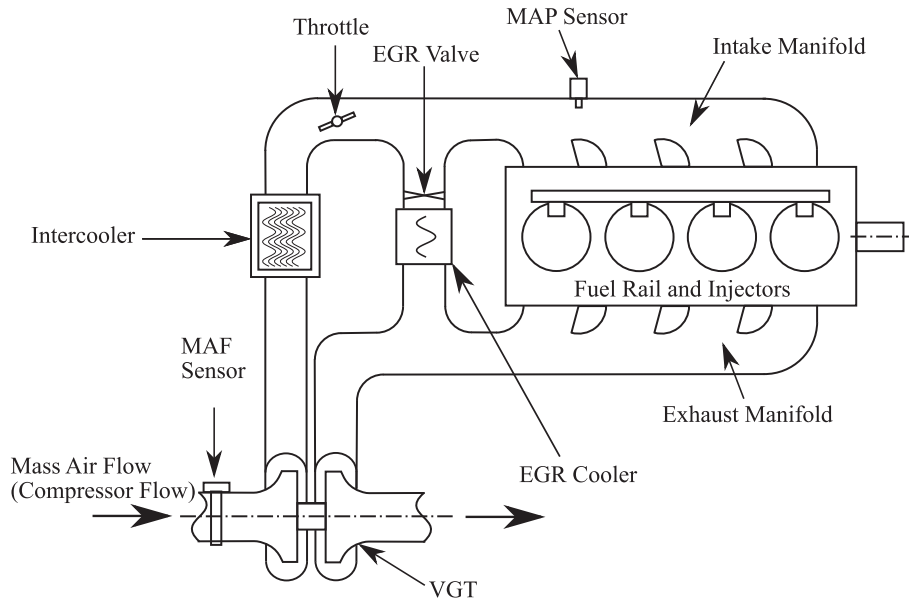
FIGURE 2 A diagram of the diesel engine airpath
