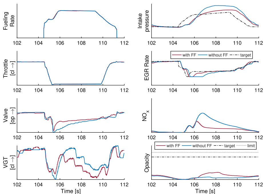
FIGURE 13 A comparison between the NMPC airpath controller with and without the NMPC feedforward module at a constant engine speed. The feedforward module improves EGR rate tracking leading to reduced \text{NO}_x emissions. The y-axis scales have been removed to preserve data confidentiality [Colour figure can be viewed at wileyonlinelibrary.com ]
