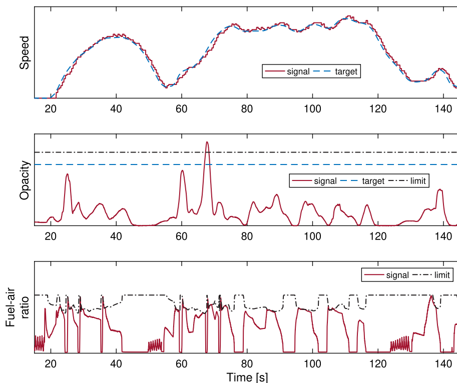
FIGURE 16 A portion of the WLTC with the MPC controller in closed loop with the engine. The vehicle was able to successfully complete the drivecycle despite some fuel limiting. The smoke is well controlled with only a few spikes reaching the edge of the visible range. The y-axes scales have been removed to preserve data confidentiality [Colour figure can be viewed at wileyonlinelibrary.com ]
