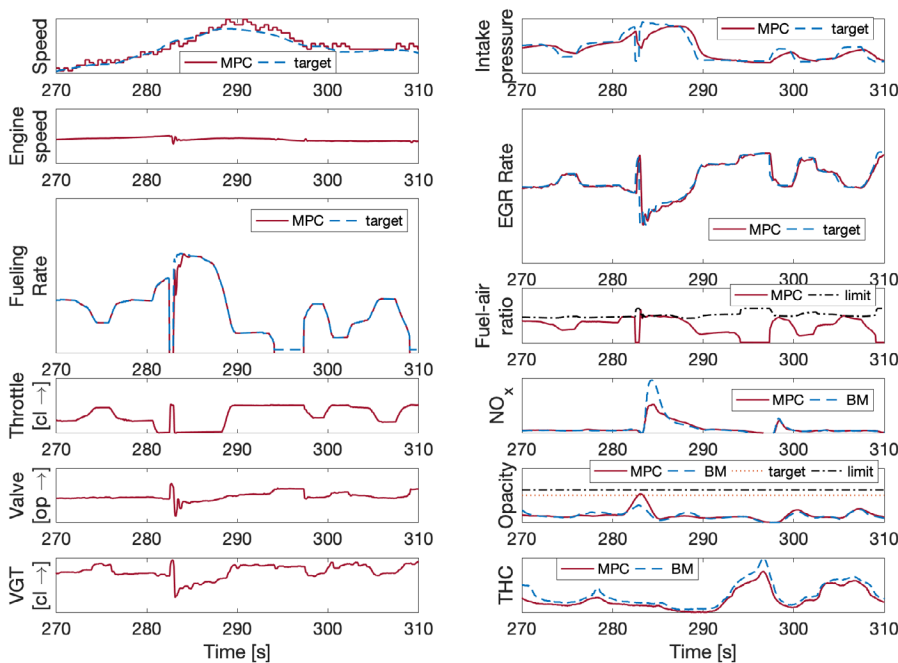
FIGURE 20 A comparison between the MPC and a benchmark (BM) strategy running in closed loop with the engine during the WLTC. The MPC controller is able to reduce NO x emissions compared with the benchmark strategy without causing visible smoke or increasing hydrocarbon output. All signals are generated by the MPC controller unless otherwise noted. The y-axes scales have been removed to preserve data confidentiality [Colour figure can be viewed at wileyonlinelibrary.com ]
