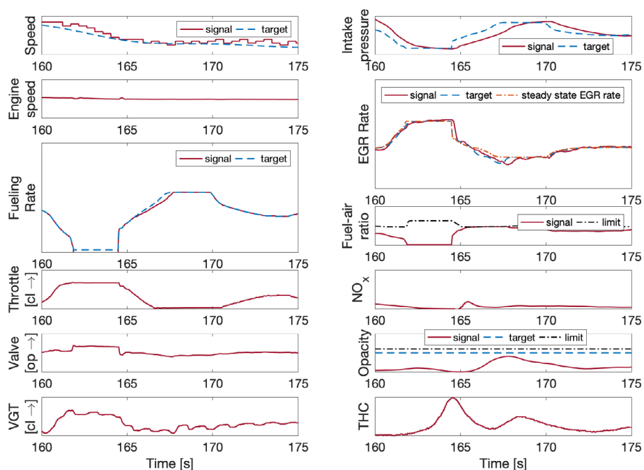
FIGURE 17 A close-up of a high speed portion of the WLTC with the MPC controller in closed loop with the engine. The supervisory layer prevents visible smoke by coordinating the fuel input and the EGR rate. It causes the EGR rate target to undershoot the steady-state optimum, this command is tracked by the NMPC controller, and limits the fueling rate to satisfy the fuel-air ratio constraint and prevent visible smoke. The y-axes scales have been removed to preserve data confidentiality [Colour figure can be viewed at wileyonlinelibrary.com ]
