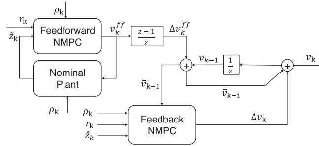
FIGURE 9 A diagram of the feedforward + feedback NMPC architecture. In the square boxes z stands for the discrete shift operator, that is, u_k + 1 = z u_k , and r = [\chi^{trg} \ p_{im}^{trg}]^T . The feedforward NMPC controller is placed in loop with a nominal plant model which is used to generate fictitious measurements, denoted by \bar{z} , as opposed to the real measurements, \hat{z} , which are provided to the feedback controller. Note that \Delta v is computed by the feedback module, v^{ff} is computed by the feedforward module, v is applied to the engine, and \bar{v} is supplied to the feedback module through (19d)
