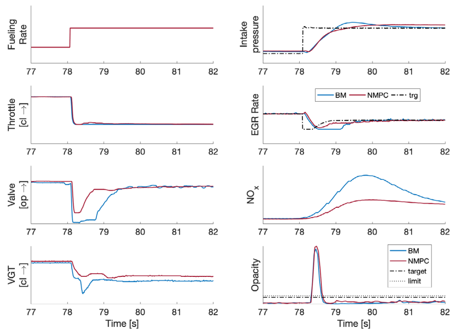
FIGURE 11 A comparison between the benchmark (BM) and NMPC controllers during a fuel step-up maneuver at a constant engine speed. The NMPC controller is able to more closely track the EGR rate target leading to reduced \text{NO}_x emissions. The supervisory controller is disabled so opacity limits are not enforced. The y-axes scales have been removed to preserve data confidentiality [Colour figure can be viewed at wileyonlinelibrary.com ]
