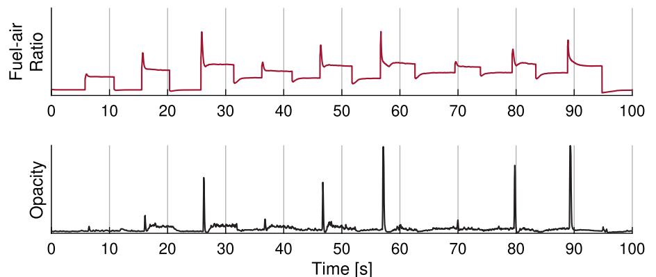
FIGURE 8 The normalized fuel-air ratio is strongly correlated with smoke [Colour figure can be viewed at wileyonlinelibrary.com ]
