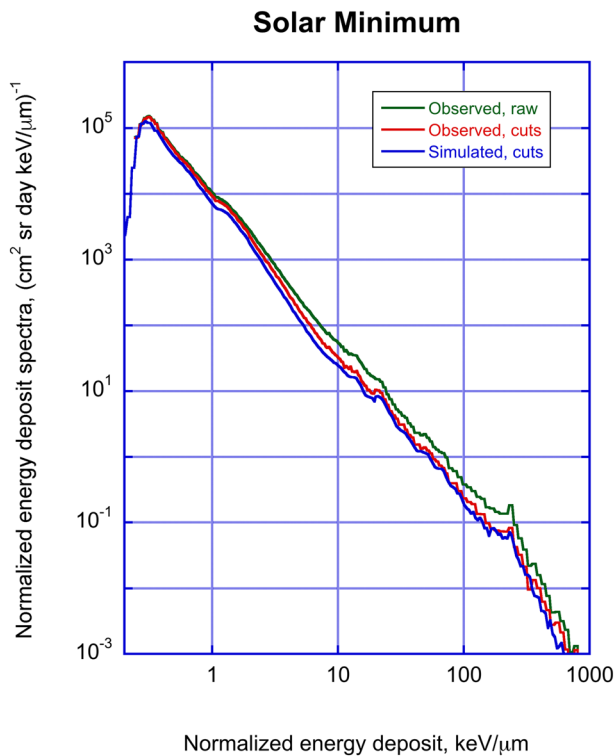
Figure 5. Effect of cuts on observed D5/6 LET spectrum compared with simulations.
