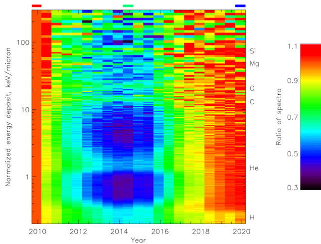
Figure 6. Ratios between measured LET spectra for each 6-month period and the spectrum from the first period (shown as solid red or unity on the linear colorscale). Energy deposit values where peaks due to relativistic ions are less modulated are labeled with the applicable element's symbol at right. Red, green, and blue bars above the plot identify time periods plotted in Figure 7.
