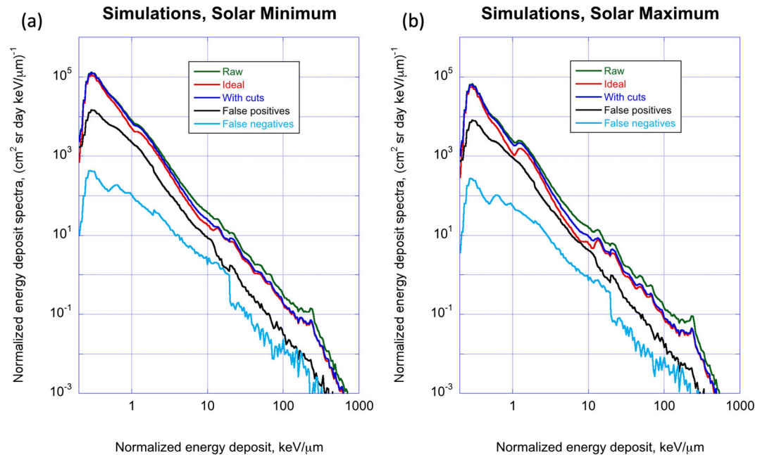
Figure 4. Effectiveness of cuts on simulated D5/6 LET spectra. (a) Solar minimum GCR spectra. (b) Solar maximum GCR spectra.
