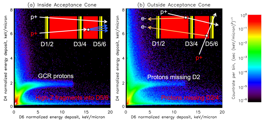
Figure 1. Crossplots of simulated energy deposits in D4 and D6 detectors from GCR protons. Inset diagrams show examples of particle trajectories contributing to each plot. (a) Foreground signal from protons arriving within the acceptance cone, showing events contributing to the LET spectrum in D5 and D6. (b) Background signal from protons arriving from all other directions except those blocked by the Moon, showing events that may be confused with the foreground signal.
