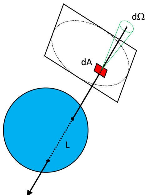
Figure A1. Geometry for calculation of dose rate from LET spectrum.
