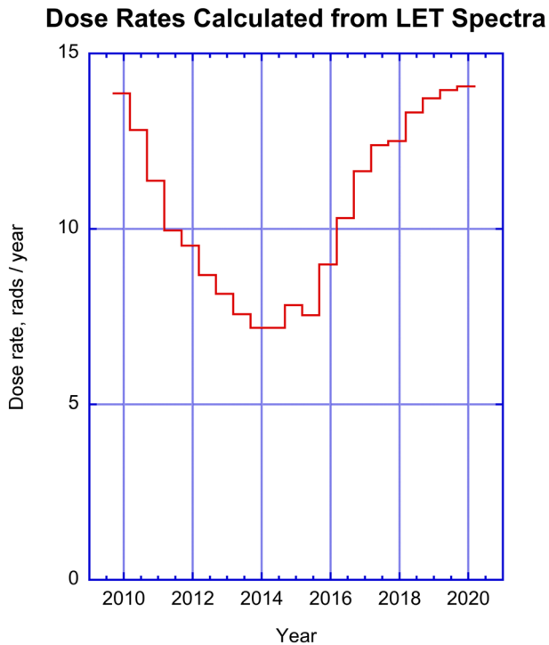
Figure A2. Dose rates calculated from the LET spectra for the 6-month periods in Figure 6, integrated over all look directions in an unobstructed 4\pi sr.
