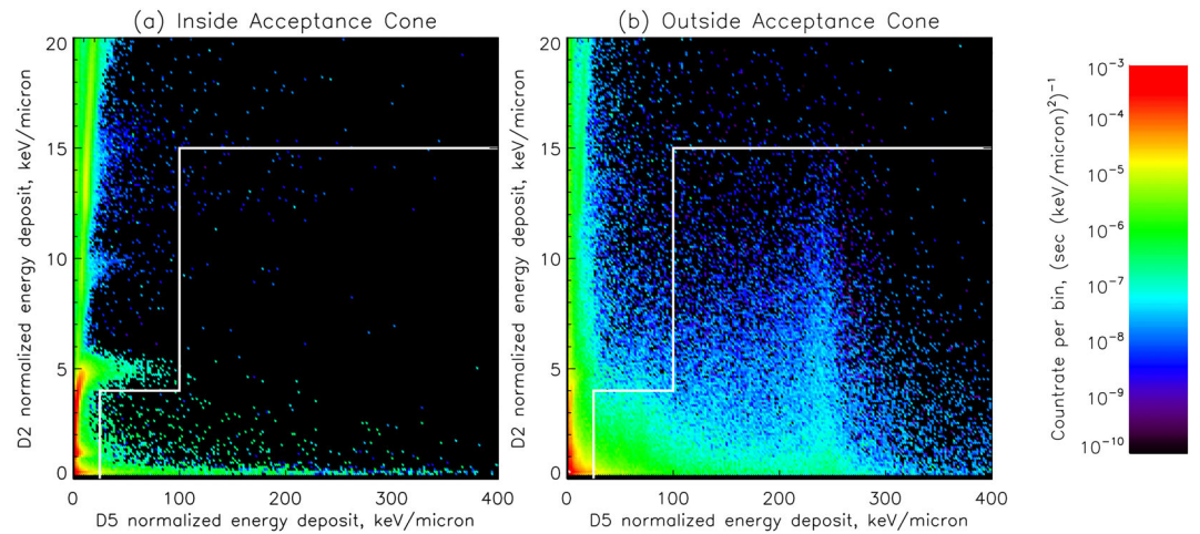
Figure 3. Crossplots of simulated energy deposits in D2 and D5 detectors for all GCR ions up to nickel having energy deposits in D4 above 1.7 \text{ keV}/\mu\text{m} , with white lines indicating the cut described in the main text. (a) Events due to particles arriving within the acceptance cone, showing few events below the cut line. (b) Events due to particles arriving from outside the acceptance cone, showing many events below the line that can be rejected by the cut.
