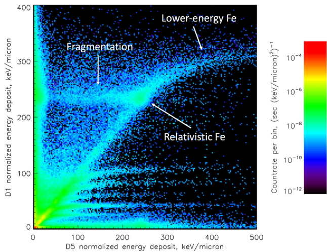
Figure 2. Crossplot of simulated energy deposits in D1 and D5 detectors from all GCR ions up to nickel, both inside and outside the acceptance cone. Portions of the event population due to GCR iron are labeled.
