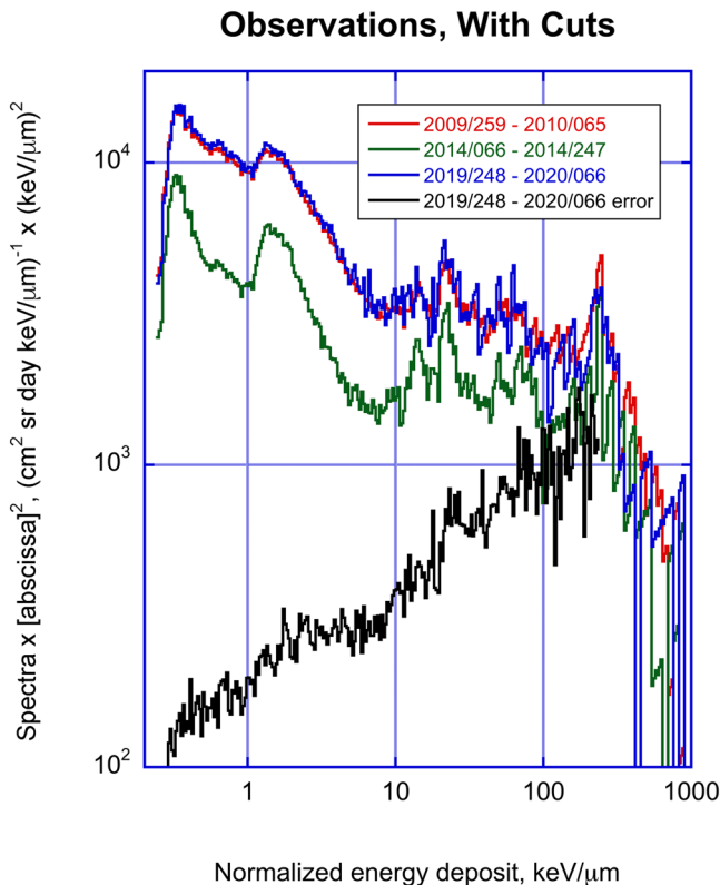
Figure 7. LET spectra at two solar minima and the solar maximum between them, from the periods identified by bars of the same colors as these curves above the plot in Figure 6. Black curve shows the standard deviation of the mean of the daily measurements for the individual LET bins composing the blue curve. All curves are multiplied by the square of the abscissa, to compress the dynamic range.
