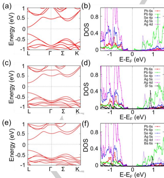
Figure 2. Electronic band structures of Ag-doped PbSe with \Delta E_v \sim 0.21 eV (a); Ag-doped and SrSe-allyed PbSe with \Delta E_v \sim 0.17 eV (c); Ag-doped and BaSe-allyed PbSe with \Delta E_v \sim 0.17 eV (e); and corresponding density of states for Ag-doped PbSe (b); Ag-doped and SrSe-allyed PbSe (d); Ag-doped and BaSe-allyed PbSe (f), where the corresponding states with only one atom in each species are displayed to clearly show their contribution.
