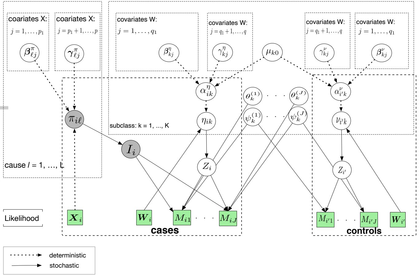
FIGURE 1 The directed acyclic graph (DAG) representing the structure of the model likelihood. The quantities in squares are either data or hyperparameters; the unknown quantities are shown in the circles. The arrows connecting variables indicate that the parent parameterizes the distribution of the child node (solid lines) or completely determines the value of the child node (dotted arrows). The rectangular “plates” where the variables are enclosed indicate that a similar graphical structure is repeated over the index; The index in a plate indicate subjects, causes, covariates or subclasses. Figure S6 in the Supplementary Materials presents the complete DAG with prior specification.
