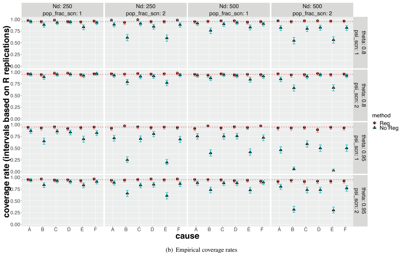
FIGURE 4 The regression analyses produce less biased posterior mean estimates and more valid empirical coverage rates for \pi_\ell^* in Simulation II. Each panel corresponds to one of 16 combinations of true parameter values and sample sizes. Top ) Each boxplot (left: regression; right: no regression) shows the distribution of the percent relative bias of the posterior mean in estimating the overall CSCF \pi_\ell^* for six causes (A - F); “- - -” indicates zero bias. Bottom ) The empirical coverage rates of the 95% CrIs with regression ( \bullet ) or without regression ( \blacktriangle ); “- - -” indicates the nominal 95% level. Since each coverage rate for \pi_\ell^* is computed from R = 200 binary observations of the true \pi_\ell^* being covered or not, a 95% CI is also shown.
