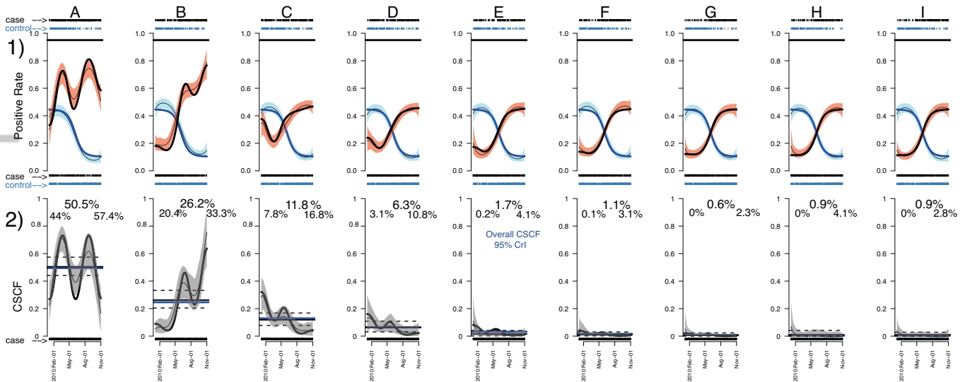
FIGURE 3 Row 2) For each of the 9 single-agent causes (by column) in Simulation I, the posterior mean (thin black curves) and pointwise 95% CrIs (gray) for the CSCF curves \pi_\ell(x) are close to the simulation truths \pi_\ell^0(x) in the stratum of S = 1 (thick black curves). The overall CSCF in the particular stratum is shown along with the 95% CrI on both sides. 25 In row 1), the fitted case (red, \hat{\Pi}(M_\ell = 1 | \mathbf{X}, \mathbf{W}, Y = 1) ) and control (blue, \hat{\Pi}(M_\ell = 1 | \mathbf{W}, Y = 0) ) positive rate curves are shown with the posterior mean curves (thin black curves) along with pointwise 95% credible bands; The rug plots show the positive (top) and negative (bottom) measurements made on cases and controls on the enrollment dates. The solid horizontal lines in row 1 indicate the true TPRs.
