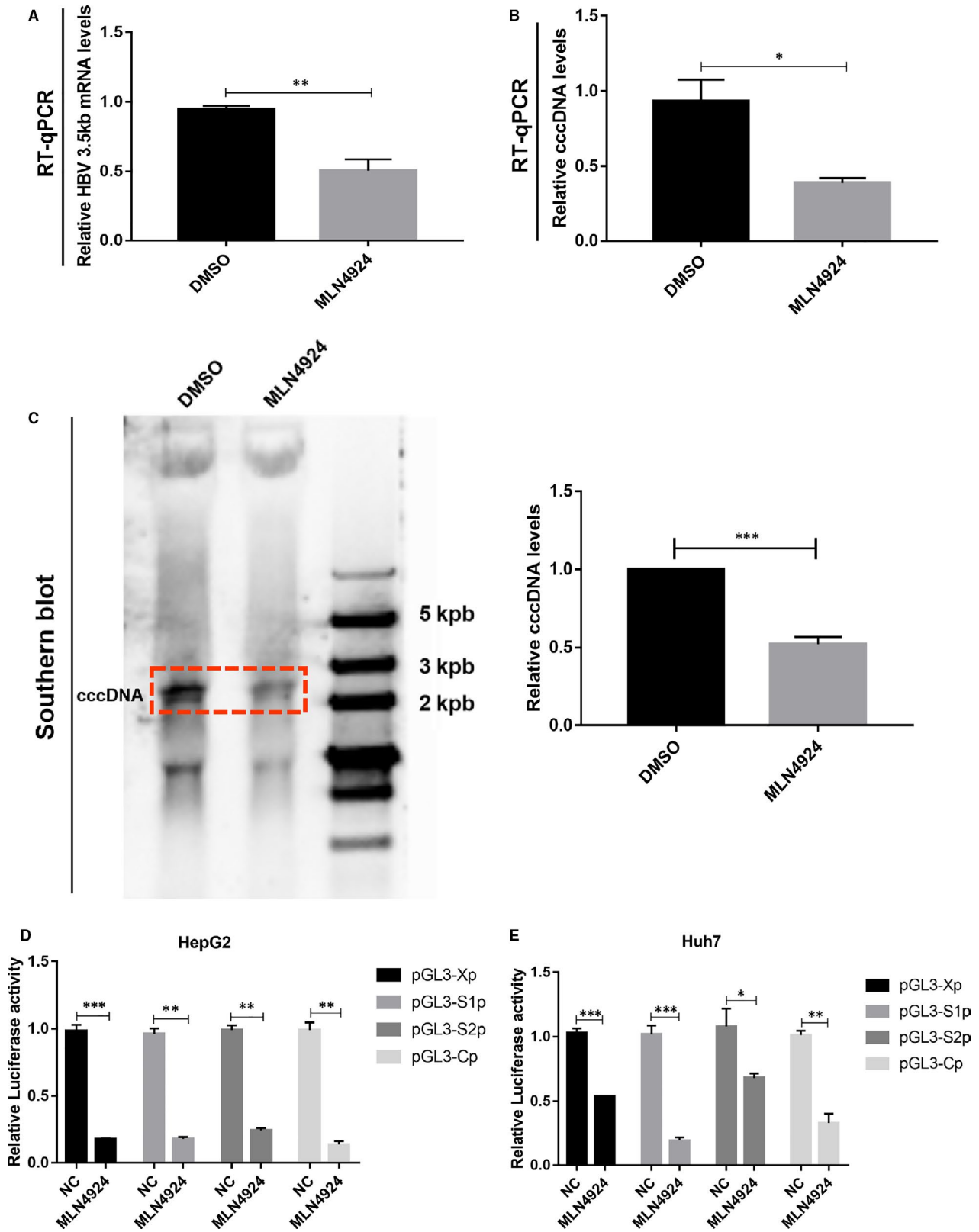
FIGURE 4 MLN4924 inhibits HBV transcription and replication. Total RNA was isolated from HepG2.2.15 cells with or without treatment of MLN4924 and subjected to RT-qPCR analysis to measure the levels of HBV 3.5kb RNA (A). (B-C) Cells were harvested and the levels of cccDNA were detected by RT-qPCR (B) and Southern blot (C). Activities of HBV promoters were assessed by luciferase-based reported assay in HepG2 (D) and Huh7 (E) cells treated with MLN4924 or vehicle control for 48 h, as indicated. Shown are mean \pm SEM from three independent experiments. * P < .05 , ** P < .01 , *** P < .001
