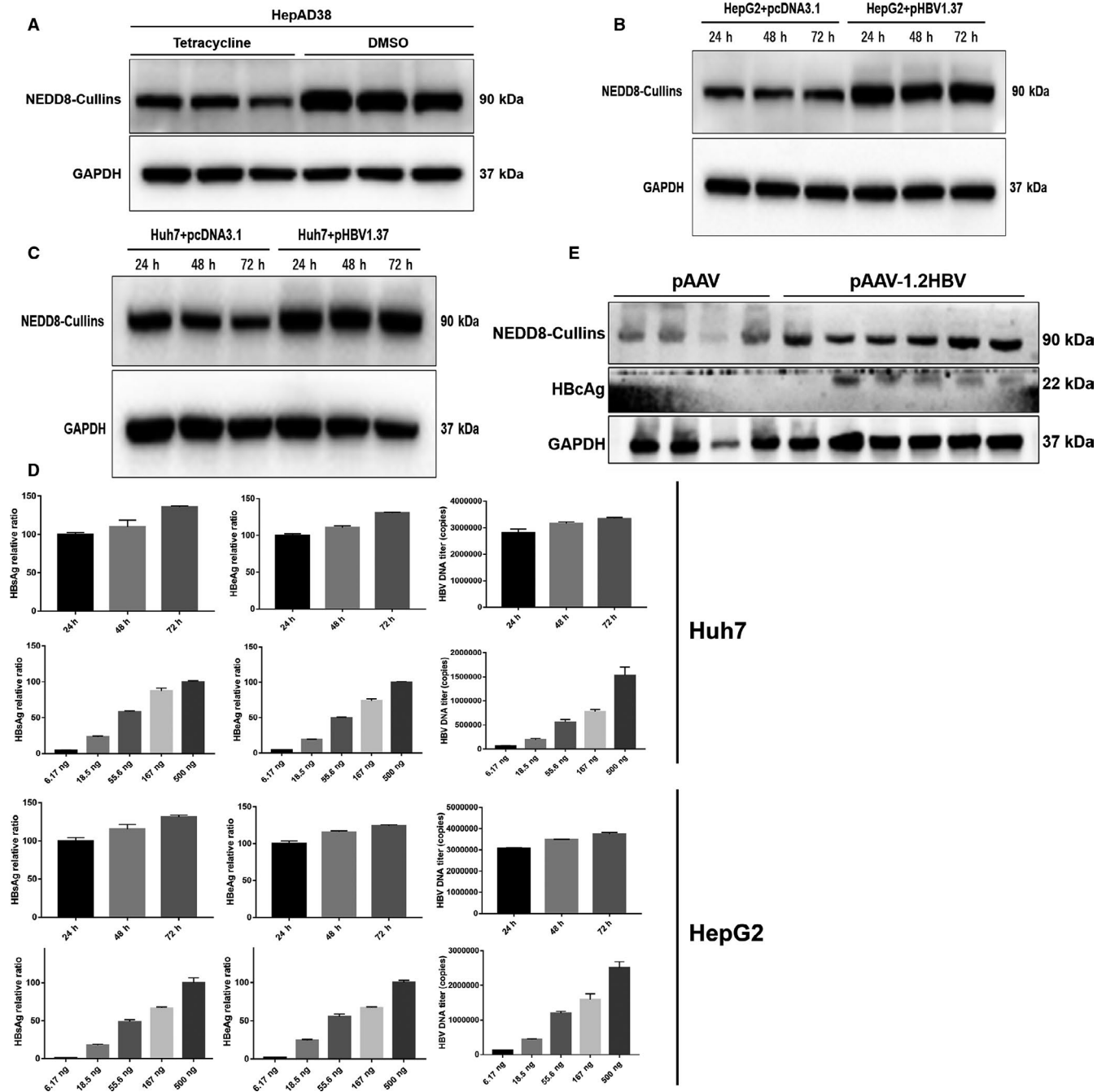
FIGURE 1 HBV activates cullin neddylation in hepatoma cells and liver tissues. (A) HepAD38 cells were cultured in 6 well plates and treated with tetracycline ( 1\mu\text{g}/\mu\text{L} ) or not until confluent. The cell lysates were harvested for Western blotting for NEDD8-Cullins. (B) HepG2 cells and (C) Huh7 cells were transfected with pHBV1.37 plasmids. Cells were collected at indicated times after transfection and subjected to Western blotting using indicated Abs.(D) HepG2 cells and Huh7 cells were transfected with pHBV1.37 plasmids in a time-dependent manner(the concentration of plasmids were 1\mu\text{g}/\text{mL} ) as well as with different dose of plasmids(culture mediums were collected for HBV detection after 48h transfection) separately. Culture mediums were collected for RT-qPCR to determine the HBV DNA levels and subjected to ELISA to measure the levels of HBsAg and HBeAg. (E) 10\mu\text{g} of pAAV-HBV1.2 plasmid, along with empty vector control, were injected into C57BL/6 mice through the tail vein. The mice livers were collected from 4 controls and 6 experimental mice 4 days after injection, followed by Western blotting with indicated antibodies. Cells were then harvested for protein lysate preparation, followed by Western blotting with indicated Abs
