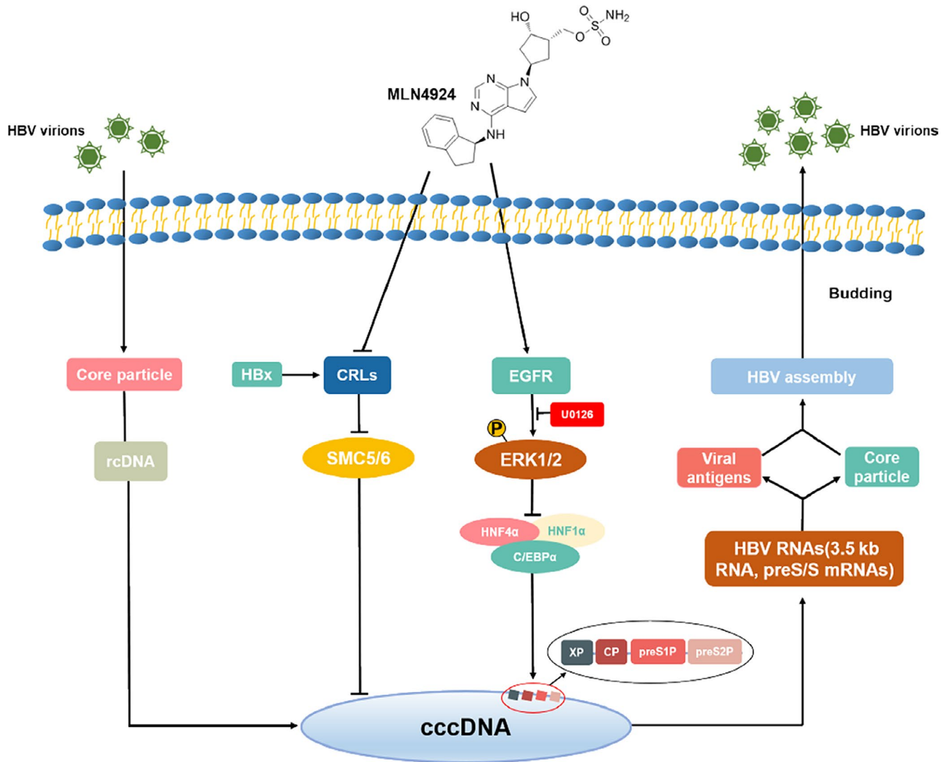
FIGURE 7 MLN4924 anti-HBV model. MLN4924 has two distinct mechanisms of action. On one hand, MLN4924 inactivates CRLs to restore the levels of SMC5/6 to suppress cccDNA, 50 and on the other hand, it activates ERK via EGFR signals to down-regulate the expression of HNF1 \alpha , HNF4 \alpha and C/EBP \alpha . Together, MLN4924 inhibits activities of various HBV promoters, leading to reduction of HBV RNA, HBsAg and rcDNA and finally virion production
