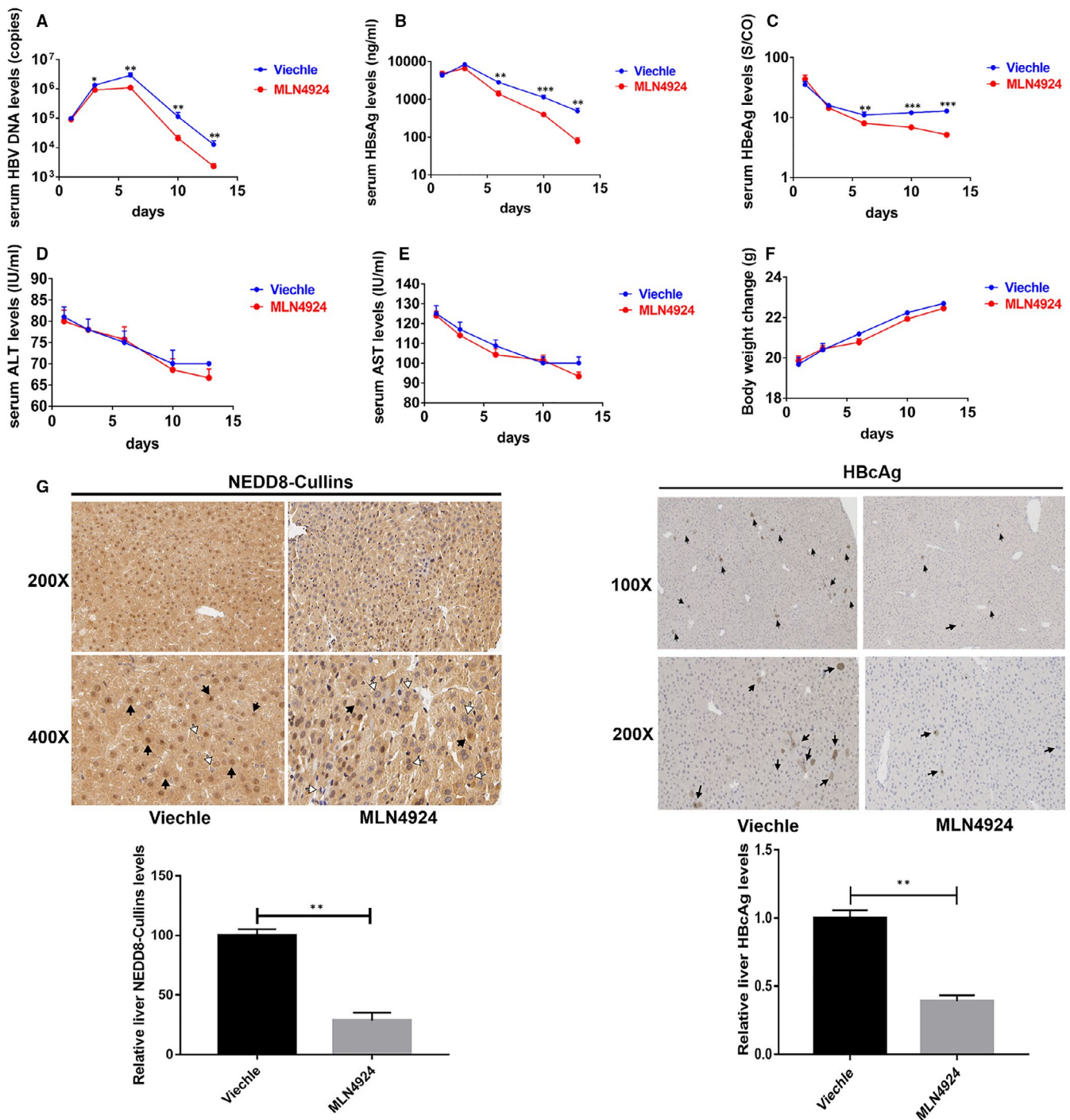
FIGURE 3 MLN4924 exhibits anti-HBV activity in HBV-mice models. C57BL/6 mice were hydrodynamically injected with 10 \mu g of pAAV-HBV1.2 plasmids through tail vein. The mice were subsequently injected i.p. with 60 mg/kg of MLN4924 at day 0, 1, 3, 5, 7 and 9 after injection. Serum samples were collected at indicated time-points. The HBV DNA replicative intermediates in the serum were evaluated by RT-qPCR (A), whereas the levels of HBsAg (B) and HBeAg (C) were measured by ELISA, along with measurement of ALT and AST (D,E), and bodyweight (F). Mice livers were collected at 13-day after virus injection, fixed, sectioned for immunohistochemistry staining with anti-NEDD8 and anti-HBeAg Ab separately. Shown are representative areas (Positive cells were indicated with solid arrows) (G). * P < .05 , ** P < .01 , *** P < .001
