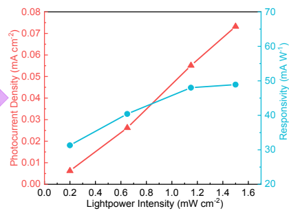
Linear light intensity measurement
