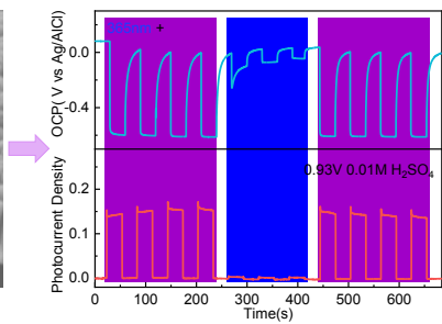
Solar-blind photodetection properties
