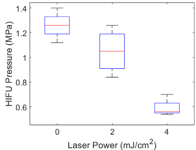
FIG. 3. Ultrasound pressure threshold for effective thrombolysis at 0, 2, and 4 \text{mJ}/\text{cm}^2 of laser fluence after 60 s of treatment ( n = 4 ) [Color figure can be viewed at wileyonlinelibrary.com ]
