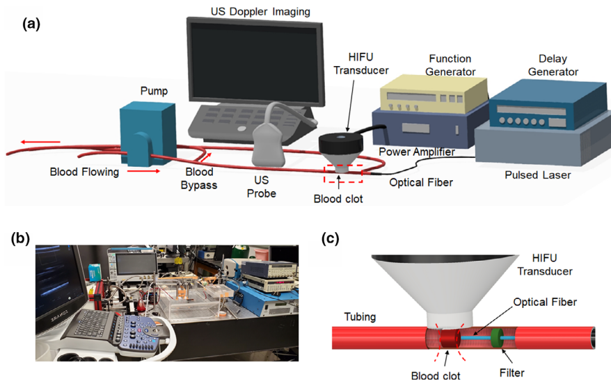
FIG. 1. (a) Schematic of the experimental setup for endovascular laser thrombolysis enhanced by high-intensity focused ultrasound. (b) Photograph of the experimental setup. (c) Schematic showing the treatment area with laser and ultrasound [red dashed box in Fig 1(a)] [Color figure can be viewed at wileyonlinelibrary.com ]
