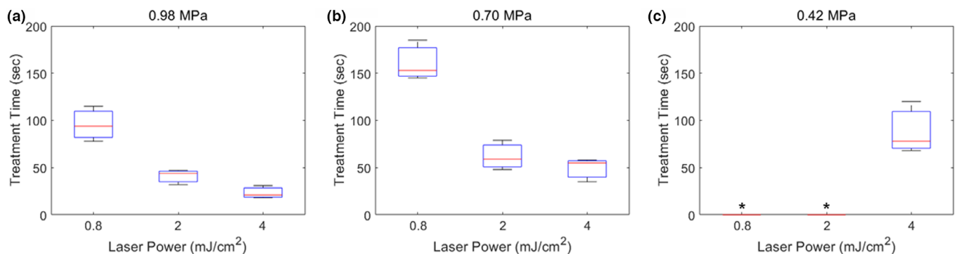
FIG. 5. The period of time needed for effective thrombolysis treatment with different laser fluences (0.8, 2, and 4 \text{ mJ/cm}^2 ) and ultrasound pressures (0.42, 0.70, and 0.98 MPa). (*: no effect of thrombolysis, n = 4 ) [Color figure can be viewed at wileyonlinelibrary.com ]
