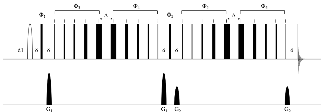
Fig. 5. Depiction of the modified water suppression pulse sequence, PEW5shapepr. The unfilled shape at the beginning of the sequence represents a soft pulse that has been modified from the original sequence. The filled rectangles represent hard pulses. G represents gradient pulses. \Phi represents the following phase cycles: \Phi_1 = x, -x ; \Phi_2 = y ; \Phi_3 = x, x, y, y, -x, -x, -y, -y ; \Phi_4 = -x, -x, -y, -y, x, x, y, y ; \Phi_5 = x, x, x, x, x, x, x, x, y, y, y, y, y, y, y, y, -x, -x, -x, -x, -x, -x, -x, -x, -y, -y, -y, -y, -y, -y, -y, -y ; \Phi_6 = -x, -x, -x, -x, -x, -x, -x, -x, -y, -y, -y, -y, -y, -y, -y, -y, x, x, x, x, x, x, x, x, y, y, y, y, y, y, y, y . Time delays are represented by \delta and \Delta . Full pulse sequence and values are detailed in the supplemental information.
