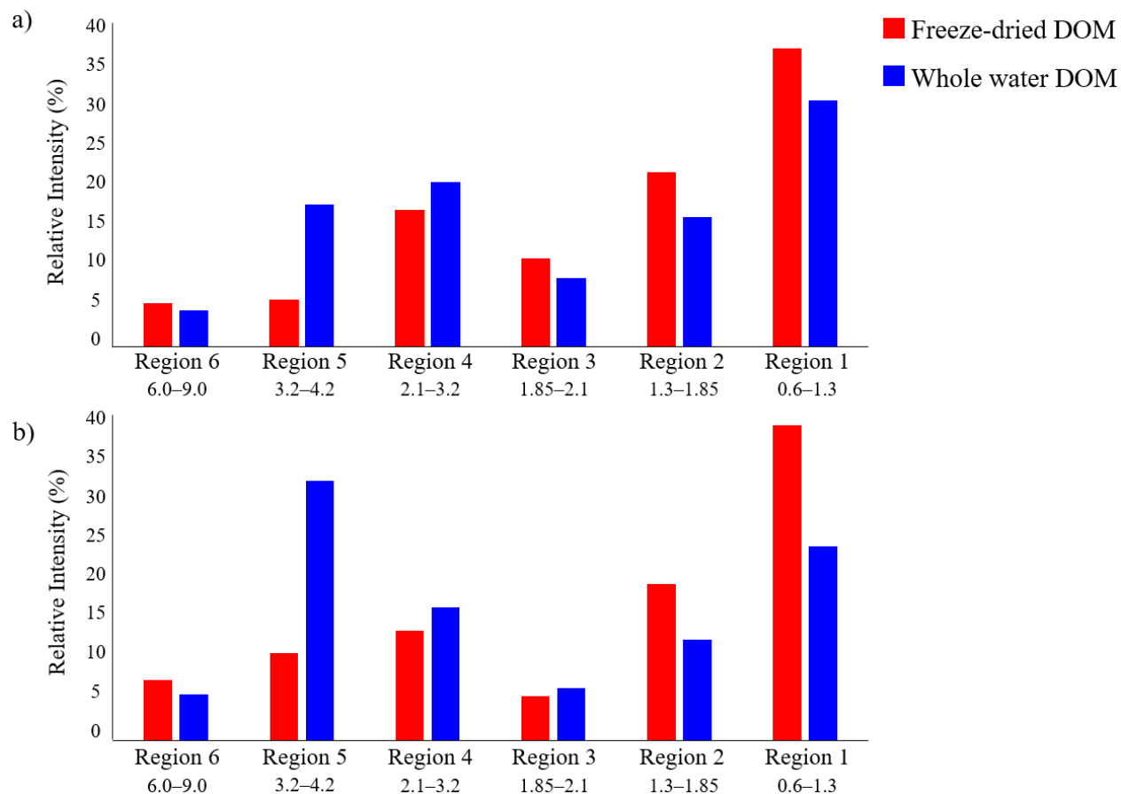
Fig. 3. Comparison of peak area integrations over the six spectral regions of the ^1\text{H} NMR spectra shown in Figure 1 of a) the concentrated 10:1 freeze-dried DOM and corresponding whole water collected from Quebrada Kathia; and b) the non-concentrated freeze-dried DOM and
