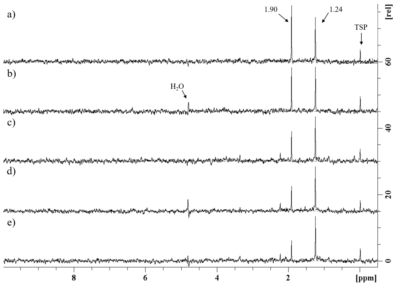
49 Fig. S5. Standard additions of stream water DOM, collected from Quebrada Kathia, analyzed as 50 whole water by 1 H NMR with water suppression. Spectra shown were analyzed following the 51 same instrumental parameters, except the number of scans (ns=600), described in the methods 52 section of the main manuscript. Spectra are as follows: a) stream water DOM + 4 μM calcium 53 acetate; b) stream water DOM + 3 μM calcium acetate; c) stream water DOM + 1 μM calcium 54 acetate; d) stream water DOM + 0.5 μM calcium acetate; and e) stream water DOM.
