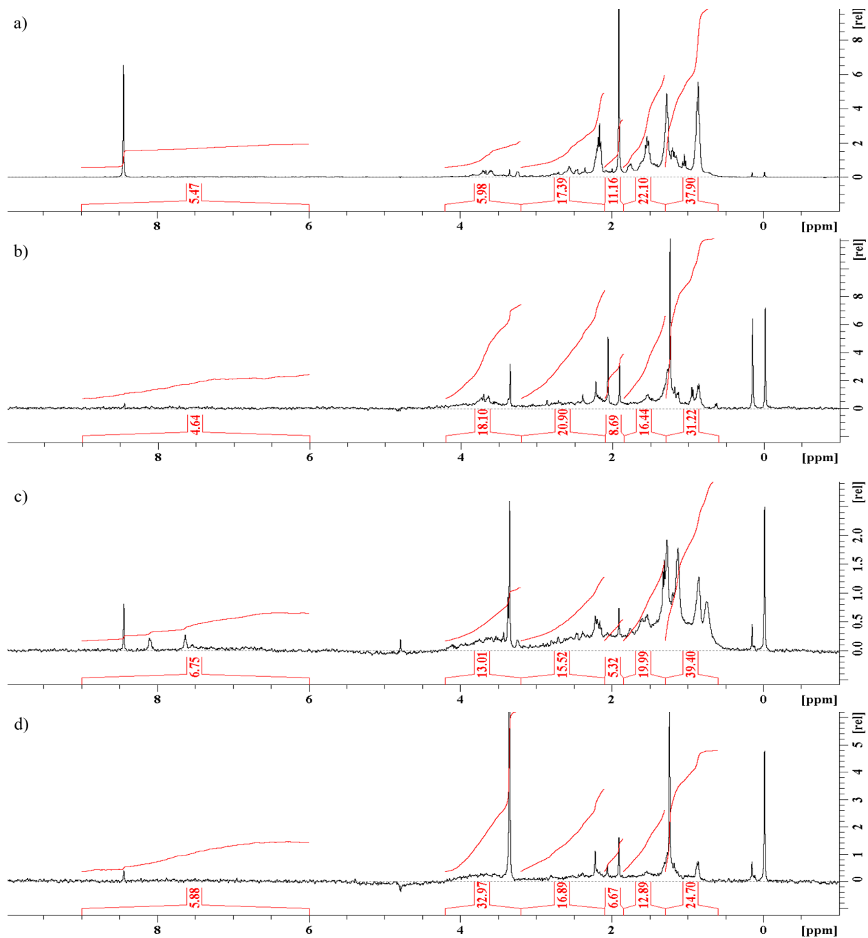
Fig. S8. Integral curves of the 1 H NMR spectra for a) Quebrada Kathia freeze-dried DOM concentrated 10:1; b) Quebrada Kathia whole water DOM; c) Quebrada Rosa freeze-dried DOM not concentrated; d) Quebrada Rosa whole water DOM.
