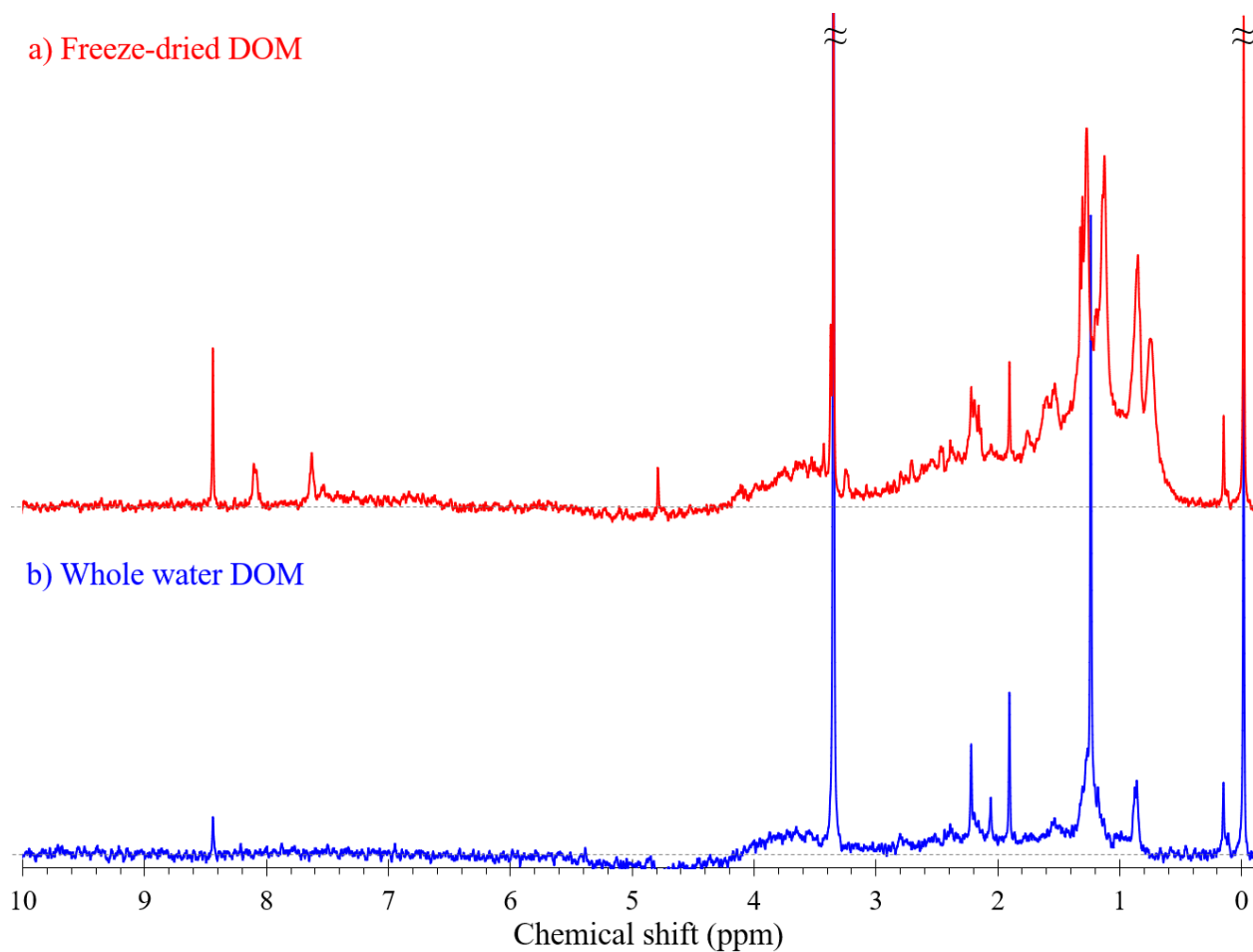
27 Fig. S2. Full ^1\text{H} NMR spectra (0–10 ppm) of stream water DOM, collected from Quebrada Rosa, 28 analyzed after subjected to different methods of preparation: a) freeze-dried but not concentrated 29 in \text{H}_2\text{O}:\text{D}_2\text{O} , and b) whole water without pre-concentration in \text{H}_2\text{O}:\text{D}_2\text{O} . Both spectra have been 30 analyzed under identical instrument parameters and normalized to TSP, the internal standard just 31 before 0.0 ppm
