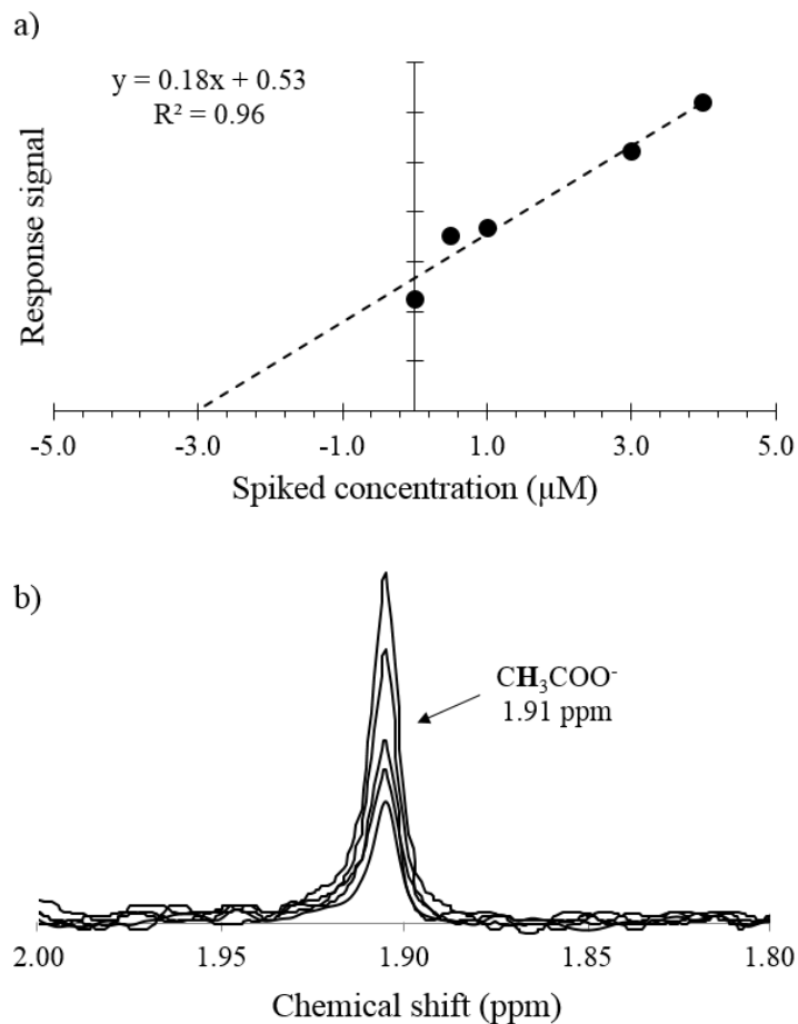
Fig. 2. Standard additions of stream water DOM, collected from Quebrada Kathia, analyzed as whole water by ^1\text{H} NMR with water suppression. a) Standard curve of the calcium acetate additions. The black data points are the standard additions and the dotted line is the extrapolated linear regression used to determine the acetate concentration in the stream water. b) ^1\text{H} NMR spectra of the acetate peak in the stream water overlaid with each addition of calcium acetate, full spectra for the matrix spikes are shown in the supplemental information Figure S5. Due to limited volume of stream water available for analysis, the stream water used for standard
