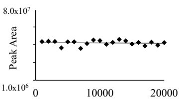
Region 1: 0.6 – 1.3 ppm
