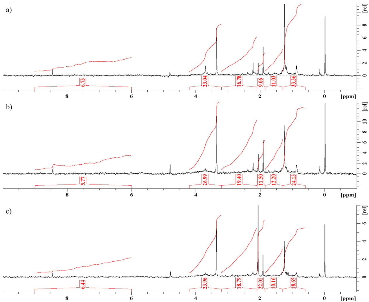
80 Fig. S9. Integral curves of the ^1\text{H} NMR spectra for a) Rio Tempisquito whole water DOM; b) 81 Rio Tempisquito Sur whole water DOM; c) confluence of the Rio Tempisquito and Rio 82 Tempisquito Sur whole water DOM.
