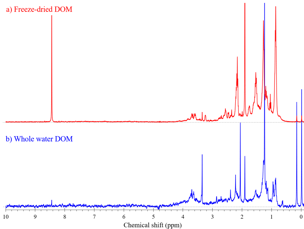
20 Fig. S1. Full ^1\text{H} NMR spectra (0–10 ppm) of stream water DOM, collected from Quebrada Kathia, 21 analyzed after subject to different methods of preparation: a) 10:1 concentration by freeze-drying 22 in \text{H}_2\text{O}:\text{D}_2\text{O} , and b) whole water without pre-concentration in \text{H}_2\text{O}:\text{D}_2\text{O} . Both spectra have been 23 analyzed under identical instrument parameters and normalized to TSP, the internal standard just 24 before 0.0 ppm
