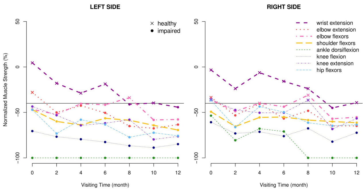
sim_8956_alsex.eps
